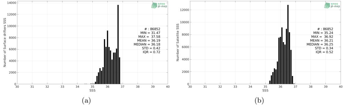
Figure 2: Histograms of SSS from Surface drifters (a) and SMOS SSS L3 v5 - 18 Days (CATDS-CECOS-LOCEAN) (b) considering all match-up pairs per bins of 0.1 over the OTT zone Pi-MEP region and for the full satellite product period.
