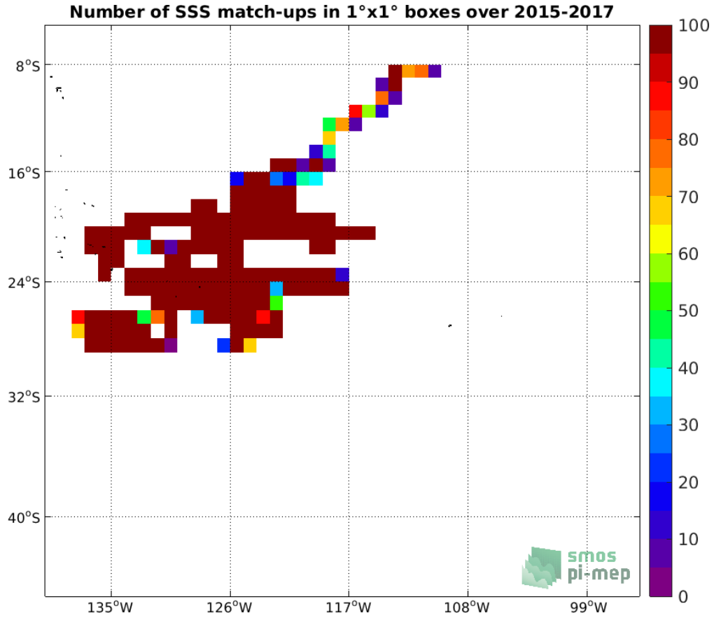
Figure 3: Number of SSS match-ups between Surface drifters SSS and the SMOS SSS L3 v5 - 18 Days (CATDS-CECOS-LOCEAN) SSS product for the OTT zone Pi-MEP region over 1°x1° boxes and for the full satellite product period.
