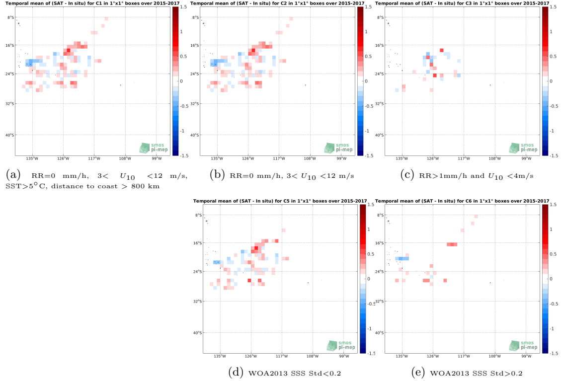
Figure 11: Temporal mean gridded over spatial boxes of size 1^{\circ}\times 1^{\circ} of \Delta\text{SSS} (SMOS SSS L3 v5 - 18 Days (CATDS-CECOS-LOCEAN) - Surface drifters) for 5 different subdatasets corresponding to:RR=0 mm/h, 3 < U_{10} < 12 m/s, \text{SST}>5^{\circ}\text{C} , distance to coast > 800 km (a), RR=0 mm/h, 3 < U_{10} < 12 m/s (b), \text{RR}>1\text{mm/h} and U_{10} < 4\text{m/s} (c), WOA2013 SSS Std <0.2 (d), WOA2013 SSS Std >0.2 (e).
