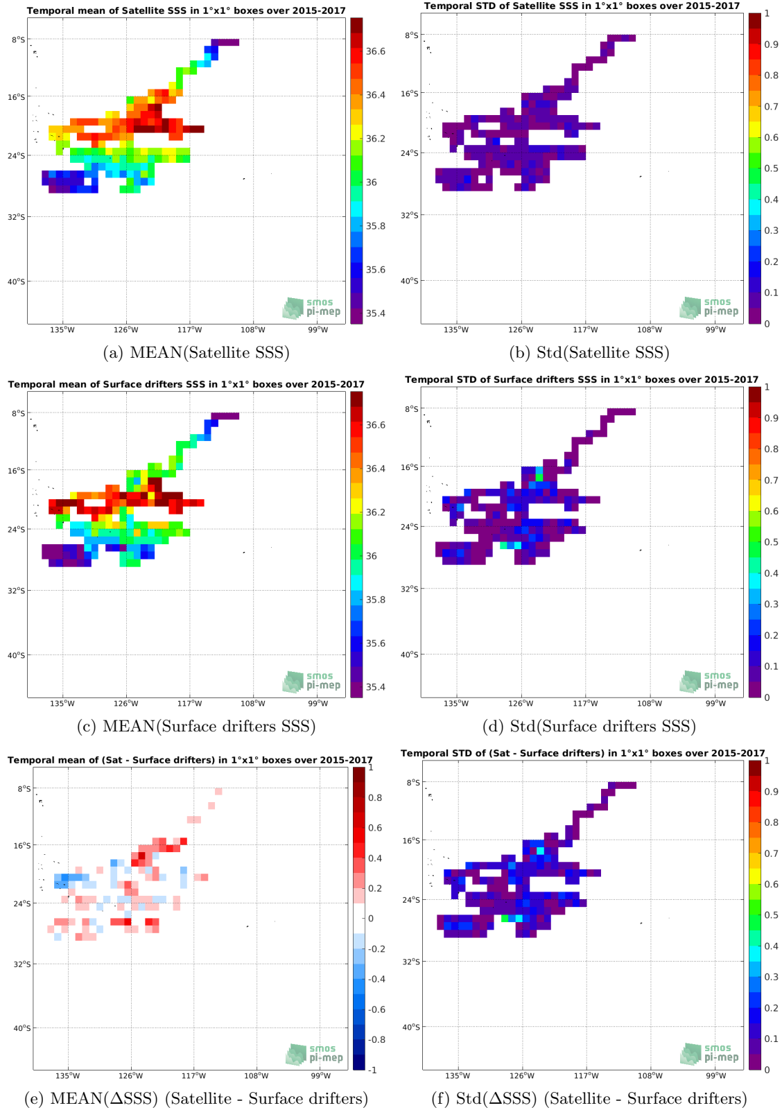
Figure 5: Temporal mean (left) and Std (right) of SSS from SMOS SSS L3 v5 - 18 Days (CATDS-CECOS-LOCEAN) (top), Surface drifters (middle), and of \Delta SSS (Satellite - Surface drifters). Only match-up pairs are used to generate these maps.
