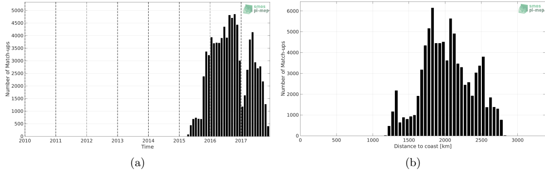
Figure 1: Number of match-ups between Surface drifters and SMOS SSS L3 v5 - 18 Days (CATDS-CECOS-LOCEAN) SSS as a function of time (a) and as function of the distance to coast (b) over the OTT zone Pi-MEP region and for the full satellite product period.
