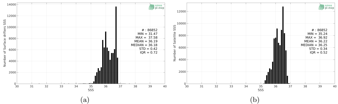
Figure 2: Histograms of SSS from Surface drifters (a) and SMOS SSS L3 v5 - 18 Days (CATDS-CECOS-LOCEAN) (b) considering all match-up pairs per bins of 0.1 over the OTT zone Pi-MEP region and for the full satellite product period.
