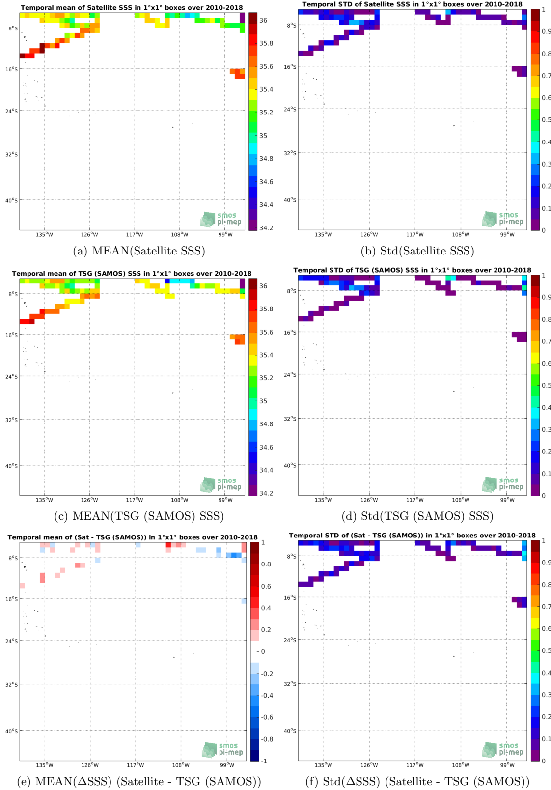
Figure 6: Temporal mean (left) and Std (right) of SSS from SMOS SSS L3 v4 - 9 Days (CATDS-CECOS-LOCEAN) (top), TSG (SAMOS) (middle), and of \Delta SSS (Satellite - TSG (SAMOS)). Only match-up pairs are used to generate these maps.
