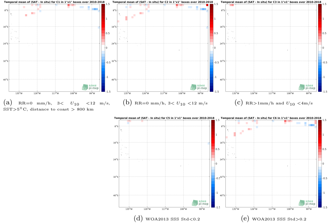
Figure 12: Temporal mean gridded over spatial boxes of size 1^{\circ}\times 1^{\circ} of \Delta\text{SSS} (SMOS SSS L3 v4 - 9 Days (CATDS-CECOS-LOCEAN) - TSG (SAMOS)) for 5 different subdatasets corresponding to: RR=0 mm/h, 3 < U_{10} < 12 m/s, SST >5^{\circ}\text{C} , distance to coast > 800 km (a), RR=0 mm/h, 3 < U_{10} < 12 m/s (b), RR >1 mm/h and U_{10} < 4 m/s (c), WOA2013 SSS Std <0.2 (d), WOA2013 SSS Std >0.2 (e).
