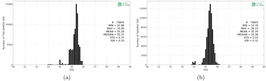
Figure 2: Histograms of SSS from TSG-SAMOS (a) and SMOS-L3-CATDS-CECOS-LOCEAN-V4-9DAYS-25KM (b) considering all match-up pairs per bins of 0.1 over the OTT zone Pi-MEP region and for the full satellite product period.
