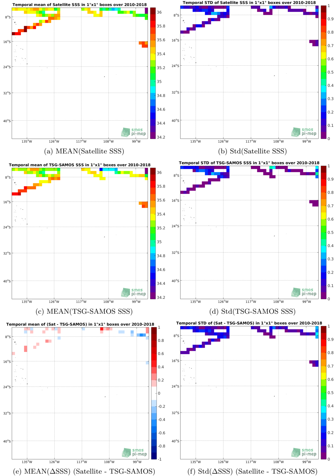
Figure 6: Temporal mean (left) and Std (right) of SSS from SMOS-L3-CATDS-CECOS-LOCEAN-V4-9DAYS-25KM (top), TSG-SAMOS (middle), and of \Delta SSS (Satellite - TSG-SAMOS). Only match-up pairs are used to generate these maps.
