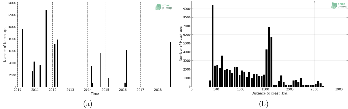
Figure 1: Number of match-ups between TSG-SAMOS and SMOS-L3-CATDS-CECOS-LOCEAN-V4-9DAYS-25KM SSS as a function of time (a) and as function of the distance to coast (b) over the OTT zone Pi-MEP region and for the full satellite product period.
