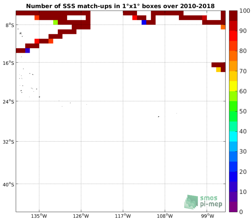
Figure 4: Number of SSS match-ups between TSG-SAMOS SSS and the SMOS-L3-CATDS-CECOS-LOCEAN-V4-9DAYS-25KM SSS product for the OTT zone Pi-MEP region over 1°x1° boxes and for the full satellite product period.
