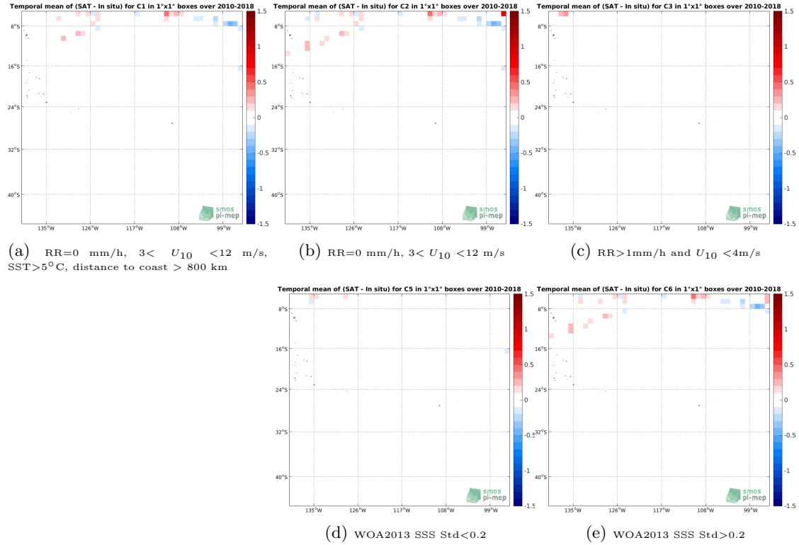
Figure 12: Temporal mean gridded over spatial boxes of size 1^{\circ}\times 1^{\circ} of \Delta\text{SSS} (SMOS-L3-CATDS-CECOS-LOCEAN-V4-9DAYS-25KM - TSG-SAMOS) for 5 different subdatasets corresponding to:RR=0 mm/h, 3 < U_{10} < 12 m/s, SST >5^{\circ}\text{C} , distance to coast > 800 km (a), RR=0 mm/h, 3 < U_{10} < 12 m/s (b), RR >1 mm/h and U_{10} < 4 m/s (c), WOA2013 SSS Std <0.2 (d), WOA2013 SSS Std >0.2 (e).
