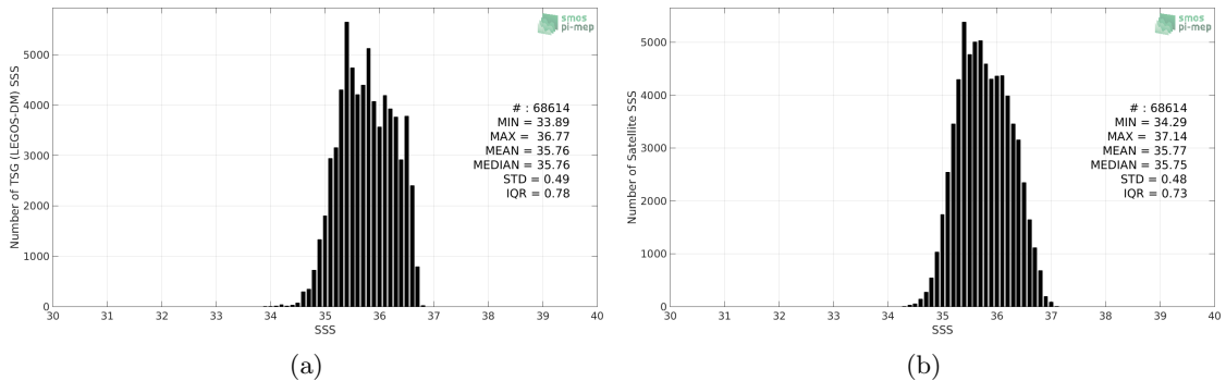
Figure 2: Histograms of SSS from TSG (LEGOS-DM) (a) and SMOS SSS L3 v4 - 9 Days (CATDS-CECOS-LOCEAN) (b) considering all match-up pairs per bins of 0.1 over the OTT zone Pi-MEP region and for the full satellite product period.
