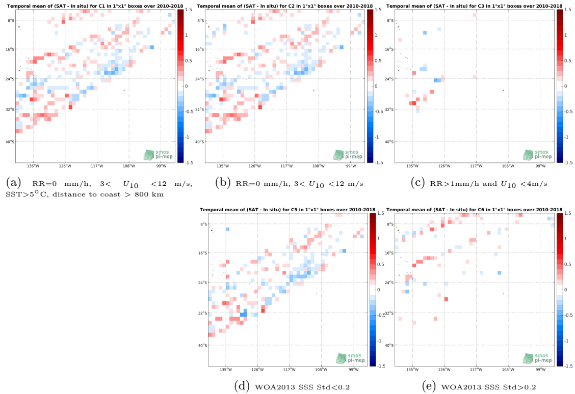
Figure 12: Temporal mean gridded over spatial boxes of size 1^{\circ}\times 1^{\circ} of \Delta\text{SSS} (SMOS-L3-CATDS-CECOS-LOCEAN-V4-9DAYS-25KM - TSG-LEGOS-DM) for 5 different subdatasets corresponding to:RR=0 mm/h, 3 < U_{10} < 12 m/s, SST >5^{\circ}\text{C} , distance to coast > 800 km (a), RR=0 mm/h, 3 < U_{10} < 12 m/s (b), RR >1 mm/h and U_{10} < 4 m/s (c), WOA2013 SSS Std <0.2 (d), WOA2013 SSS Std >0.2 (e).
