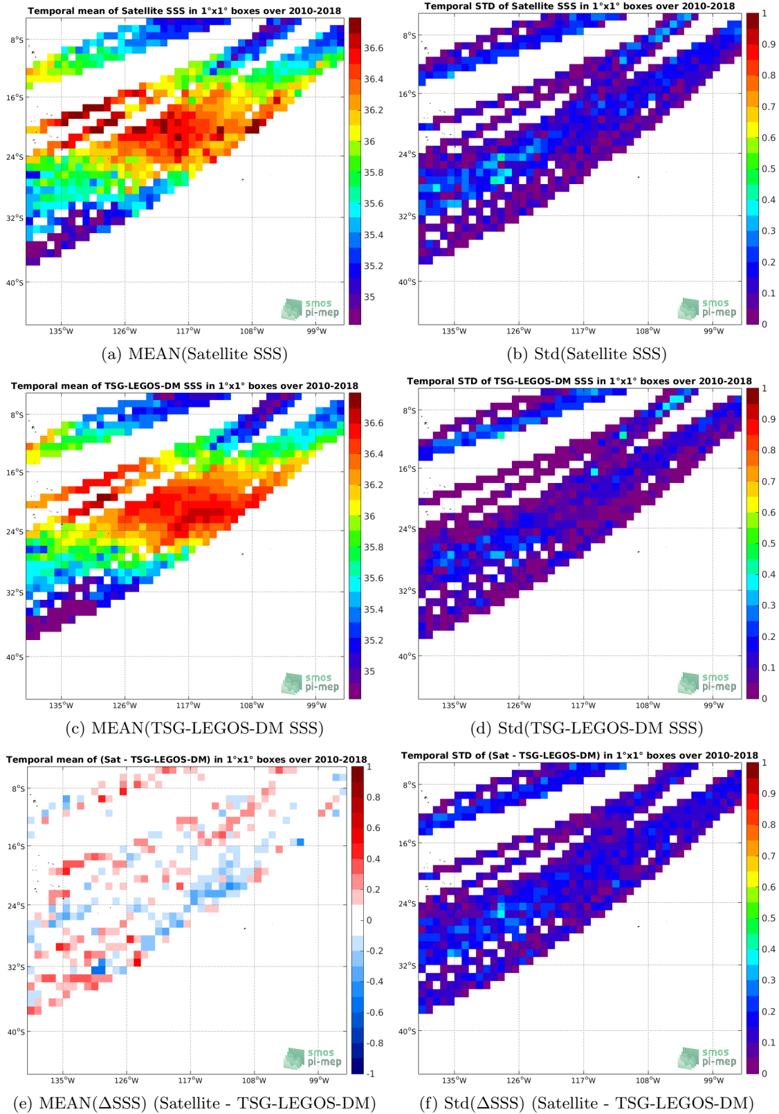
Figure 6: Temporal mean (left) and Std (right) of SSS from SMOS-L3-CATDS-CECOS-LOCEAN-V4-9DAYS-25KM (top), TSG-LEGOS-DM (middle), and of \Delta SSS (Satellite - TSG-LEGOS-DM). Only match-up pairs are used to generate these maps.
