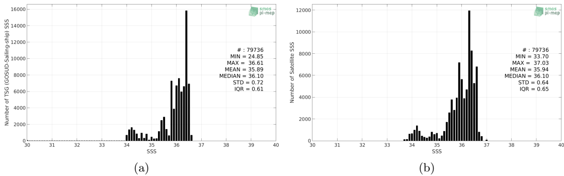
Figure 2: Histograms of SSS from TSG (GOSUD-Sailing-ship) (a) and SMOS SSS L3 v4 - 9 Days (CATDS-CECOS-LOCEAN) (b) considering all match-up pairs per bins of 0.1 over the OTT zone Pi-MEP region and for the full satellite product period.
