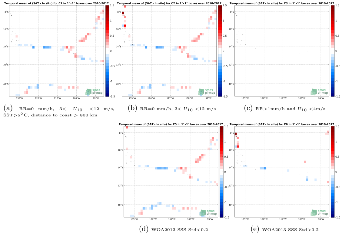
Figure 12: Temporal mean gridded over spatial boxes of size 1^\circ \times 1^\circ of \Delta\text{SSS} (SMOS SSS L3 v4 - 9 Days (CATDS-CECOS-LOCEAN) - TSG (GOSUD-Sailing-ship)) for 5 different subdatasets corresponding to: \text{RR}=0 \text{ mm/h} , 3 < U_{10} < 12 \text{ m/s} , \text{SST} > 5^\circ\text{C} , distance to coast > 800 \text{ km} (a), \text{RR}=0 \text{ mm/h} , 3 < U_{10} < 12 \text{ m/s} (b), \text{RR} > 1\text{mm/h} and U_{10} < 4\text{m/s} (c), WOA2013 SSS Std < 0.2 (d), WOA2013 SSS Std > 0.2 (e).
