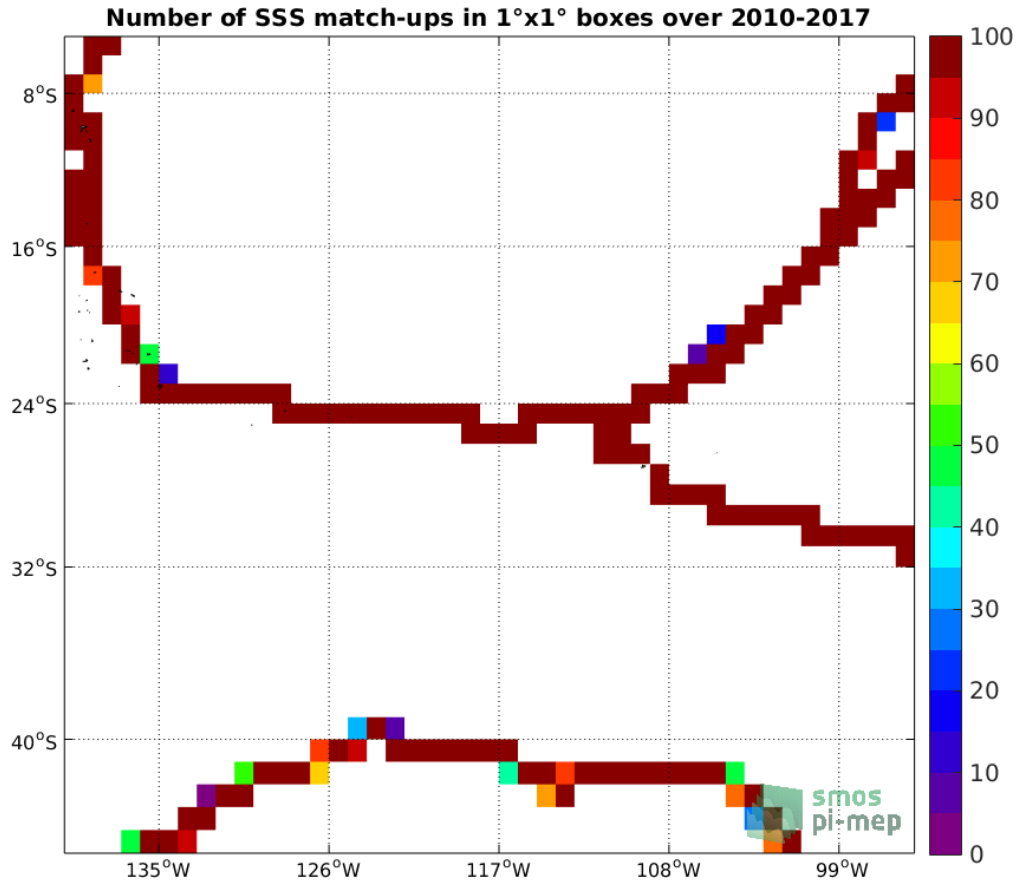
Figure 4: Number of SSS match-ups between TSG (GOSUD-Sailing-ship) SSS and the SMOS SSS L3 v4 - 9 Days (CATDS-CECOS-LOCEAN) SSS product for the OTT zone Pi-MEP region over 1°x1° boxes and for the full satellite product period.
