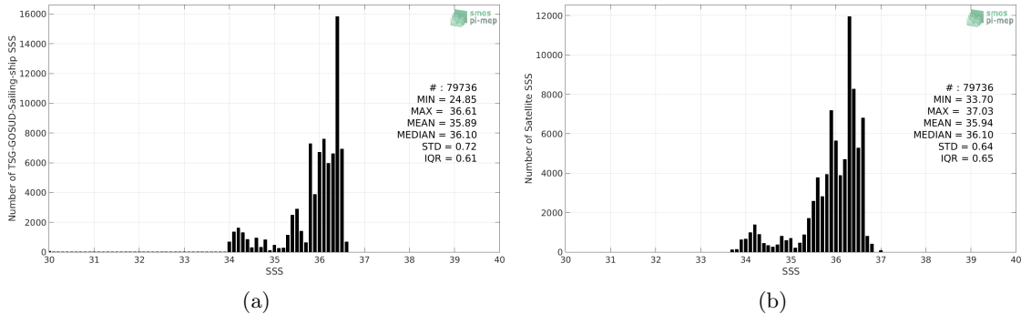
Figure 2: Histograms of SSS from TSG-GOSUD-Sailing-ship (a) and SMOS-L3-CATDS-CECOS-LOCEAN-V4-9DAYS-25KM (b) considering all match-up pairs per bins of 0.1 over the OTT zone Pi-MEP region and for the full satellite product period.
