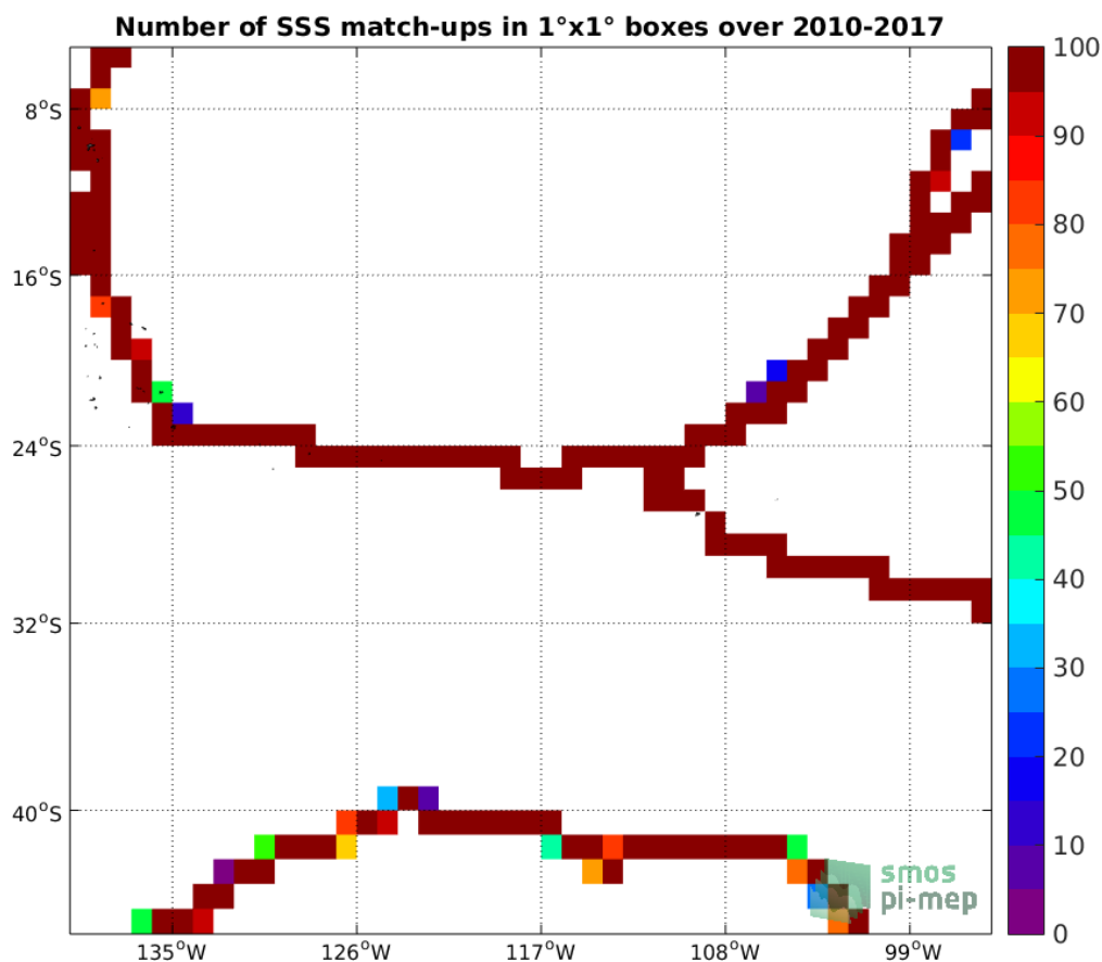
Figure 4: Number of SSS match-ups between TSG-GOSUD-Sailing-ship SSS and the SMOS-L3-CATDS-CECOS-LOCEAN-V4-9DAYS-25KM SSS product for the OTT zone Pi-MEP region over 1°x1° boxes and for the full satellite product period.
