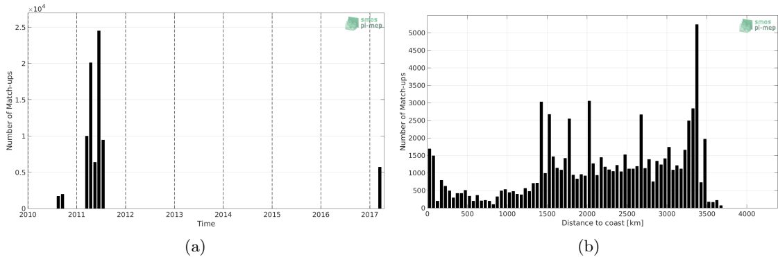
Figure 1: Number of match-ups between TSG-GOSUD-Sailing-ship and SMOS-L3-CATDS-CECOS-LOCEAN-V4-9DAYS-25KM SSS as a function of time (a) and as function of the distance to coast (b) over the OTT zone Pi-MEP region and for the full satellite product period.
