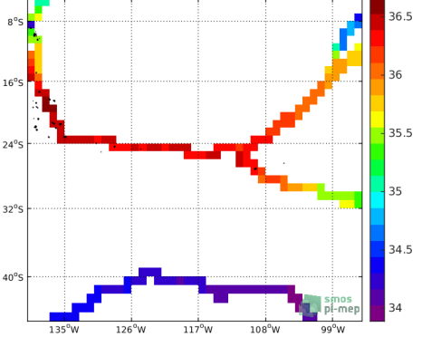
(c) MEAN(TSG-GOSUD-Sailing-ship SSS)
