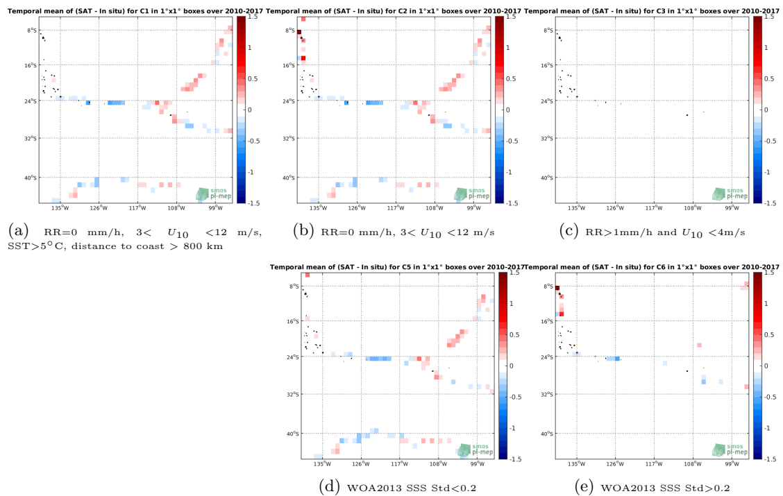
Figure 12: Temporal mean gridded over spatial boxes of size 1^\circ \times 1^\circ of \Delta SSS (SMOS-L3-CATDS-CECOS-LOCEAN-V4-9DAYS-25KM - TSG-GOSUD-Sailing-ship) for 5 different subdatasets corresponding to:RR=0 mm/h, 3 < U_{10} < 12 m/s, SST >5^\circ C, distance to coast > 800 km (a), RR=0 mm/h, 3 < U_{10} < 12 m/s (b), RR >1 mm/h and U_{10} < 4 m/s (c), WOA2013 SSS Std <0.2 (d), WOA2013 SSS Std >0.2 (e).
