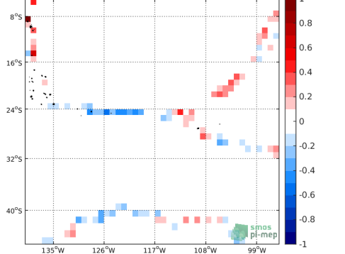
(e) MEAN( \Delta SSS) (Satellite - TSG-GOSUD-Sailing-ship)
