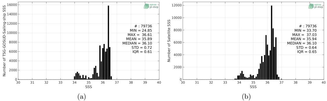
Figure 2: Histograms of SSS from TSG-GOSUD-Sailing-ship (a) and SMOS-L3-CATDS-CECOS-LOCEAN-V4-9DAYS-25KM (b) considering all match-up pairs per bins of 0.1 over the OTT zone Pi-MEP region and for the full satellite product period.
