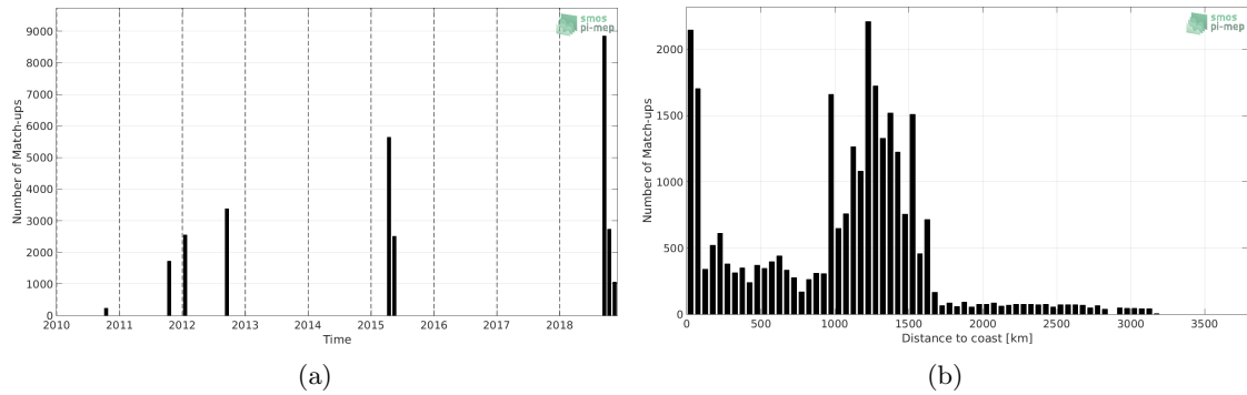
Figure 1: Number of match-ups between TSG (GOSUD-Research-vessel) and SMOS SSS L3 v4 - 9 Days (CATDS-CECOS-LOCEAN) SSS as a function of time (a) and as function of the distance to coast (b) over the OTT zone Pi-MEP region and for the full satellite product period.
