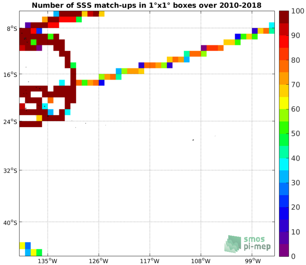
Figure 4: Number of SSS match-ups between TSG (GOSUD-Research-vessel) SSS and the SMOS SSS L3 v4 - 9 Days (CATDS-CECOS-LOCEAN) SSS product for the OTT zone Pi-MEP region over 1°x1° boxes and for the full satellite product period.
