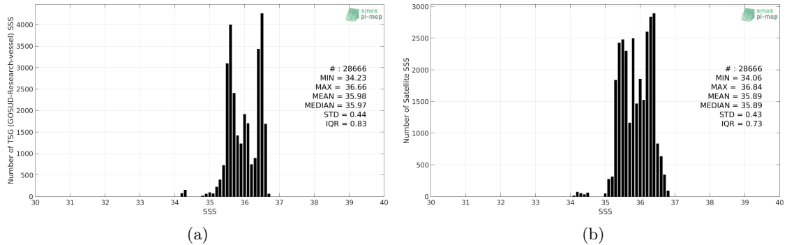
Figure 2: Histograms of SSS from TSG (GOSUD-Research-vessel) (a) and SMOS SSS L3 v4 - 9 Days (CATDS-CECOS-LOCEAN) (b) considering all match-up pairs per bins of 0.1 over the OTT zone Pi-MEP region and for the full satellite product period.
