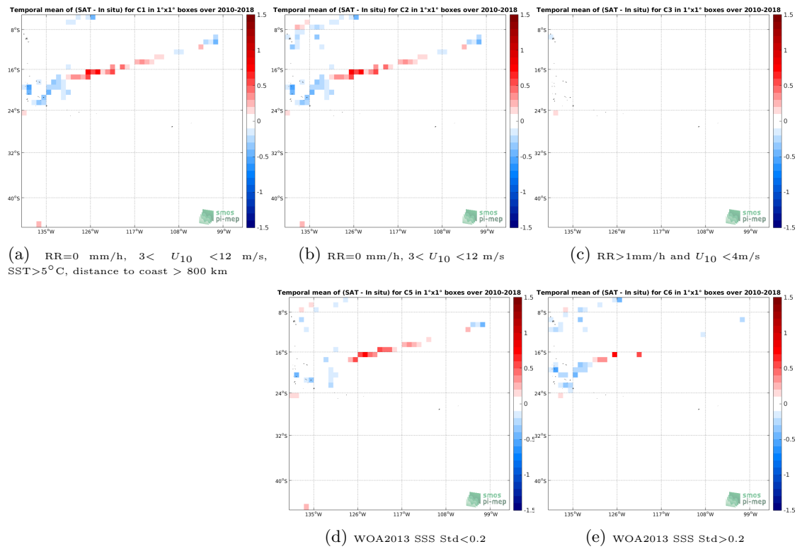
Figure 12: Temporal mean gridded over spatial boxes of size 1^\circ \times 1^\circ of \Delta\text{SSS} (SMOS SSS L3 v4 - 9 Days (CATDS-CECOS-LOCEAN) - TSG (GOSUD-Research-vessel)) for 5 different subdatasets corresponding to: RR=0 mm/h, 3 < U_{10} < 12 \text{ m/s} , SST > 5^\circ\text{C} , distance to coast > 800 \text{ km} (a), RR=0 mm/h, 3 < U_{10} < 12 \text{ m/s} (b), RR > 1 \text{ mm/h} and U_{10} < 4 \text{ m/s} (c), WOA2013 SSS Std < 0.2 (d), WOA2013 SSS Std > 0.2 (e).
