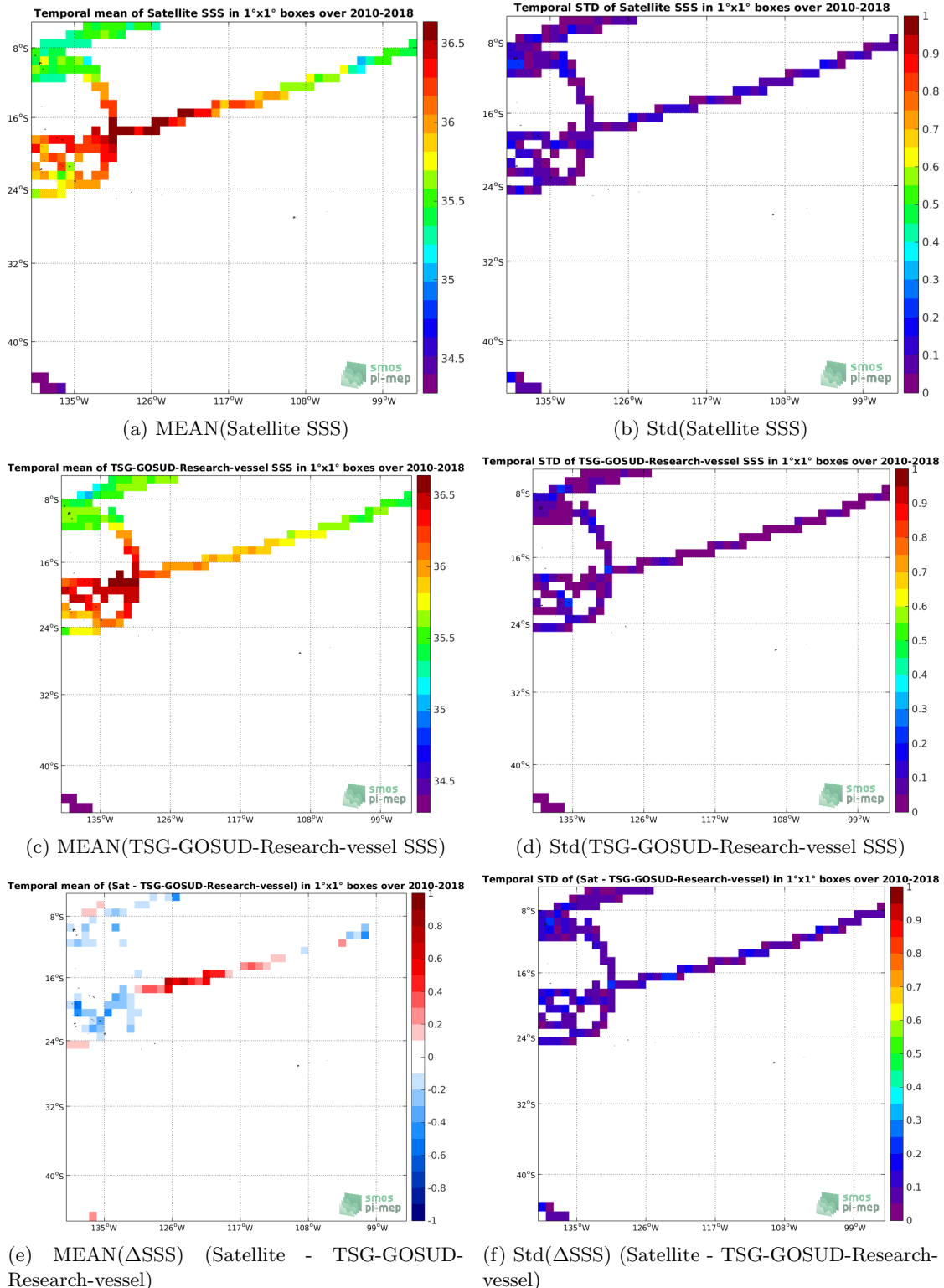
Figure 6: Temporal mean (left) and Std (right) of SSS from SMOS-L3-CATDS-CECOS-LOCEAN-V4-9DAYS-25KM (top), TSG-GOSUD-Research-vessel (middle), and of \Delta SSS (Satellite - TSG-GOSUD-Research-vessel). Only match-up pairs are used to generate these maps.
