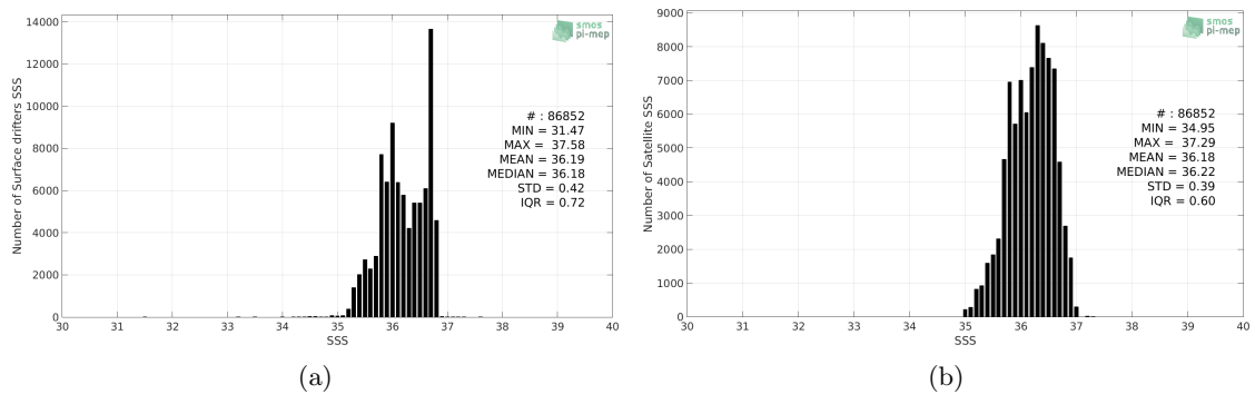
Figure 2: Histograms of SSS from Surface drifters (a) and SMOS SSS L3 v4 - 9 Days (CATDS-CECOS-LOCEAN) (b) considering all match-up pairs per bins of 0.1 over the OTT zone Pi-MEP region and for the full satellite product period.
