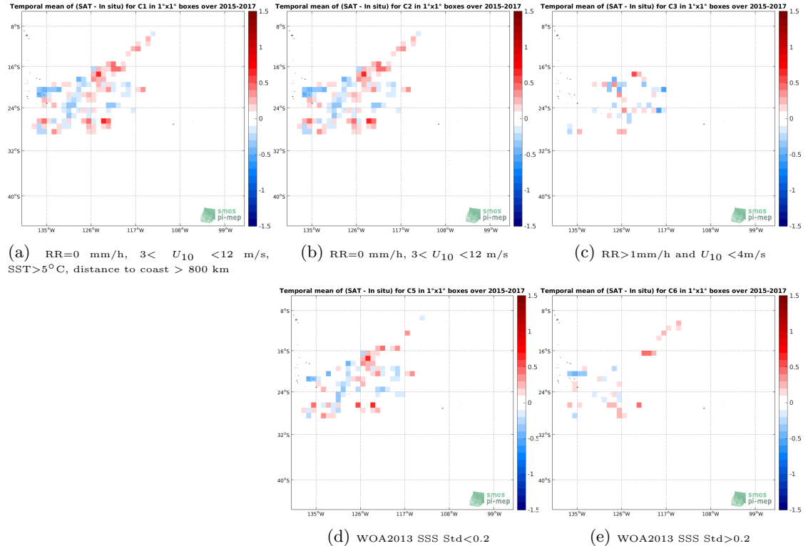
Figure 11: Temporal mean gridded over spatial boxes of size 1^{\circ}\times 1^{\circ} of \Delta\text{SSS} (SMOS SSS L3 v4 - 9 Days (CATDS-CECOS-LOCEAN) - Surface drifters) for 5 different subdatasets corresponding to: \text{RR}=0 mm/h, 3 < U_{10} < 12 m/s, \text{SST} > 5^{\circ}\text{C} , distance to coast > 800 km (a), \text{RR}=0 mm/h, 3 < U_{10} < 12 m/s (b), \text{RR} > 1\text{mm/h} and U_{10} < 4\text{m/s} (c), WOA2013 SSS Std < 0.2 (d), WOA2013 SSS Std > 0.2 (e).
