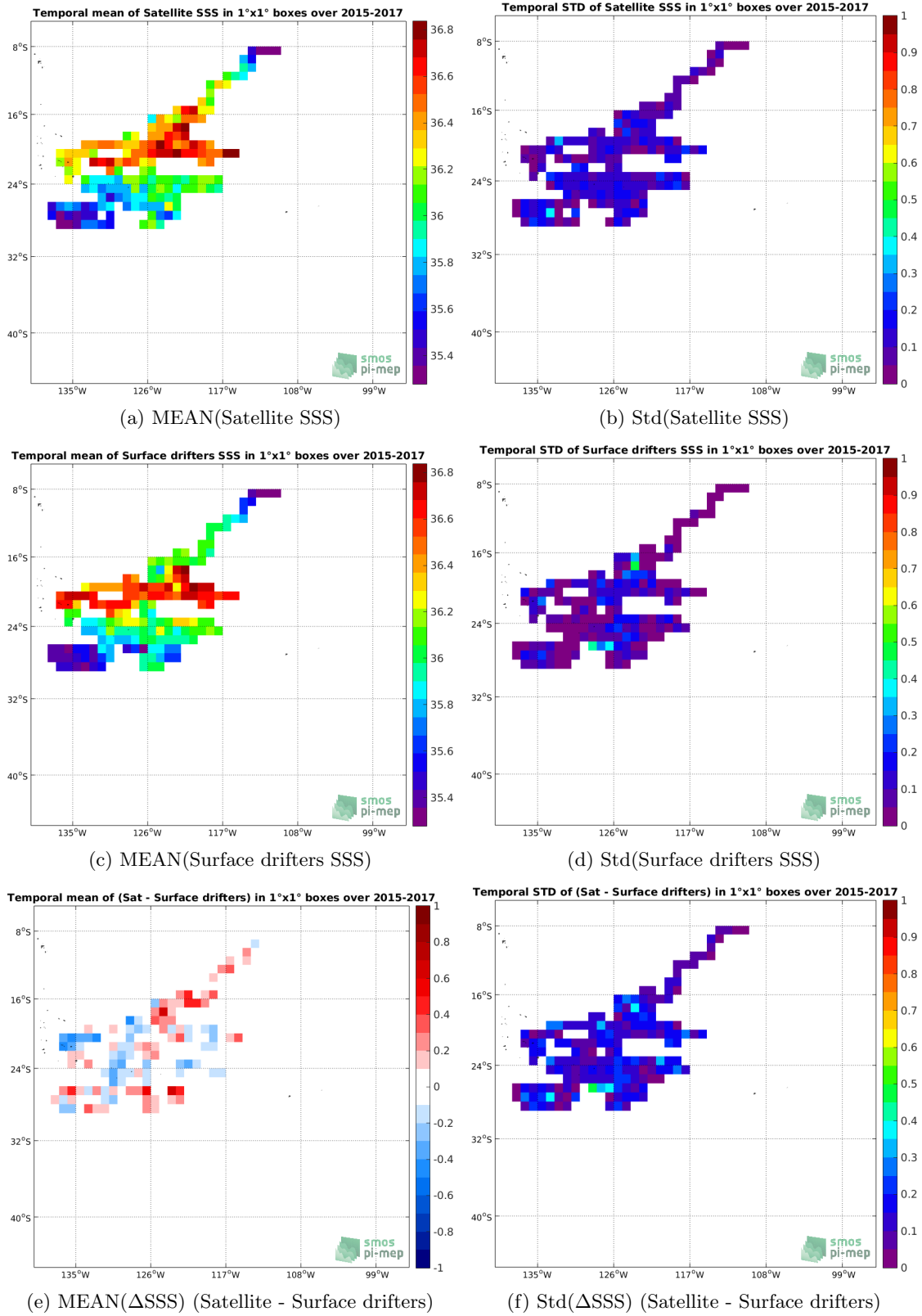
Figure 5: Temporal mean (left) and Std (right) of SSS from SMOS SSS L3 v4 - 9 Days (CATDS-CECOS-LOCEAN) (top), Surface drifters (middle), and of \Delta SSS (Satellite - Surface drifters). Only match-up pairs are used to generate these maps.
