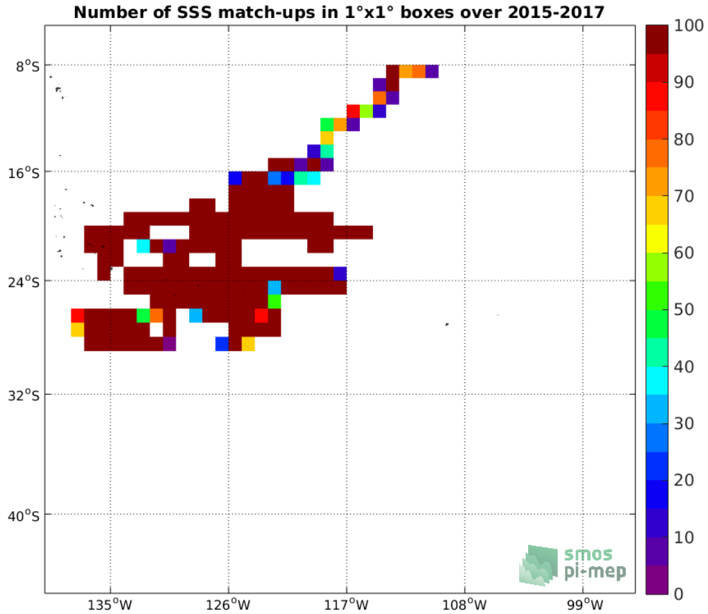
Figure 3: Number of SSS match-ups between Surface drifters SSS and the SMOS SSS L3 v4 - 9 Days (CATDS-CECOS-LOCEAN) SSS product for the OTT zone Pi-MEP region over 1^\circ \times 1^\circ boxes and for the full satellite product period.
