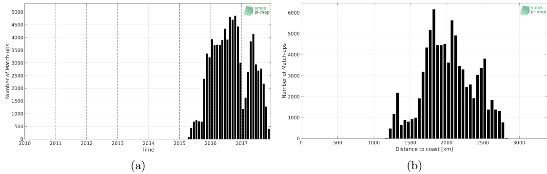
Figure 1: Number of match-ups between Surface drifters and SMOS SSS L3 v4 - 9 Days (CATDS-CECOS-LOCEAN) SSS as a function of time (a) and as function of the distance to coast (b) over the OTT zone Pi-MEP region and for the full satellite product period.
