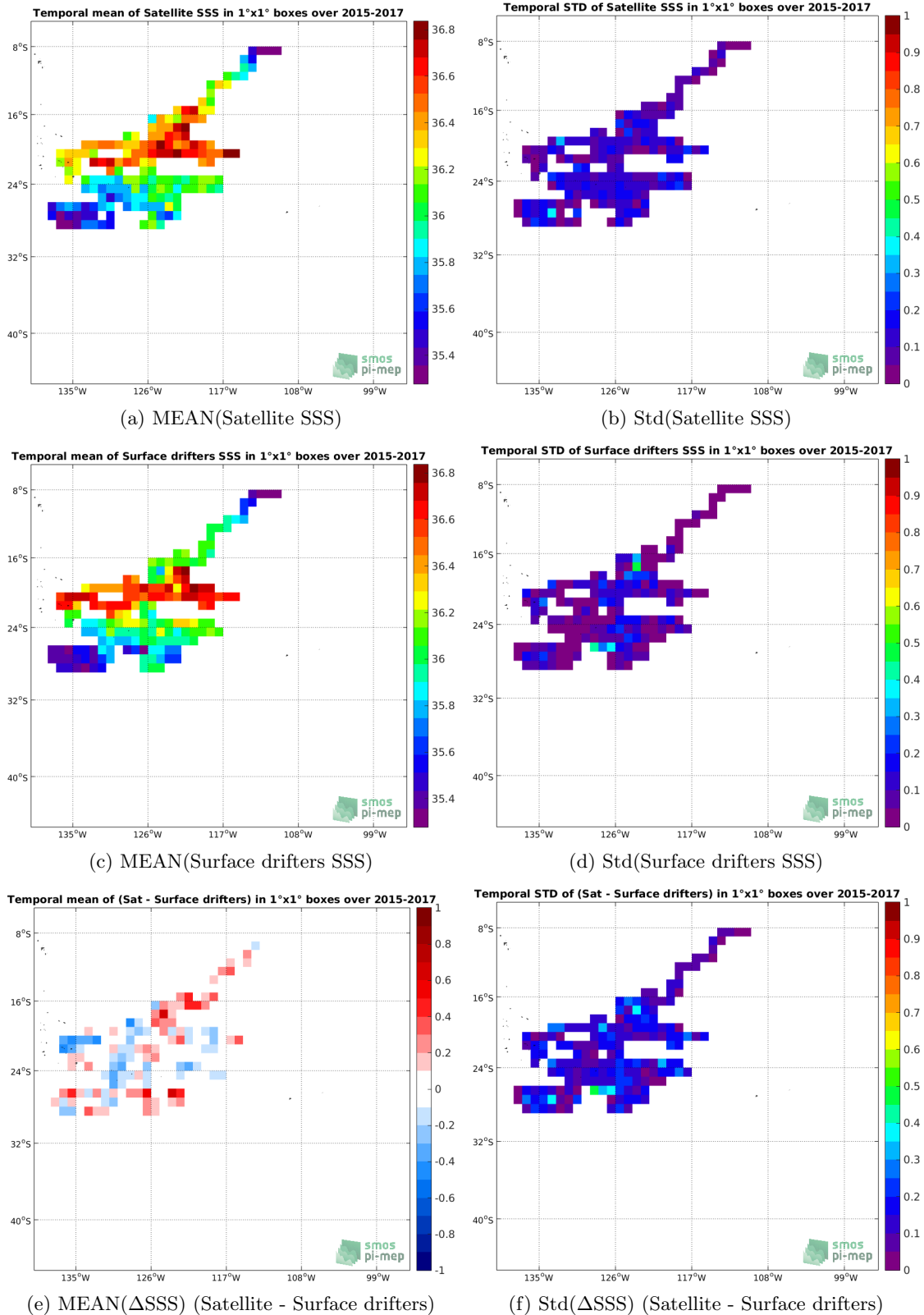
Figure 5: Temporal mean (left) and Std (right) of SSS from SMOS-L3-CATDS-CECOS-LOCEAN-V4-9DAYS-25KM (top), Surface drifters (middle), and of \Delta SSS (Satellite - Surface drifters). Only match-up pairs are used to generate these maps.
