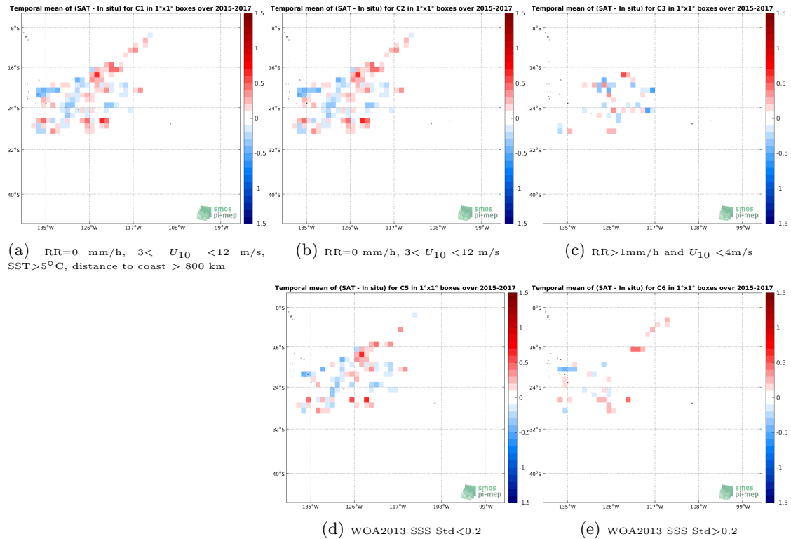
Figure 11: Temporal mean gridded over spatial boxes of size 1^{\circ}\times 1^{\circ} of \Delta\text{SSS} (SMOS-L3-CATDS-CECOS-LOCEAN-V4-9DAYS-25KM - Surface drifters) for 5 different subdatasets corresponding to:RR=0 mm/h, 3 < U_{10} < 12 m/s, SST >5^{\circ}\text{C} , distance to coast > 800 km (a), RR=0 mm/h, 3 < U_{10} < 12 m/s (b), RR >1 mm/h and U_{10} < 4 m/s (c), WOA2013 SSS Std <0.2 (d), WOA2013 SSS Std >0.2 (e).
