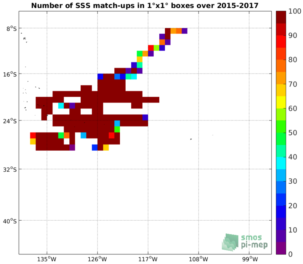
Figure 3: Number of SSS match-ups between Surface drifters SSS and the SMOS-L3-CATDS-CECOS-LOCEAN-V4-9DAYS-25KM SSS product for the OTT zone Pi-MEP region over 1°x1° boxes and for the full satellite product period.
