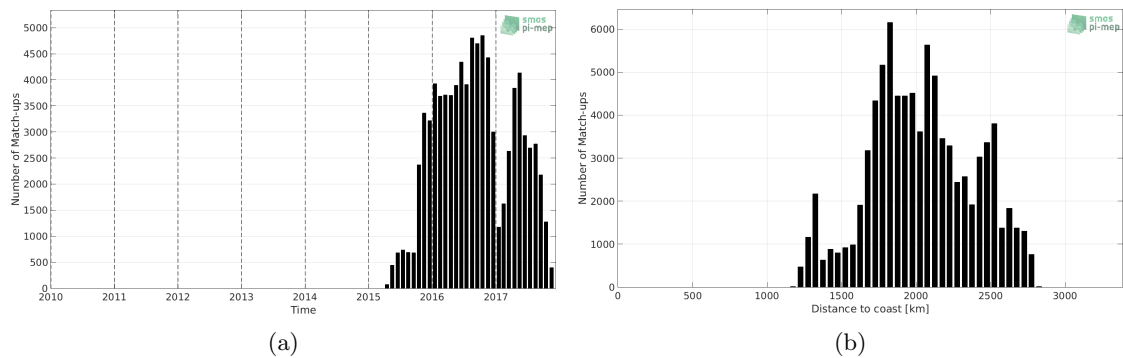
Figure 1: Number of match-ups between Surface drifters and SMOS-L3-CATDS-CECOS-LOCEAN-V4-9DAYS-25KM SSS as a function of time (a) and as function of the distance to coast (b) over the OTT zone Pi-MEP region and for the full satellite product period.
