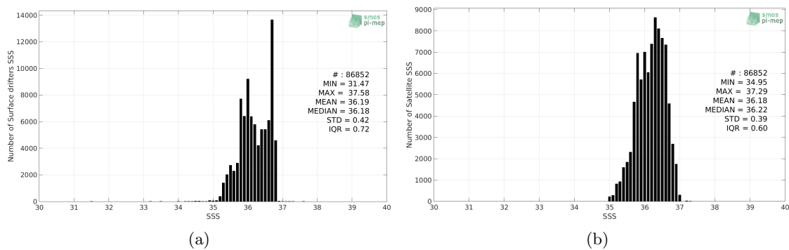
Figure 2: Histograms of SSS from Surface drifters (a) and SMOS-L3-CATDS-CECOS-LOCEAN-V4-9DAYS-25KM (b) considering all match-up pairs per bins of 0.1 over the OTT zone Pi-MEP region and for the full satellite product period.
