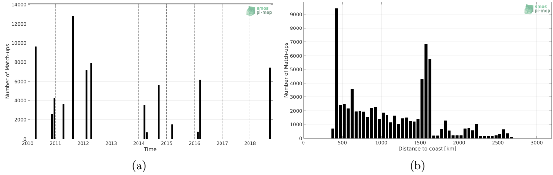
Figure 1: Number of match-ups between TSG (SAMOS) and SMOS SSS L3 v4 - 18 Days (CATDS-CECOS-LOCEAN) SSS as a function of time (a) and as function of the distance to coast (b) over the OTT zone Pi-MEP region and for the full satellite product period.
