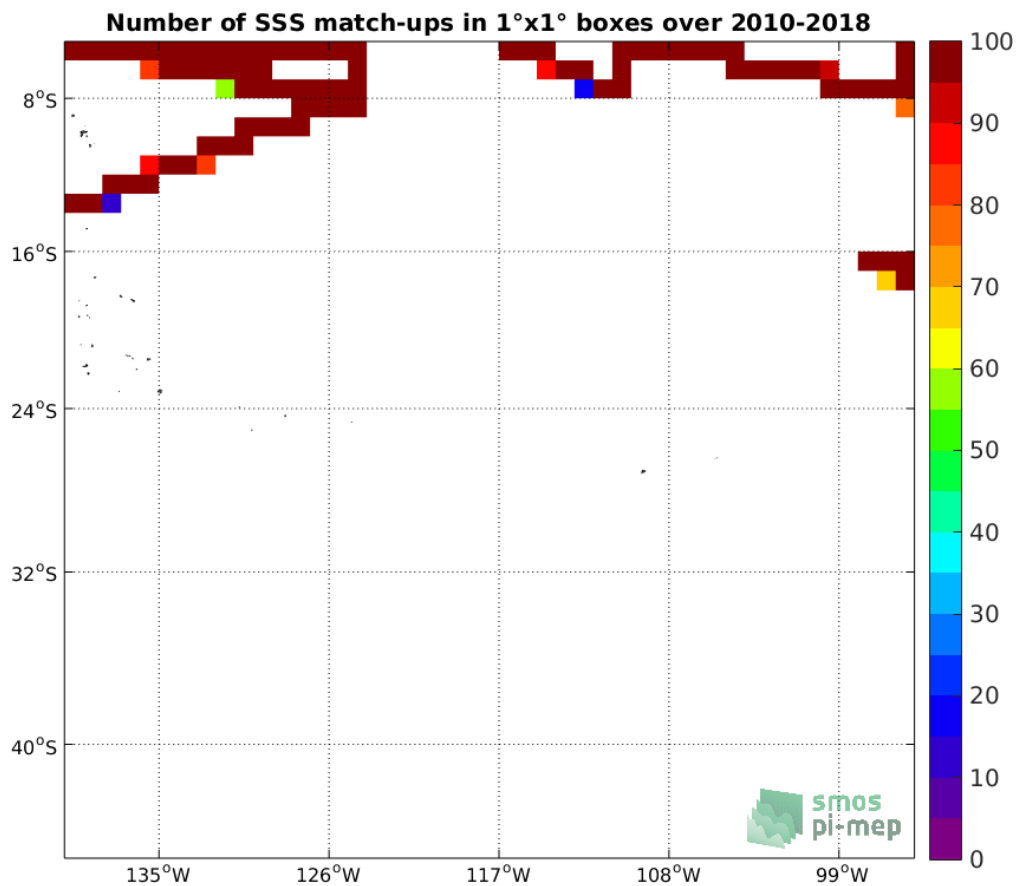
Figure 4: Number of SSS match-ups between TSG (SAMOS) SSS and the SMOS SSS L3 v4 - 18 Days (CATDS-CECOS-LOCEAN) SSS product for the OTT zone Pi-MEP region over 1°x1° boxes and for the full satellite product period.
