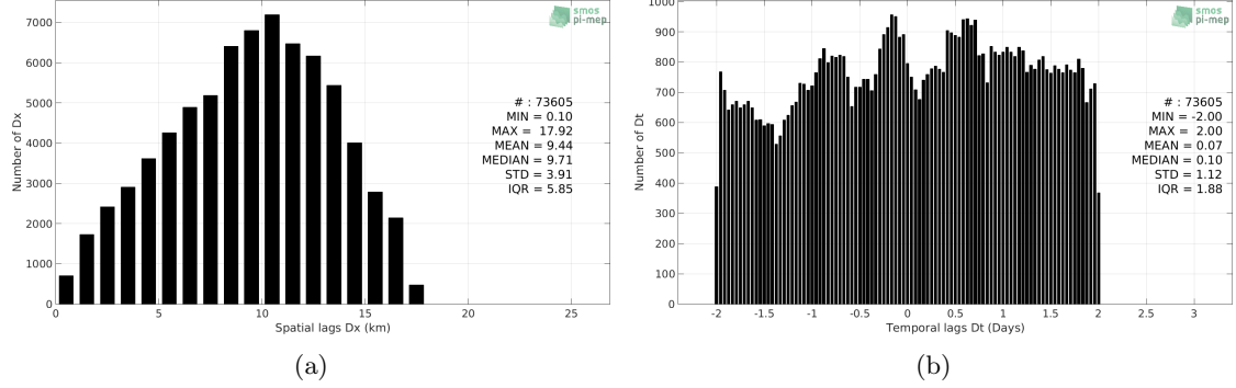
Figure 5: Histograms of the spatial (a) and temporal (b) lags between the time of the TSG (SAMOS) measurements and the date of the corresponding SMOS SSS L3 v4 - 18 Days (CATDS-CECOS-LOCEAN) SSS product.
