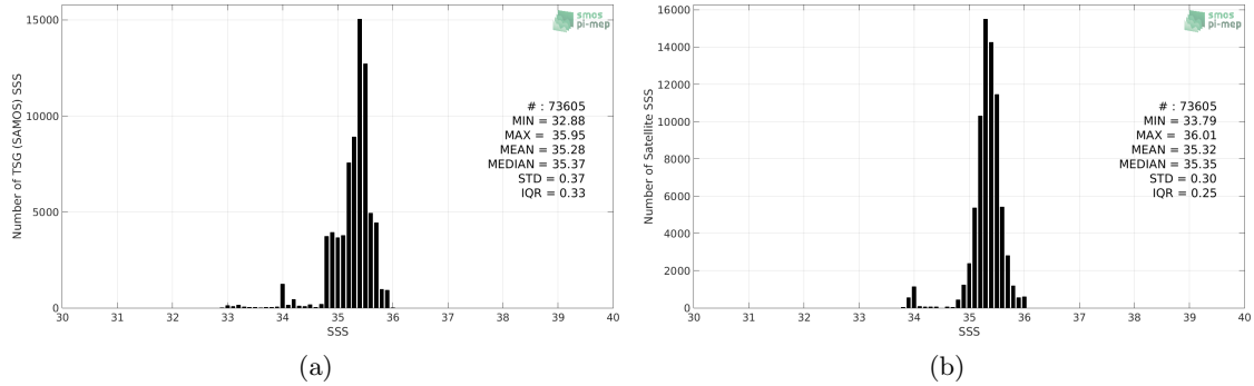
Figure 2: Histograms of SSS from TSG (SAMOS) (a) and SMOS SSS L3 v4 - 18 Days (CATDS-CECOS-LOCEAN) (b) considering all match-up pairs per bins of 0.1 over the OTT zone Pi-MEP region and for the full satellite product period.
