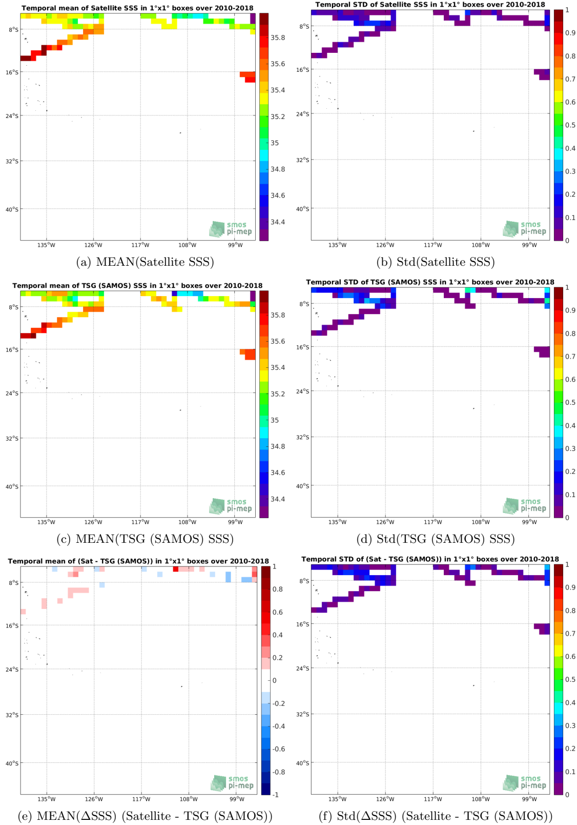
Figure 6: Temporal mean (left) and Std (right) of SSS from SMOS SSS L3 v4 - 18 Days (CATDS-CECOS-LOCEAN) (top), TSG (SAMOS) (middle), and of \Delta SSS (Satellite - TSG (SAMOS)). Only match-up pairs are used to generate these maps.
