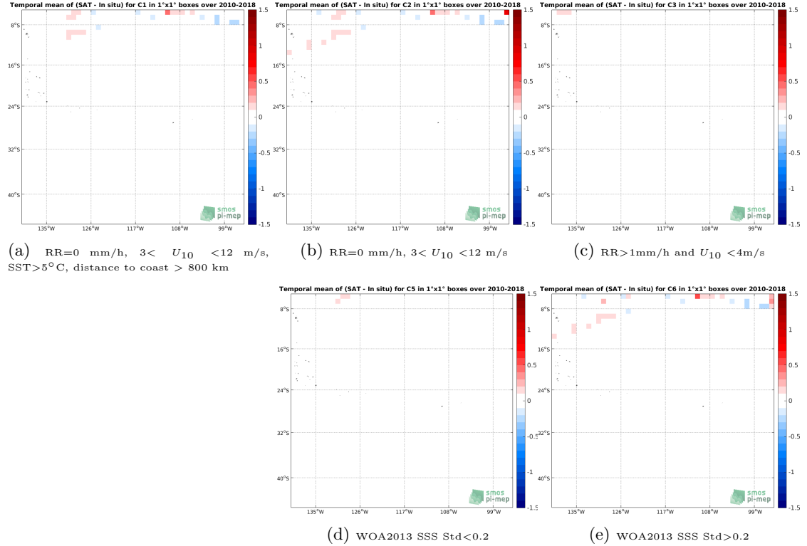
Figure 12: Temporal mean gridded over spatial boxes of size 1^{\circ}\times 1^{\circ} of \Delta\text{SSS} (SMOS SSS L3 v4 - 18 Days (CATDS-CECOS-LOCEAN) - TSG (SAMOS)) for 5 different subdatasets corresponding to: RR=0 mm/h, 3 < U_{10} < 12 m/s, SST >5^{\circ}\text{C} , distance to coast > 800 km (a), RR=0 mm/h, 3 < U_{10} < 12 m/s (b), RR >1 mm/h and U_{10} < 4 m/s (c), WOA2013 SSS Std <0.2 (d), WOA2013 SSS Std >0.2 (e).
