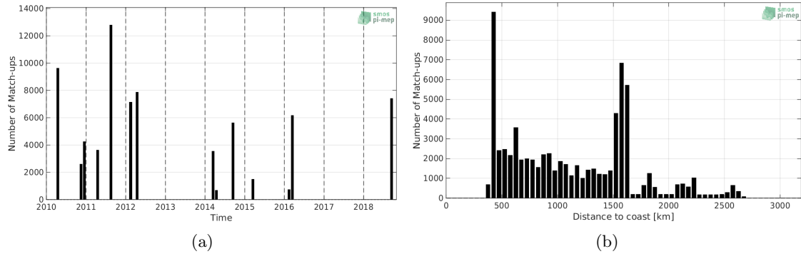
Figure 1: Number of match-ups between TSG-SAMOS and SMOS-L3-CATDS-CECOS-LOCEAN-V4-18DAYS-25KM SSS as a function of time (a) and as function of the distance to coast (b) over the OTT zone Pi-MEP region and for the full satellite product period.
