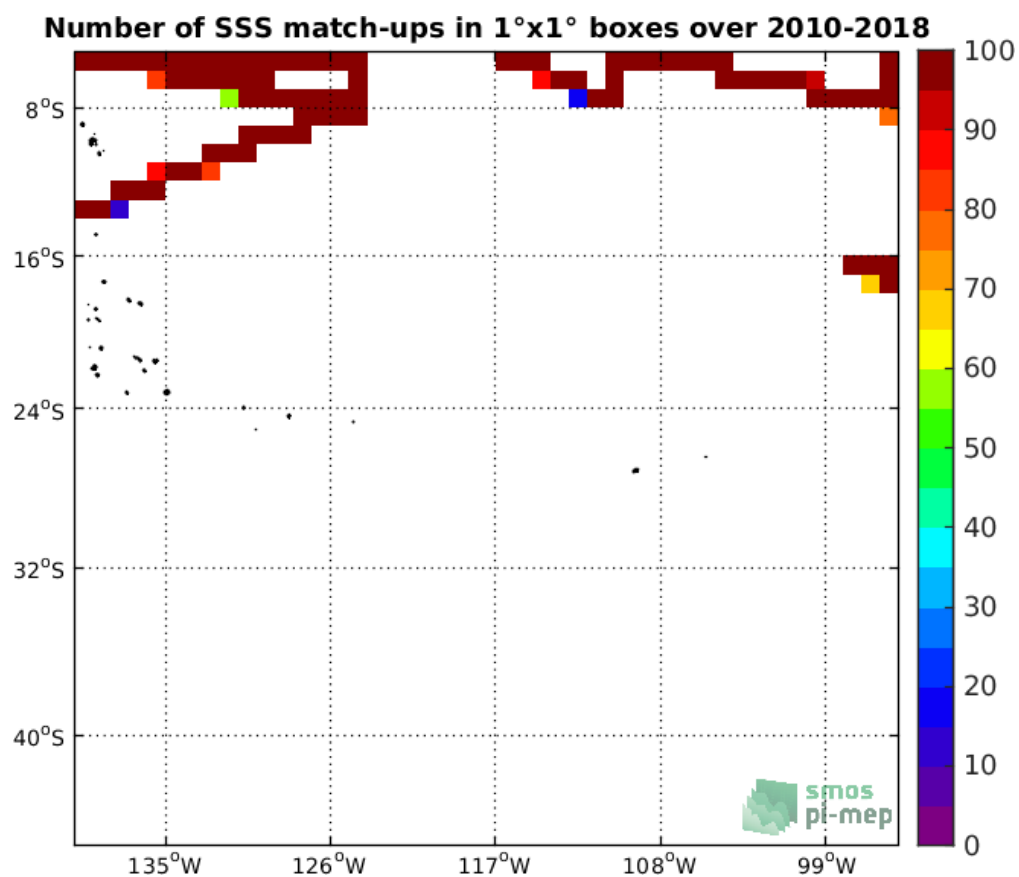
Figure 4: Number of SSS match-ups between TSG-SAMOS SSS and the SMOS-L3-CATDS-CECOS-LOCEAN-V4-18DAYS-25KM SSS product for the OTT zone Pi-MEP region over 1°x1° boxes and for the full satellite product period.
