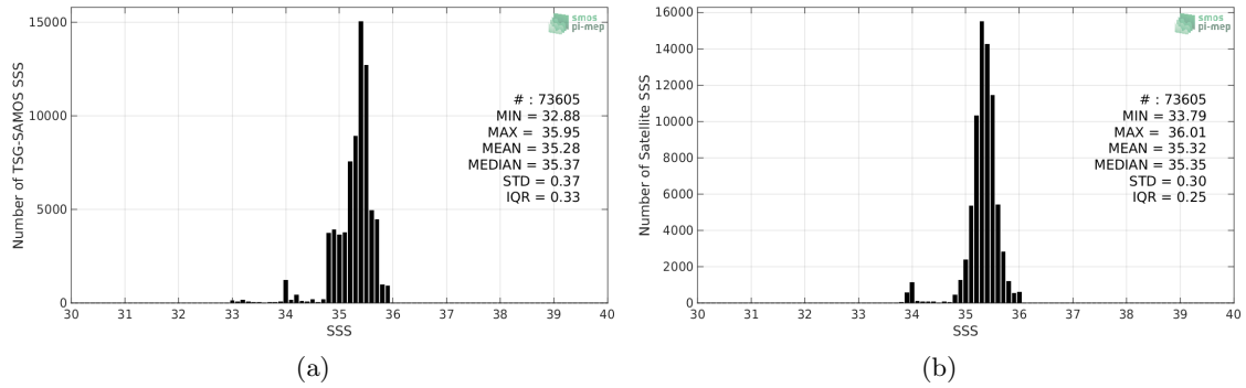
Figure 2: Histograms of SSS from TSG-SAMOS (a) and SMOS-L3-CATDS-CECOS-LOCEAN-V4-18DAYS-25KM (b) considering all match-up pairs per bins of 0.1 over the OTT zone Pi-MEP region and for the full satellite product period.
