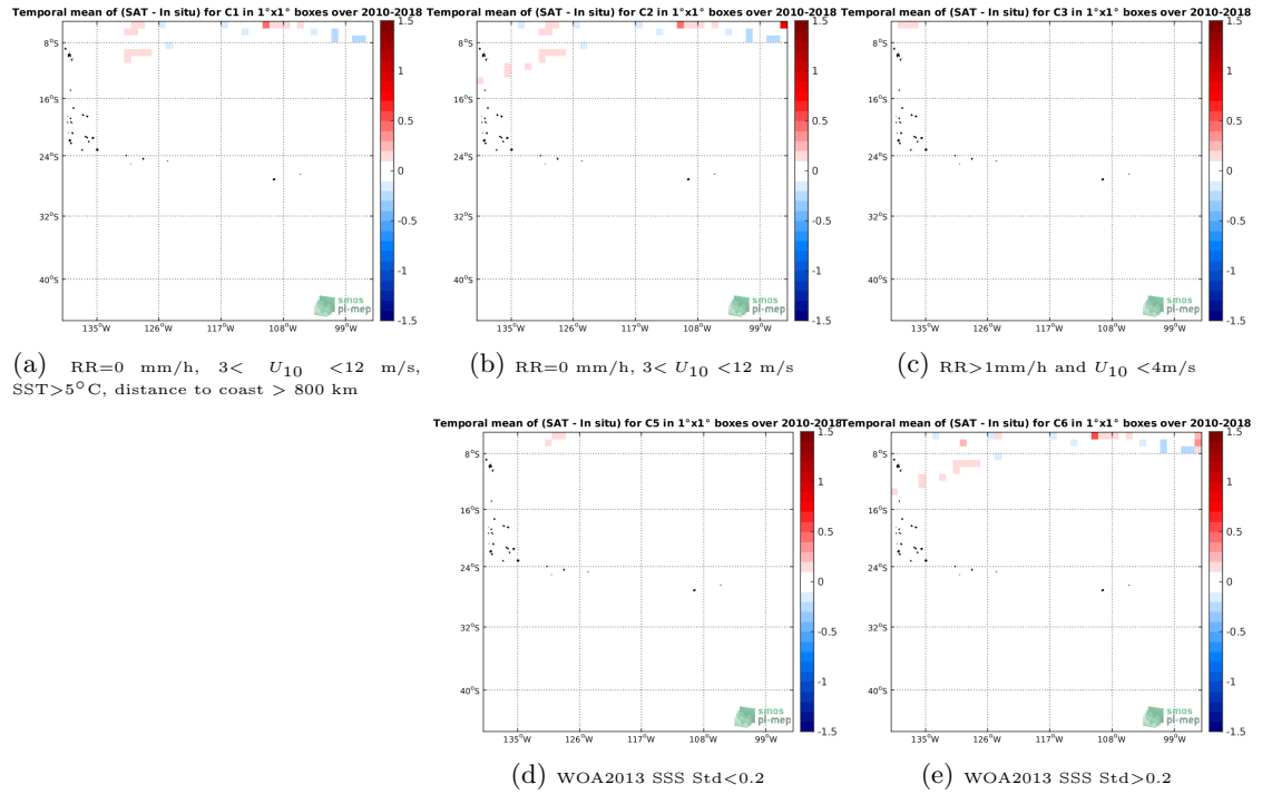
Figure 12: Temporal mean gridded over spatial boxes of size 1^\circ \times 1^\circ of \Delta SSS (SMOS-L3-CATDS-CECOS-LOCEAN-V4-18DAYS-25KM - TSG-SAMOS) for 5 different subdatasets corresponding to:RR=0 mm/h, 3 < U_{10} < 12 m/s, SST >5^\circ C, distance to coast > 800 km (a), RR=0 mm/h, 3 < U_{10} < 12 m/s (b), RR >1 mm/h and U_{10} < 4 m/s (c), WOA2013 SSS Std <0.2 (d), WOA2013 SSS Std >0.2 (e).
