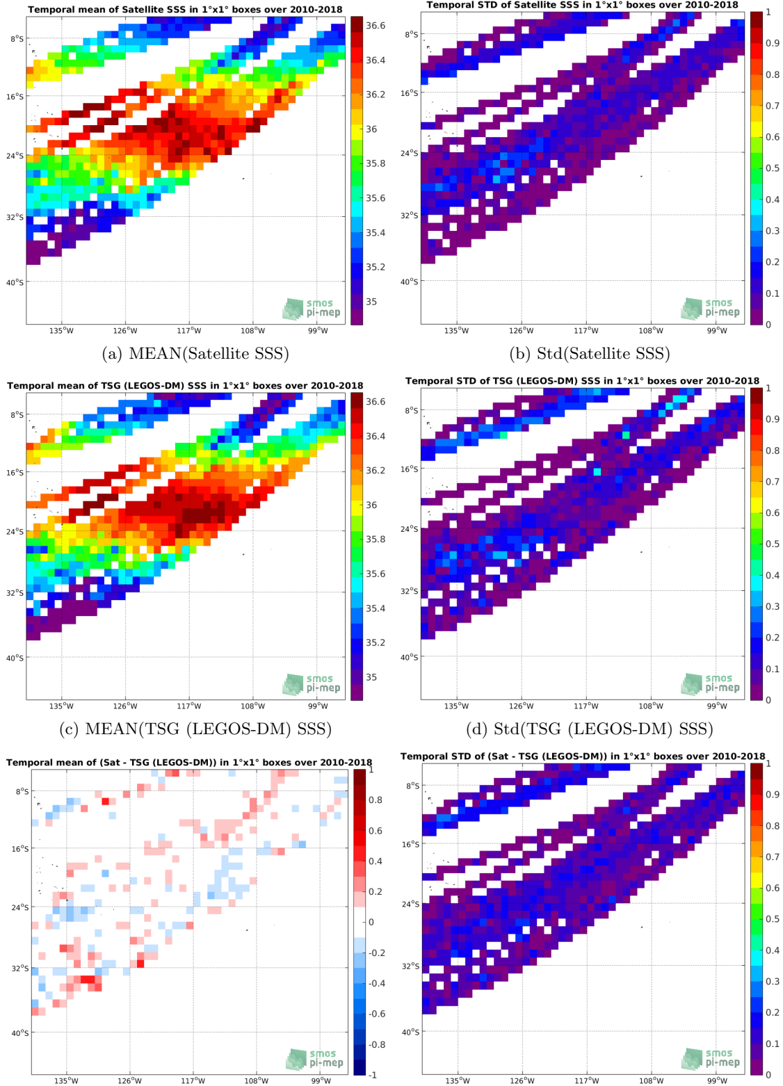
Figure 6: Temporal mean (left) and Std (right) of SSS from SMOS SSS L3 v4 - 18 Days (CATDS-CECOS-LOCEAN) (top), TSG (LEGOS-DM) (middle), and of \Delta SSS (Satellite - TSG (LEGOS-DM)). Only match-up pairs are used to generate these maps.
