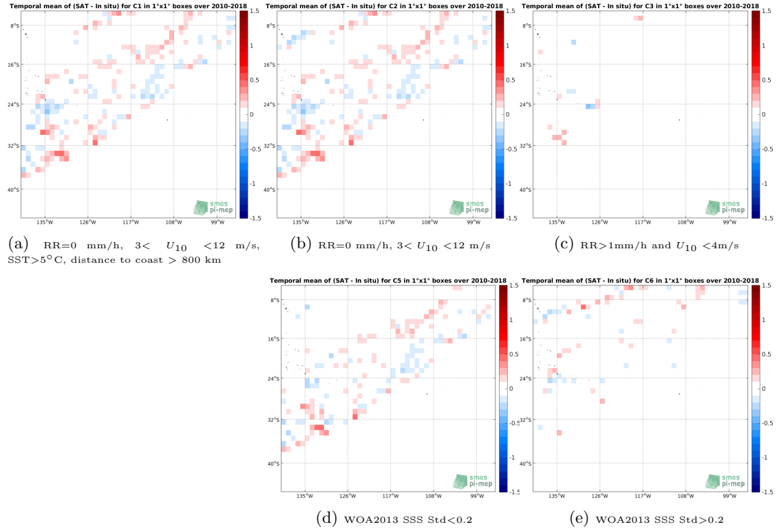
Figure 12: Temporal mean gridded over spatial boxes of size 1^{\circ}\times 1^{\circ} of \Delta\text{SSS} (SMOS SSS L3 v4 - 18 Days (CATDS-CECOS-LOCEAN) - TSG (LEGOS-DM)) for 5 different subdatasets corresponding to:RR=0 mm/h, 3 < U_{10} < 12 m/s, SST >5^{\circ}\text{C} , distance to coast > 800 km (a), RR=0 mm/h, 3 < U_{10} < 12 m/s (b), RR >1 mm/h and U_{10} < 4 m/s (c), WOA2013 SSS Std <0.2 (d), WOA2013 SSS Std >0.2 (e).
