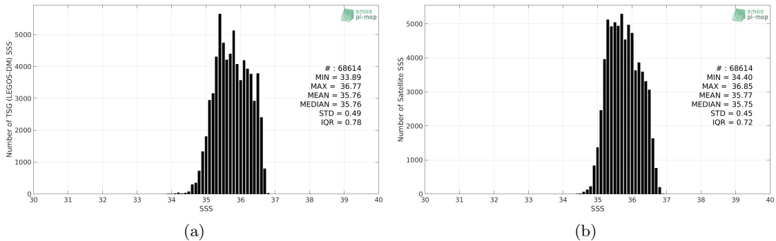
Figure 2: Histograms of SSS from TSG (LEGOS-DM) (a) and SMOS SSS L3 v4 - 18 Days (CATDS-CECOS-LOCEAN) (b) considering all match-up pairs per bins of 0.1 over the OTT zone Pi-MEP region and for the full satellite product period.
