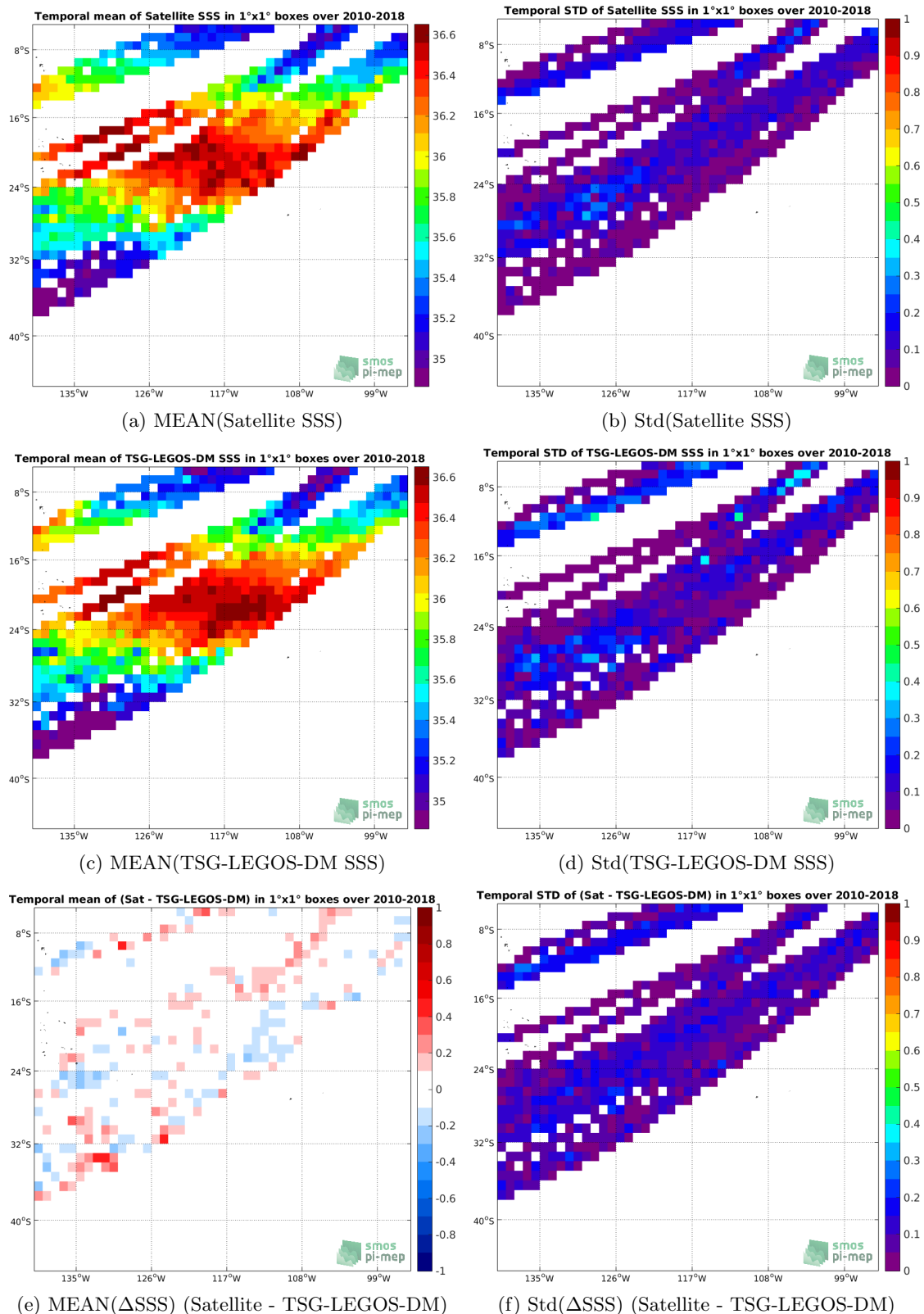
Figure 6: Temporal mean (left) and Std (right) of SSS from SMOS-L3-CATDS-CECOS-LOCEAN-V4-18DAYS-25KM (top), TSG-LEGOS-DM (middle), and of \Delta SSS (Satellite - TSG-LEGOS-DM). Only match-up pairs are used to generate these maps.
