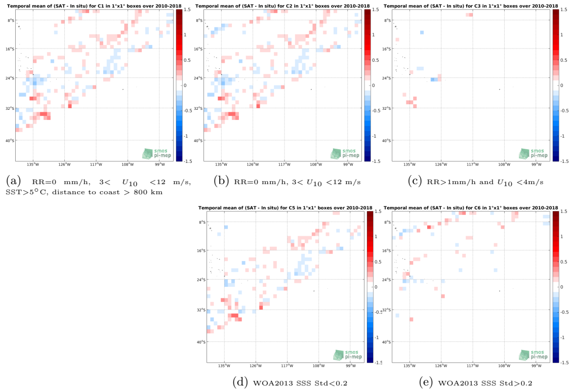
Figure 12: Temporal mean gridded over spatial boxes of size 1^{\circ}\times 1^{\circ} of \Delta\text{SSS} (SMOS-L3-CATDS-CECOS-LOCEAN-V4-18DAYS-25KM - TSG-LEGOS-DM) for 5 different subdatasets corresponding to:RR=0 mm/h, 3 < U_{10} < 12 m/s, \text{SST} > 5^{\circ}\text{C} , distance to coast > 800 km (a), RR=0 mm/h, 3 < U_{10} < 12 m/s (b), RR >1 mm/h and U_{10} < 4 m/s (c), WOA2013 SSS Std <0.2 (d), WOA2013 SSS Std >0.2 (e).
