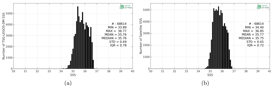
Figure 2: Histograms of SSS from TSG-LEGOS-DM (a) and SMOS-L3-CATDS-CECOS-LOCEAN-V4-18DAYS-25KM (b) considering all match-up pairs per bins of 0.1 over the OTT zone Pi-MEP region and for the full satellite product period.
