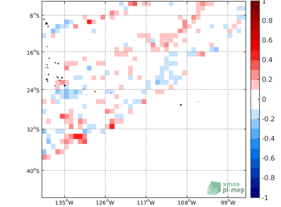
(e) MEAN( \Delta SSS) (Satellite - TSG-LEGOS-DM)
