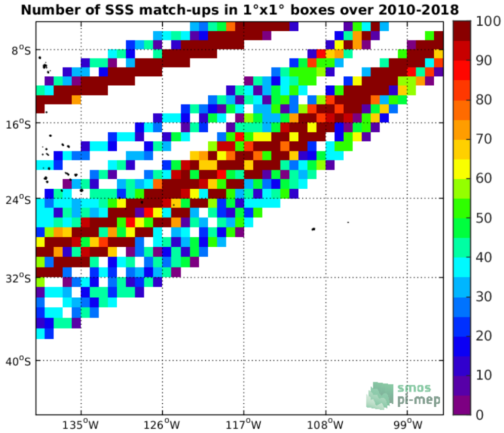
Figure 4: Number of SSS match-ups between TSG-LEGOS-DM SSS and the SMOS-L3-CATDS-CECOS-LOCEAN-V4-18DAYS-25KM SSS product for the OTT zone Pi-MEP region over 1°x1° boxes and for the full satellite product period.
