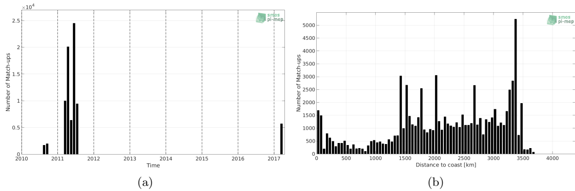
Figure 1: Number of match-ups between TSG-GOSUD-Sailing-ship and SMOS-L3-CATDS-CECOS-LOCEAN-V4-18DAYS-25KM SSS as a function of time (a) and as function of the distance to coast (b) over the OTT zone Pi-MEP region and for the full satellite product period.
