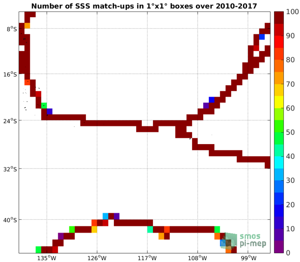
Figure 4: Number of SSS match-ups between TSG-GOSUD-Sailing-ship SSS and the SMOS-L3-CATDS-CECOS-LOCEAN-V4-18DAYS-25KM SSS product for the OTT zone Pi-MEP region over 1°x1° boxes and for the full satellite product period.
