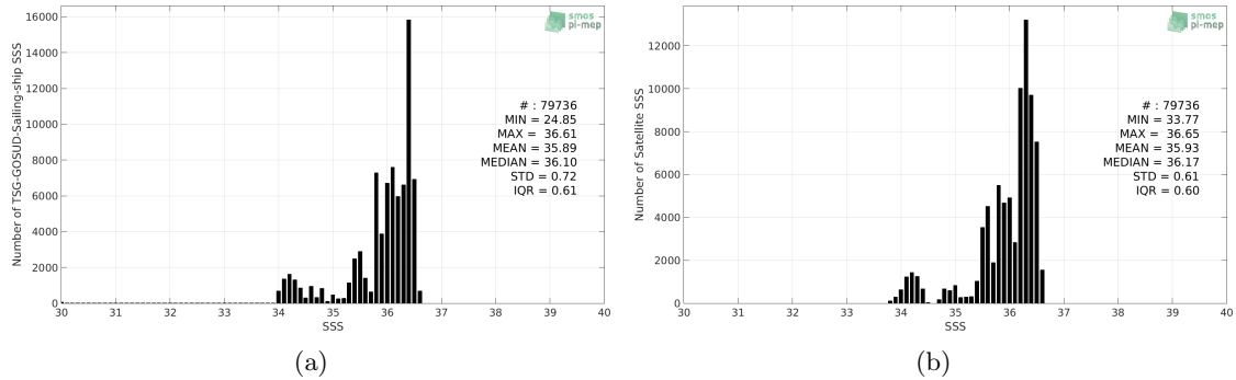
Figure 2: Histograms of SSS from TSG-GOSUD-Sailing-ship (a) and SMOS-L3-CATDS-CECOS-LOCEAN-V4-18DAYS-25KM (b) considering all match-up pairs per bins of 0.1 over the OTT zone Pi-MEP region and for the full satellite product period.
