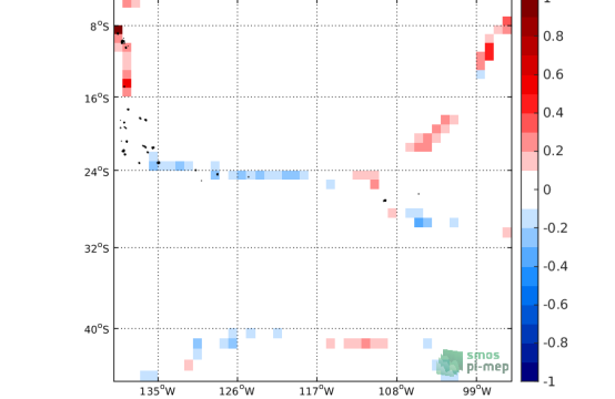
(e) MEAN( \Delta SSS) (Satellite - TSG-GOSUD-Sailing-ship)
