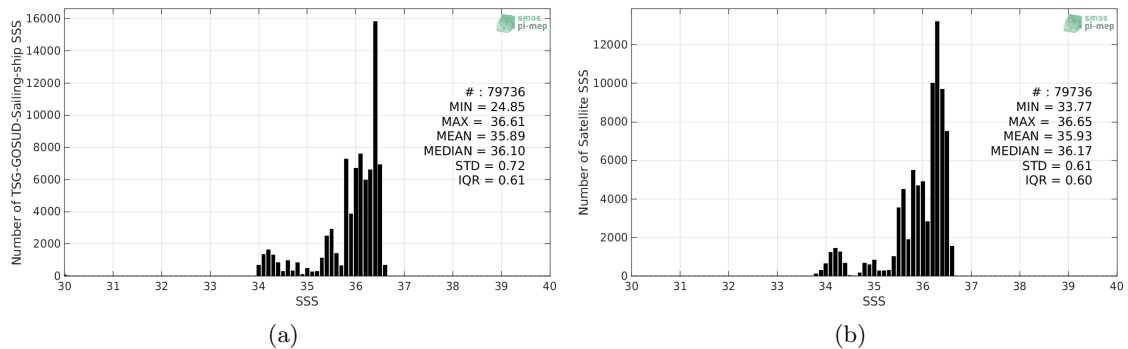
Figure 2: Histograms of SSS from TSG-GOSUD-Sailing-ship (a) and SMOS-L3-CATDS-CECOS-LOCEAN-V4-18DAYS-25KM (b) considering all match-up pairs per bins of 0.1 over the OTT zone Pi-MEP region and for the full satellite product period.
