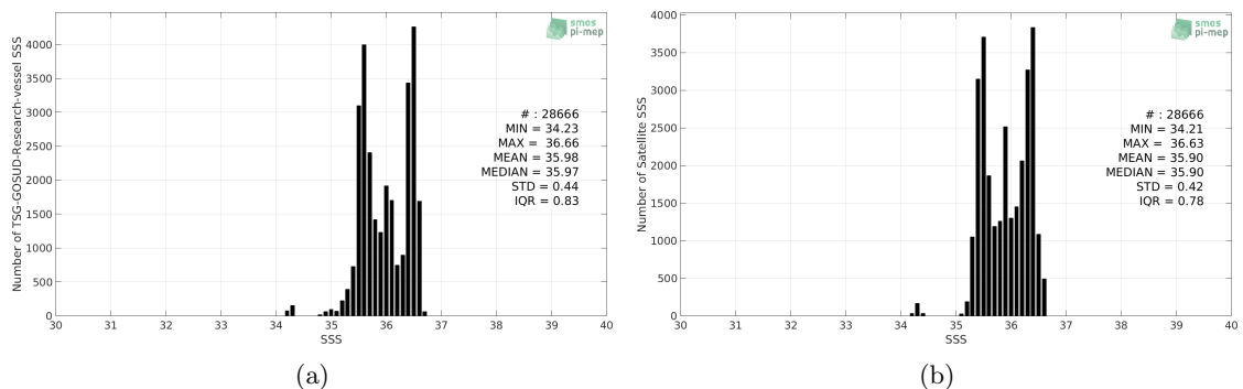
Figure 2: Histograms of SSS from TSG-GOSUD-Research-vessel (a) and SMOS-L3-CATDS-CECOS-LOCEAN-V4-18DAYS-25KM (b) considering all match-up pairs per bins of 0.1 over the OTT zone Pi-MEP region and for the full satellite product period.
