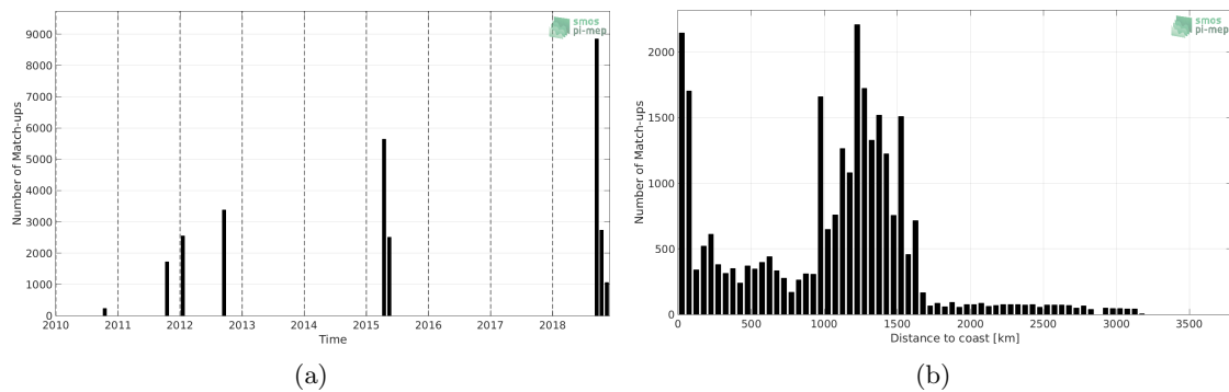
Figure 1: Number of match-ups between TSG-GOSUD-Research-vessel and SMOS-L3-CATDS-CECOS-LOCEAN-V4-18DAYS-25KM SSS as a function of time (a) and as function of the distance to coast (b) over the OTT zone Pi-MEP region and for the full satellite product period.
