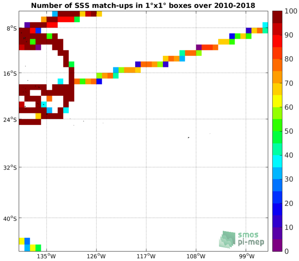
Figure 4: Number of SSS match-ups between TSG-GOSUD-Research-vessel SSS and the SMOS-L3-CATDS-CECOS-LOCEAN-V4-18DAYS-25KM SSS product for the OTT zone Pi-MEP region over 1°x1° boxes and for the full satellite product period.
