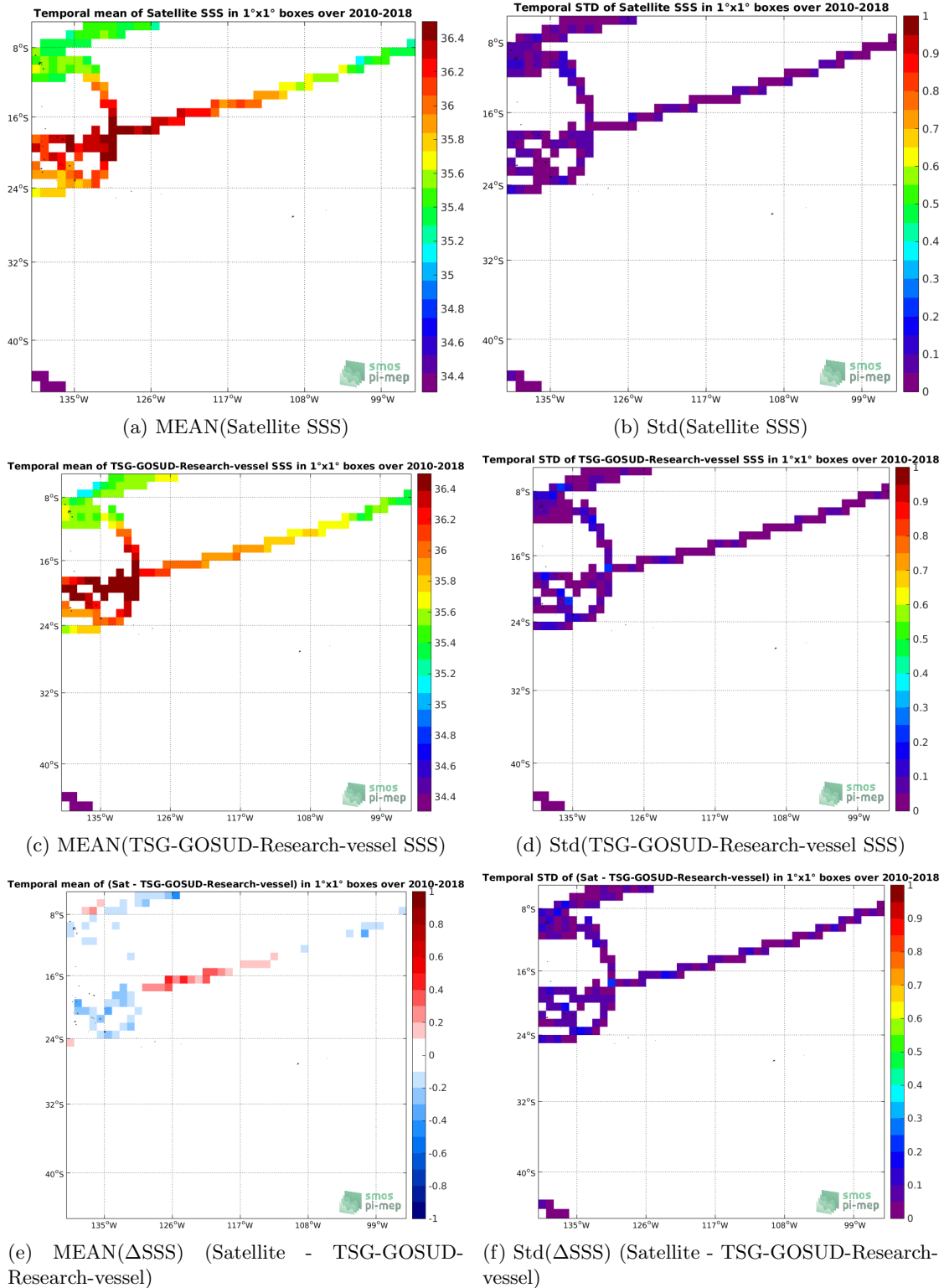
Figure 6: Temporal mean (left) and Std (right) of SSS from SMOS-L3-CATDS-CECOS-LOCEAN-V4-18DAYS-25KM (top), TSG-GOSUD-Research-vessel (middle), and of \Delta SSS (Satellite - TSG-GOSUD-Research-vessel). Only match-up pairs are used to generate these maps.
