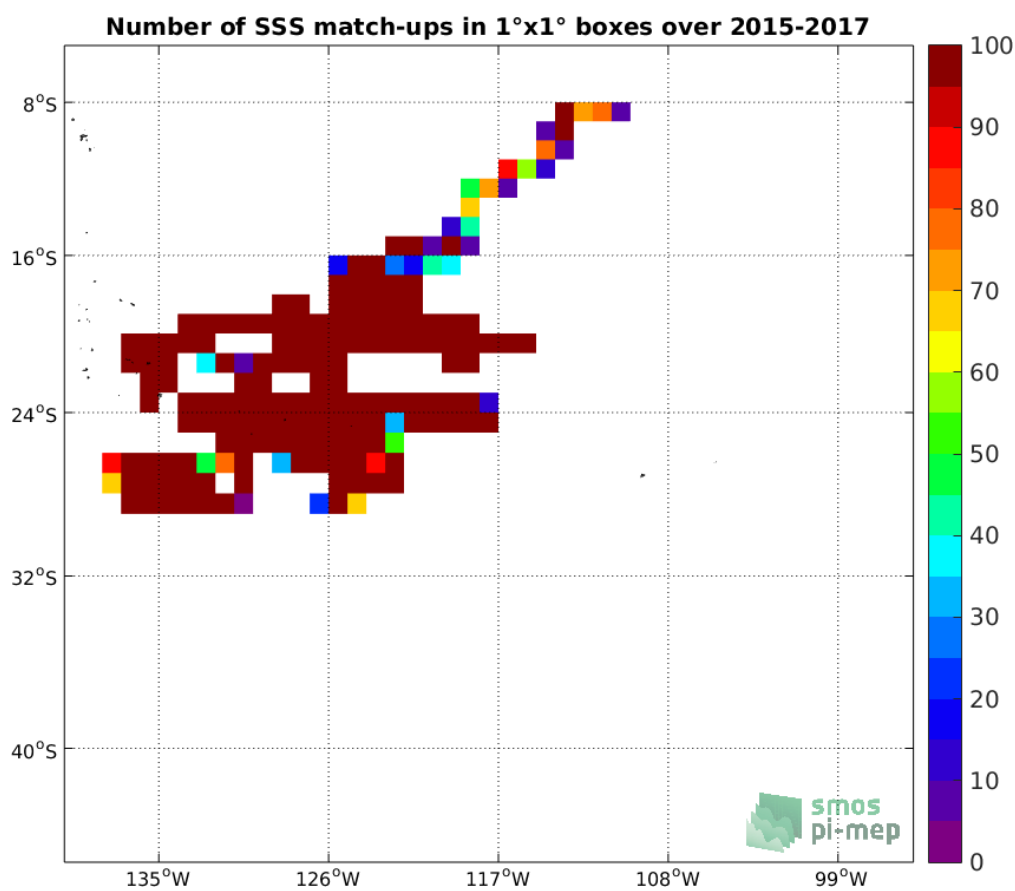
Figure 3: Number of SSS match-ups between Surface drifters SSS and the SMOS-L3-CATDS-CECOS-LOCEAN-V4-18DAYS-25KM SSS product for the OTT zone Pi-MEP region over 1°x1° boxes and for the full satellite product period.
