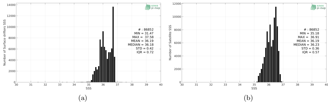
Figure 2: Histograms of SSS from Surface drifters (a) and SMOS-L3-CATDS-CECOS-LOCEAN-V4-18DAYS-25KM (b) considering all match-up pairs per bins of 0.1 over the OTT zone Pi-MEP region and for the full satellite product period.
