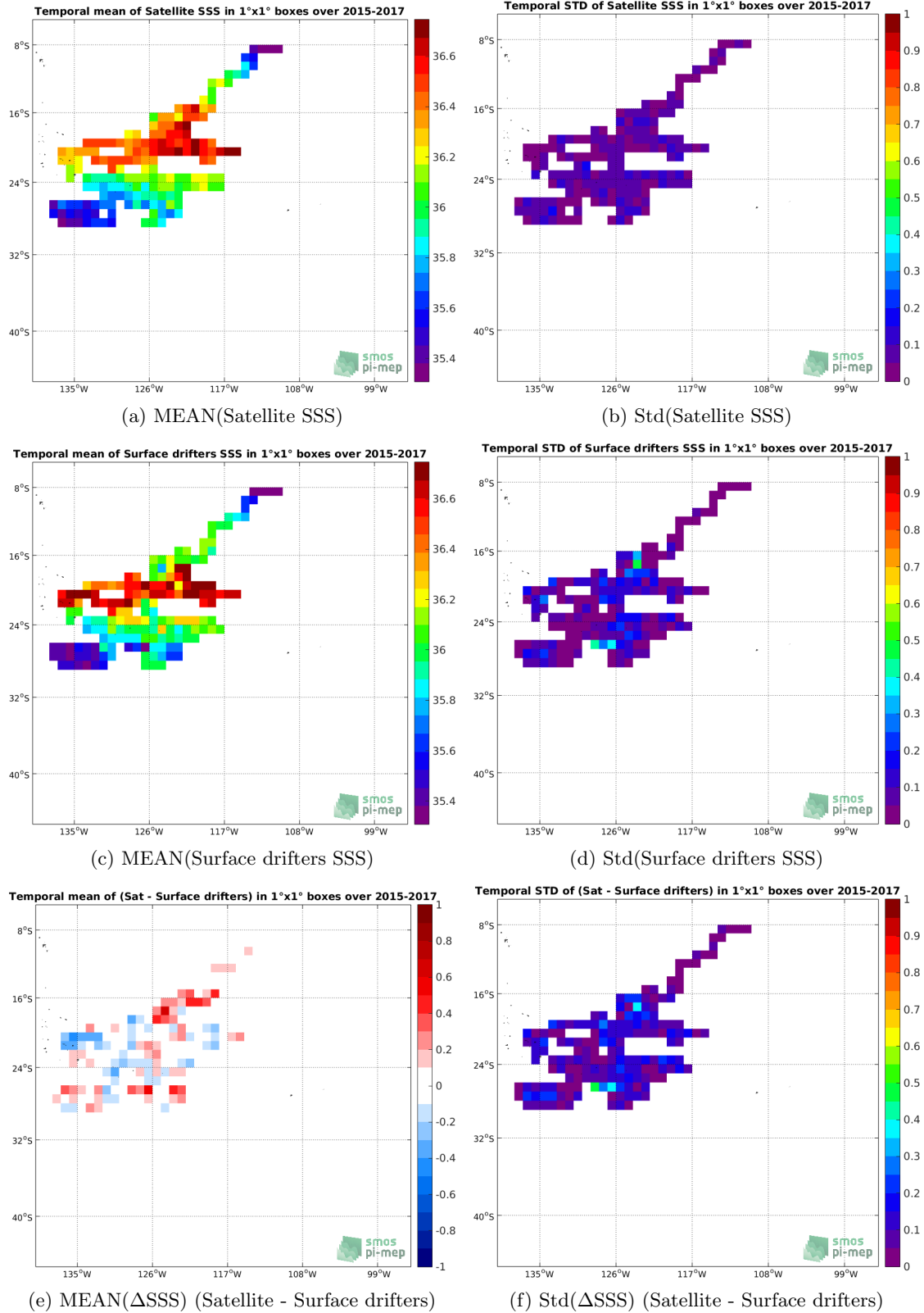
Figure 5: Temporal mean (left) and Std (right) of SSS from SMOS-L3-CATDS-CECOS-LOCEAN-V4-18DAYS-25KM (top), Surface drifters (middle), and of \Delta SSS (Satellite - Surface drifters). Only match-up pairs are used to generate these maps.
