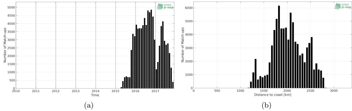
Figure 1: Number of match-ups between Surface drifters and SMOS-L3-CATDS-CECOS-LOCEAN-V4-18DAYS-25KM SSS as a function of time (a) and as function of the distance to coast (b) over the OTT zone Pi-MEP region and for the full satellite product period.
