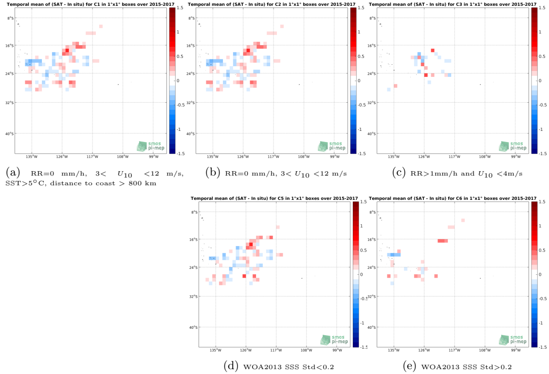
Figure 11: Temporal mean gridded over spatial boxes of size 1^{\circ}\times 1^{\circ} of \Delta\text{SSS} (SMOS-L3-CATDS-CECOS-LOCEAN-V4-18DAYS-25KM - Surface drifters) for 5 different subdatasets corresponding to: \text{RR}=0 mm/h, 3 < U_{10} < 12 m/s, \text{SST}>5^{\circ}\text{C} , distance to coast > 800 km (a), \text{RR}=0 mm/h, 3 < U_{10} < 12 m/s (b), \text{RR}>1\text{mm/h} and U_{10} < 4\text{m/s} (c), WOA2013 SSS Std <0.2 (d), WOA2013 SSS Std >0.2 (e).
