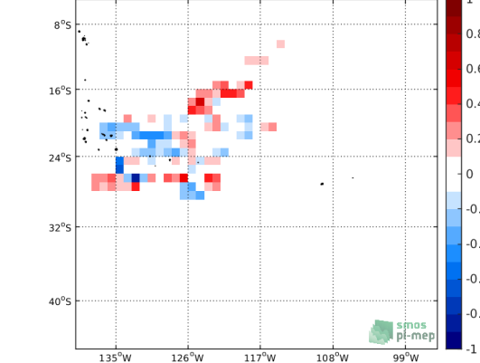
(e) MEAN( \Delta SSS) (Satellite - Surface drifters)
