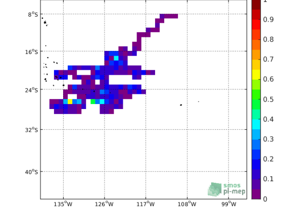
(f) Std( \Delta SSS) (Satellite - Surface drifters)
