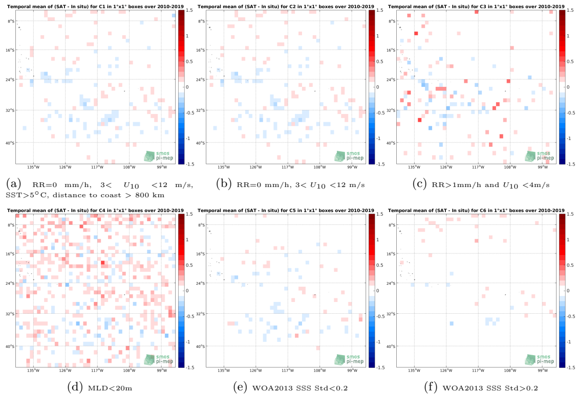
Figure 12: Temporal mean gridded over spatial boxes of size 1^\circ \times 1^\circ of \Delta SSS (SMOS SSS L3 v4 - 18 Days (CATDS-CECOS-LOCEAN) - Argo) for 6 different subdatasets corresponding to:RR=0 mm/h, 3 < U_{10} < 12 m/s, SST >5^\circ C, distance to coast > 800 km (a), RR=0 mm/h, 3 < U_{10} < 12 m/s (b), RR >1 mm/h and U_{10} < 4 m/s (c),MLD <20 m (d),WOA2013 SSS Std <0.2 (e),WOA2013 SSS Std >0.2 (f).
