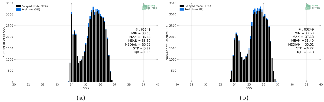
Figure 2: Histograms of SSS from Argo (a) and SMOS SSS L3 v4 - 18 Days (CATDS-CECOS-LOCEAN) (b) considering all match-up pairs per bins of 0.1 over the OTT zone Pi-MEP region and for the full satellite product period.
