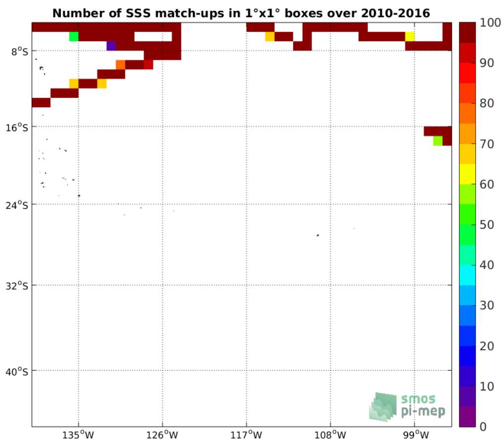
Figure 4: Number of SSS match-ups between TSG-SAMOS SSS and the SMOS-L3-CATDS-CECOS-LOCEAN-V3-9DAYS-25KM SSS product for the OTT zone Pi-MEP region over 1°x1° boxes and for the full satellite product period.
