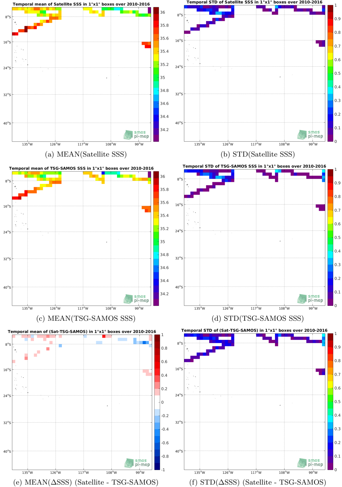
Figure 6: Temporal mean (left) and STD (right) of SSS from SMOS-L3-CATDS-CECOS-LOCEAN-V3-9DAYS-25KM (top), TSG-SAMOS (middle), and of \Delta SSS (Satellite - TSG-SAMOS). Only match-up pairs are used to generate these maps.
