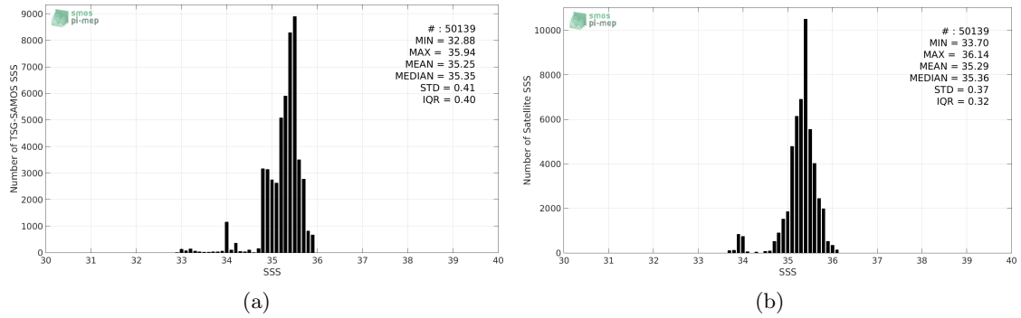
Figure 2: Histograms of SSS from TSG-SAMOS (a) and SMOS-L3-CATDS-CECOS-LOCEAN-V3-9DAYS-25KM (b) considering all match-up pairs per bins of 0.1 over the OTT zone Pi-MEP region and for the full satellite product period.
