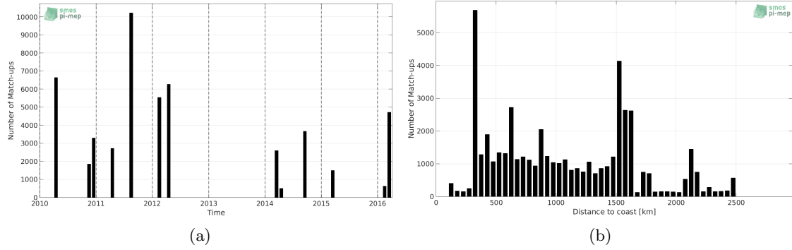
Figure 1: Number of match-ups between TSG-SAMOS and SMOS-L3-CATDS-CECOS-LOCEAN-V3-9DAYS-25KM SSS as a function of time (a) and as function of the distance to coast (b) over the OTT zone Pi-MEP region and for the full satellite product period.
