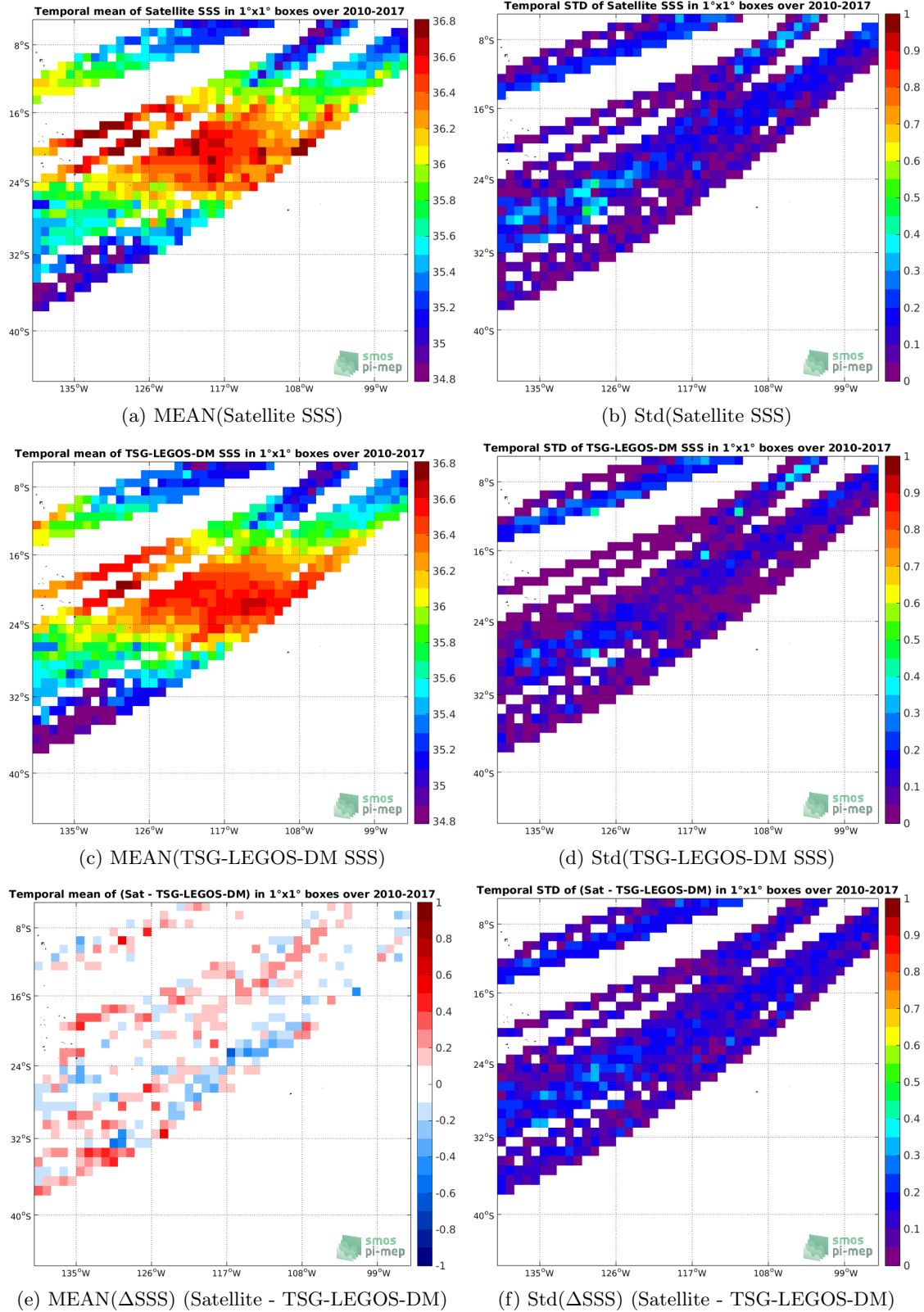
Figure 6: Temporal mean (left) and Std (right) of SSS from SMOS-L3-CATDS-CECOS-LOCEAN-V3-9DAYS-25KM (top), TSG-LEGOS-DM (middle), and of \Delta SSS (Satellite - TSG-LEGOS-DM). Only match-up pairs are used to generate these maps.
