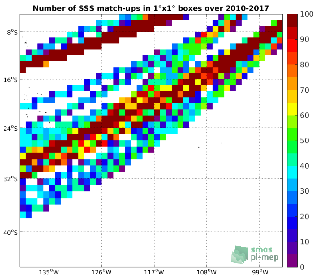
Figure 4: Number of SSS match-ups between TSG-LEGOS-DM SSS and the SMOS-L3-CATDS-CECOS-LOCEAN-V3-9DAYS-25KM SSS product for the OTT zone Pi-MEP region over 1°x1° boxes and for the full satellite product period.
