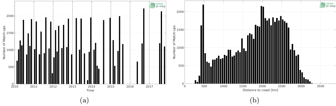
Figure 1: Number of match-ups between TSG-LEGOS-DM and SMOS-L3-CATDS-CECOS-LOCEAN-V3-9DAYS-25KM SSS as a function of time (a) and as function of the distance to coast (b) over the OTT zone Pi-MEP region and for the full satellite product period.
