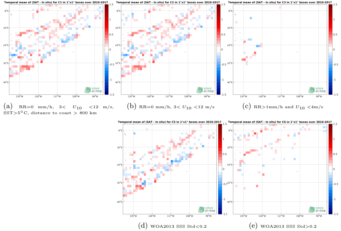
Figure 12: Temporal mean gridded over spatial boxes of size 1^\circ \times 1^\circ of \Delta SSS (SMOS-L3-CATDS-CECOS-LOCEAN-V3-9DAYS-25KM - TSG-LEGOS-DM) for 5 different subdatasets corresponding to: RR=0 mm/h, 3 < U_{10} < 12 m/s, SST >5^\circ C, distance to coast > 800 km (a), RR=0 mm/h, 3 < U_{10} < 12 m/s (b), RR >1 mm/h and U_{10} < 4 m/s (c), WOA2013 SSS Std <0.2 (d), WOA2013 SSS Std >0.2 (e).
