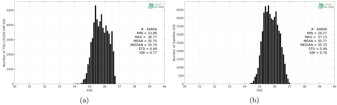
Figure 2: Histograms of SSS from TSG-LEGOS-DM (a) and SMOS-L3-CATDS-CECOS-LOCEAN-V3-9DAYS-25KM (b) considering all match-up pairs per bins of 0.1 over the OTT zone Pi-MEP region and for the full satellite product period.
