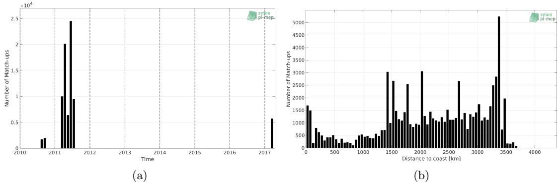
Figure 1: Number of match-ups between TSG-GOSUD-Sailing-ship and SMOS-L3-CATDS-CECOS-LOCEAN-V3-9DAYS-25KM SSS as a function of time (a) and as function of the distance to coast (b) over the OTT zone Pi-MEP region and for the full satellite product period.
