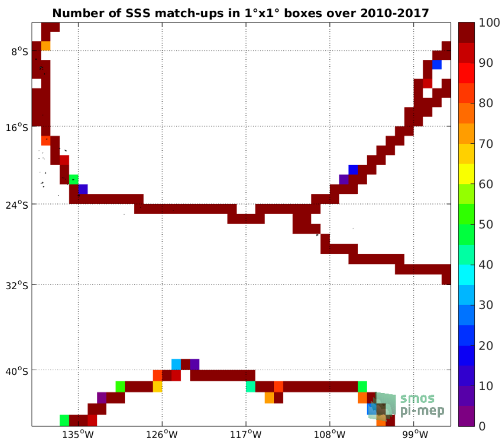
Figure 4: Number of SSS match-ups between TSG-GOSUD-Sailing-ship SSS and the SMOS-L3-CATDS-CECOS-LOCEAN-V3-9DAYS-25KM SSS product for the OTT zone Pi-MEP region over 1°x1° boxes and for the full satellite product period.
