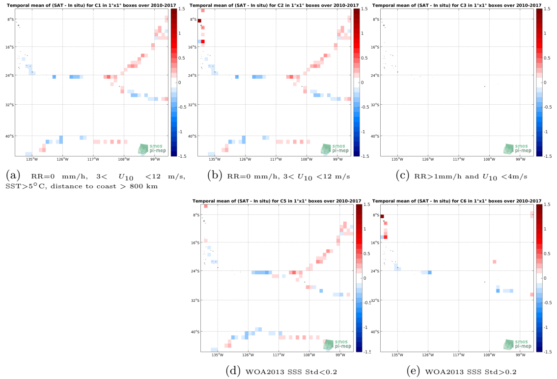
Figure 12: Temporal mean gridded over spatial boxes of size 1^\circ \times 1^\circ of \Delta SSS (SMOS-L3-CATDS-CECOS-LOCEAN-V3-9DAYS-25KM - TSG-GOSUD-Sailing-ship) for 5 different subdatasets corresponding to:RR=0 mm/h, 3 < U_{10} < 12 m/s, SST >5^\circ\text{C} , distance to coast > 800 km (a), RR=0 mm/h, 3 < U_{10} < 12 m/s (b), RR >1 mm/h and U_{10} < 4 m/s (c), WOA2013 SSS Std <0.2 (d), WOA2013 SSS Std >0.2 (e).
