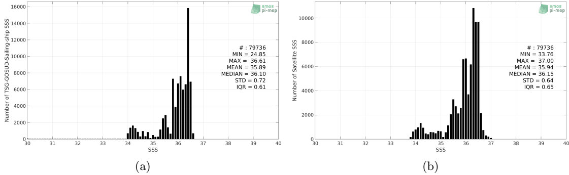
Figure 2: Histograms of SSS from TSG-GOSUD-Sailing-ship (a) and SMOS-L3-CATDS-CECOS-LOCEAN-V3-9DAYS-25KM (b) considering all match-up pairs per bins of 0.1 over the OTT zone Pi-MEP region and for the full satellite product period.
