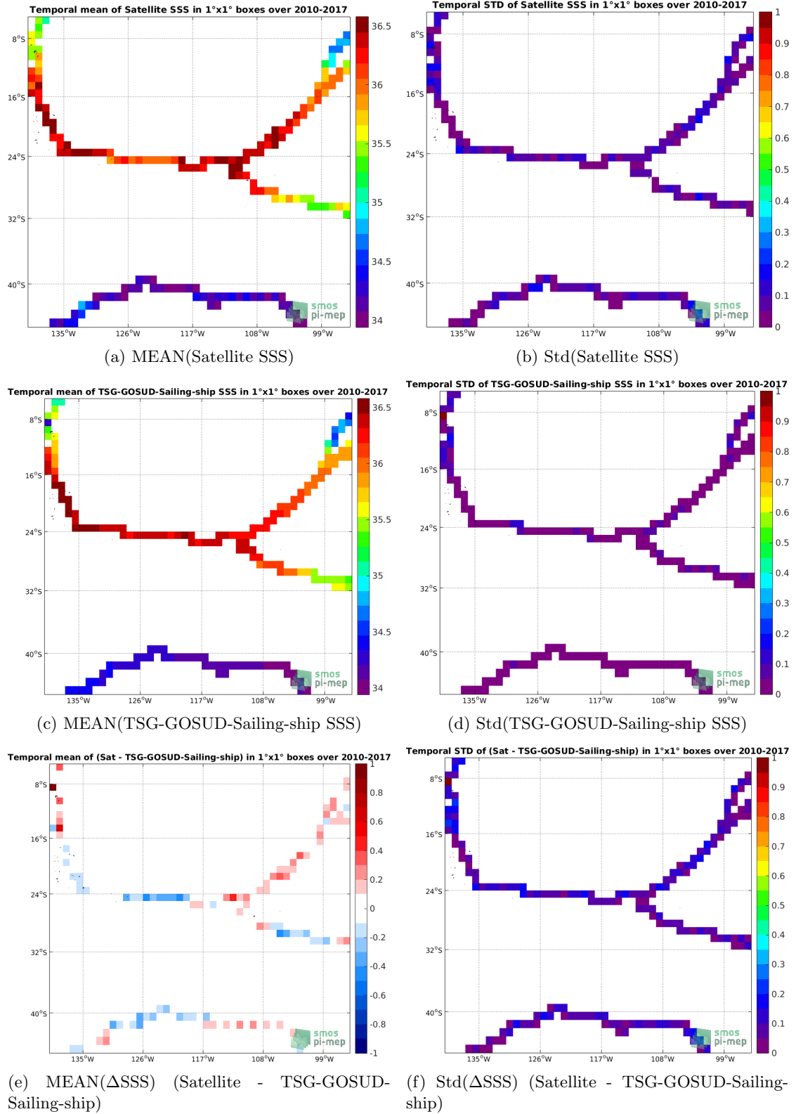
Figure 6: Temporal mean (left) and Std (right) of SSS from SMOS-L3-CATDS-CECOS-LOCEAN-V3-9DAYS-25KM (top), TSG-GOSUD-Sailing-ship (middle), and of \Delta SSS (Satellite - TSG-GOSUD-Sailing-ship). Only match-up pairs are used to generate these maps.
