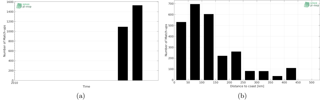
Figure 1: Number of match-ups between TSG-GOSUD-Sailing-ship and SMOS-L3-CATDS-CECOS-LOCEAN-V3-9DAYS-25KM SSS as a function of time (a) and as function of the distance to coast (b) over the OTT zone Pi-MEP region and for the full satellite product period.
