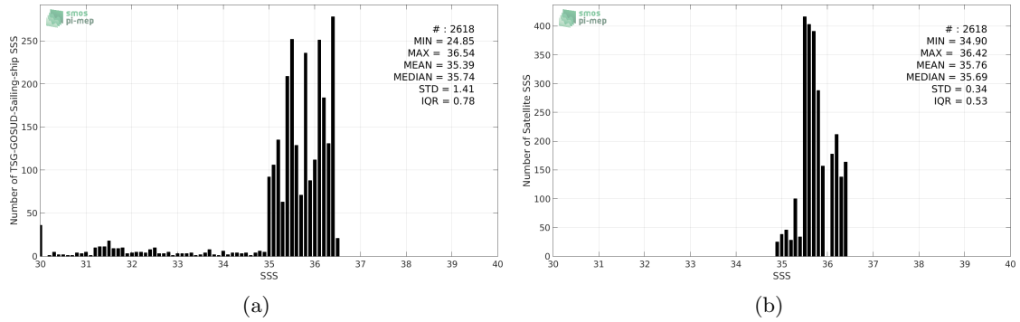
Figure 2: Histograms of SSS from TSG-GOSUD-Sailing-ship (a) and SMOS-L3-CATDS-CECOS-LOCEAN-V3-9DAYS-25KM (b) considering all match-up pairs per bins of 0.1 over the OTT zone Pi-MEP region and for the full satellite product period.
