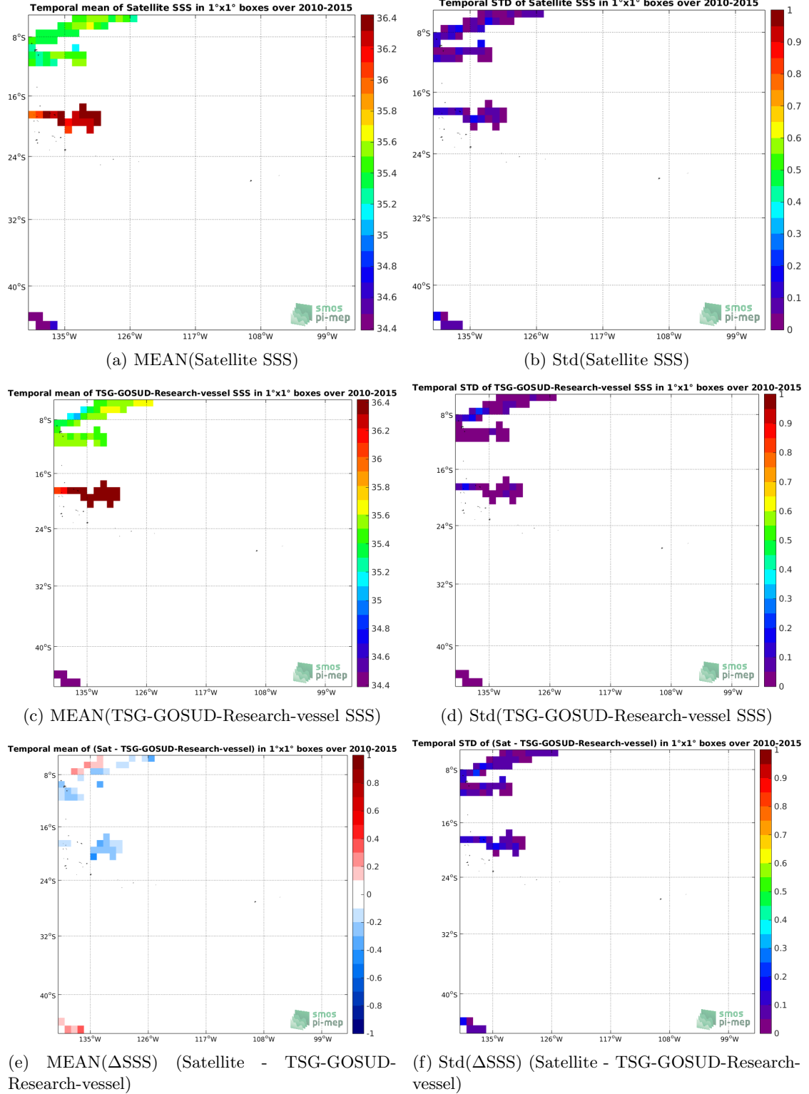
Figure 6: Temporal mean (left) and Std (right) of SSS from SMOS-L3-CATDS-CECOS-LOCEAN-V3-9DAYS-25KM (top), TSG-GOSUD-Research-vessel (middle), and of \Delta SSS (Satellite - TSG-GOSUD-Research-vessel). Only match-up pairs are used to generate these maps.
