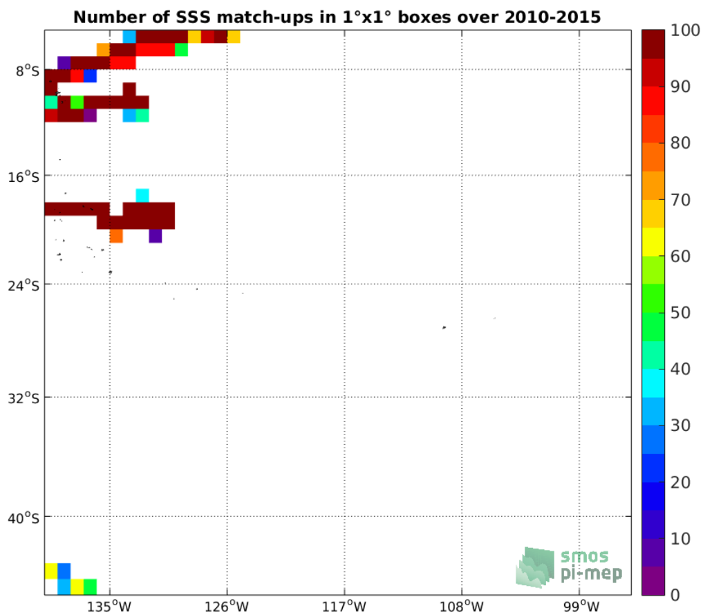
Figure 4: Number of SSS match-ups between TSG-GOSUD-Research-vessel SSS and the SMOS-L3-CATDS-CECOS-LOCEAN-V3-9DAYS-25KM SSS product for the OTT zone Pi-MEP region over 1°x1° boxes and for the full satellite product period.
