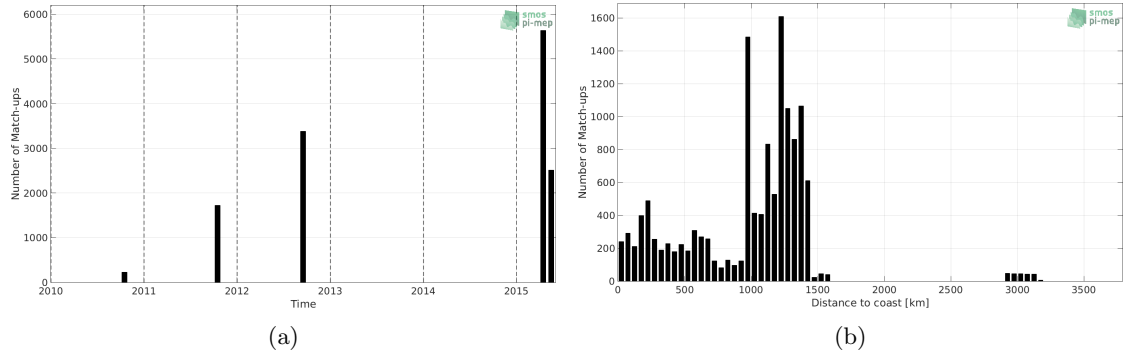
Figure 1: Number of match-ups between TSG-GOSUD-Research-vessel and SMOS-L3-CATDS-CECOS-LOCEAN-V3-9DAYS-25KM SSS as a function of time (a) and as function of the distance to coast (b) over the OTT zone Pi-MEP region and for the full satellite product period.
