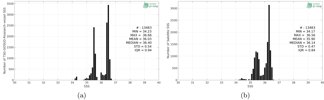
Figure 2: Histograms of SSS from TSG-GOSUD-Research-vessel (a) and SMOS-L3-CATDS-CECOS-LOCEAN-V3-9DAYS-25KM (b) considering all match-up pairs per bins of 0.1 over the OTT zone Pi-MEP region and for the full satellite product period.
