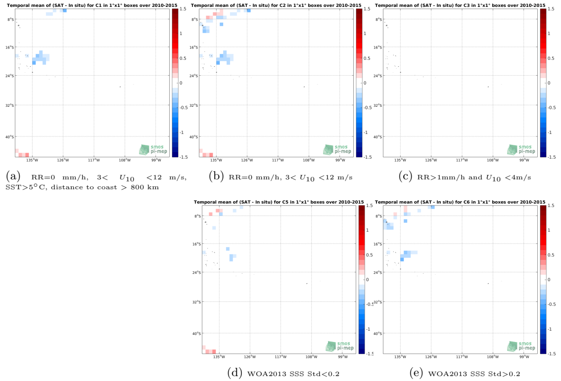
Figure 12: Temporal mean gridded over spatial boxes of size 1^\circ \times 1^\circ of \Delta SSS (SMOS-L3-CATDS-CECOS-LOCEAN-V3-9DAYS-25KM - TSG-GOSUD-Research-vessel) for 5 different subdatasets corresponding to:RR=0 mm/h, 3 < U_{10} < 12 m/s, SST >5^\circ\text{C} , distance to coast > 800 km (a), RR=0 mm/h, 3 < U_{10} < 12 m/s (b), RR >1 mm/h and U_{10} < 4 m/s (c), WOA2013 SSS Std <0.2 (d), WOA2013 SSS Std >0.2 (e).
