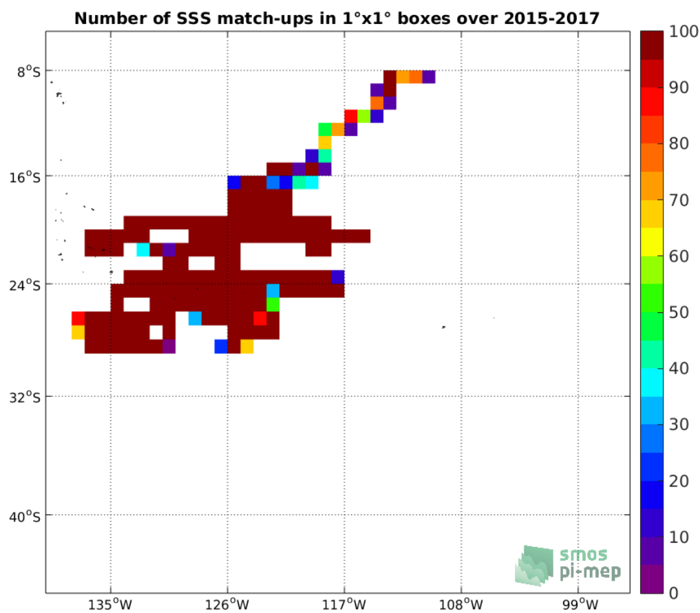
Figure 3: Number of SSS match-ups between Surface drifters SSS and the SMOS-L3-CATDS-CECOS-LOCEAN-V3-9DAYS-25KM SSS product for the OTT zone Pi-MEP region over 1°x1° boxes and for the full satellite product period.
