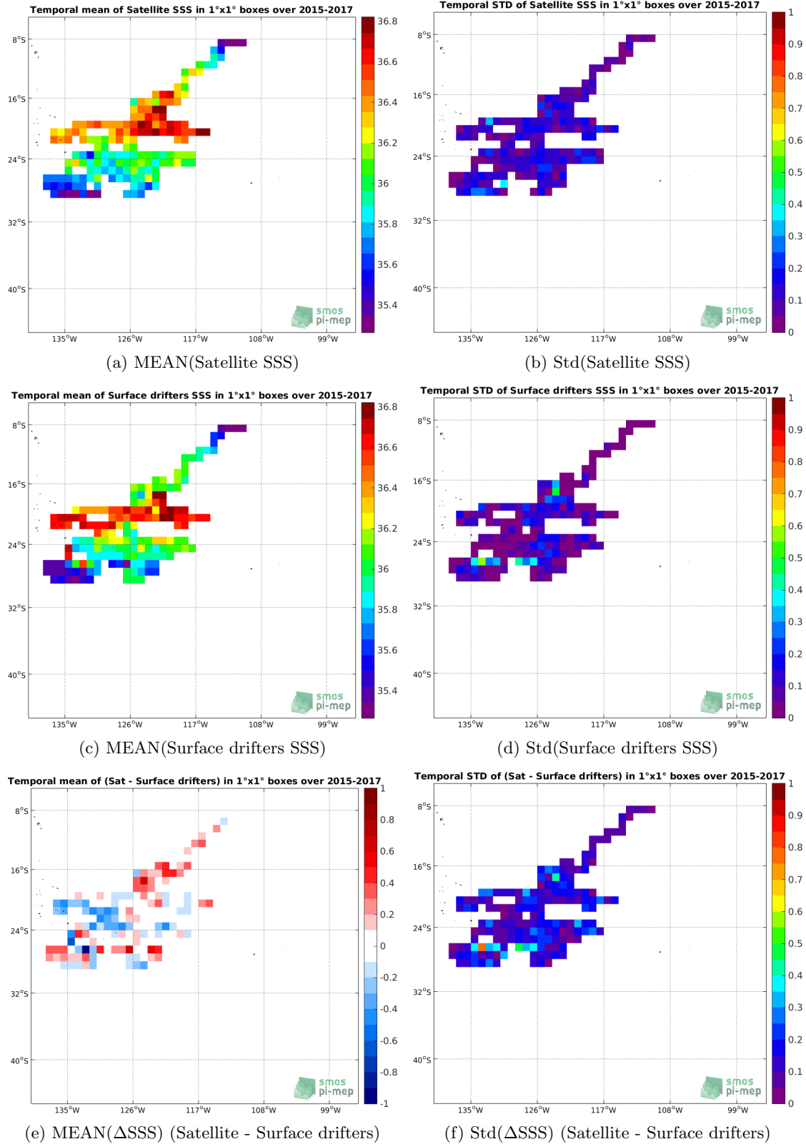
Figure 5: Temporal mean (left) and Std (right) of SSS from SMOS-L3-CATDS-CECOS-LOCEAN-V3-9DAYS-25KM (top), Surface drifters (middle), and of \Delta SSS (Satellite - Surface drifters). Only match-up pairs are used to generate these maps.
