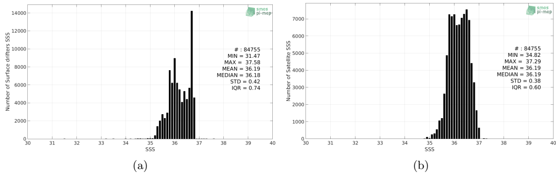
Figure 2: Histograms of SSS from Surface drifters (a) and SMOS-L3-CATDS-CECOS-LOCEAN-V3-9DAYS-25KM (b) considering all match-up pairs per bins of 0.1 over the OTT zone Pi-MEP region and for the full satellite product period.
