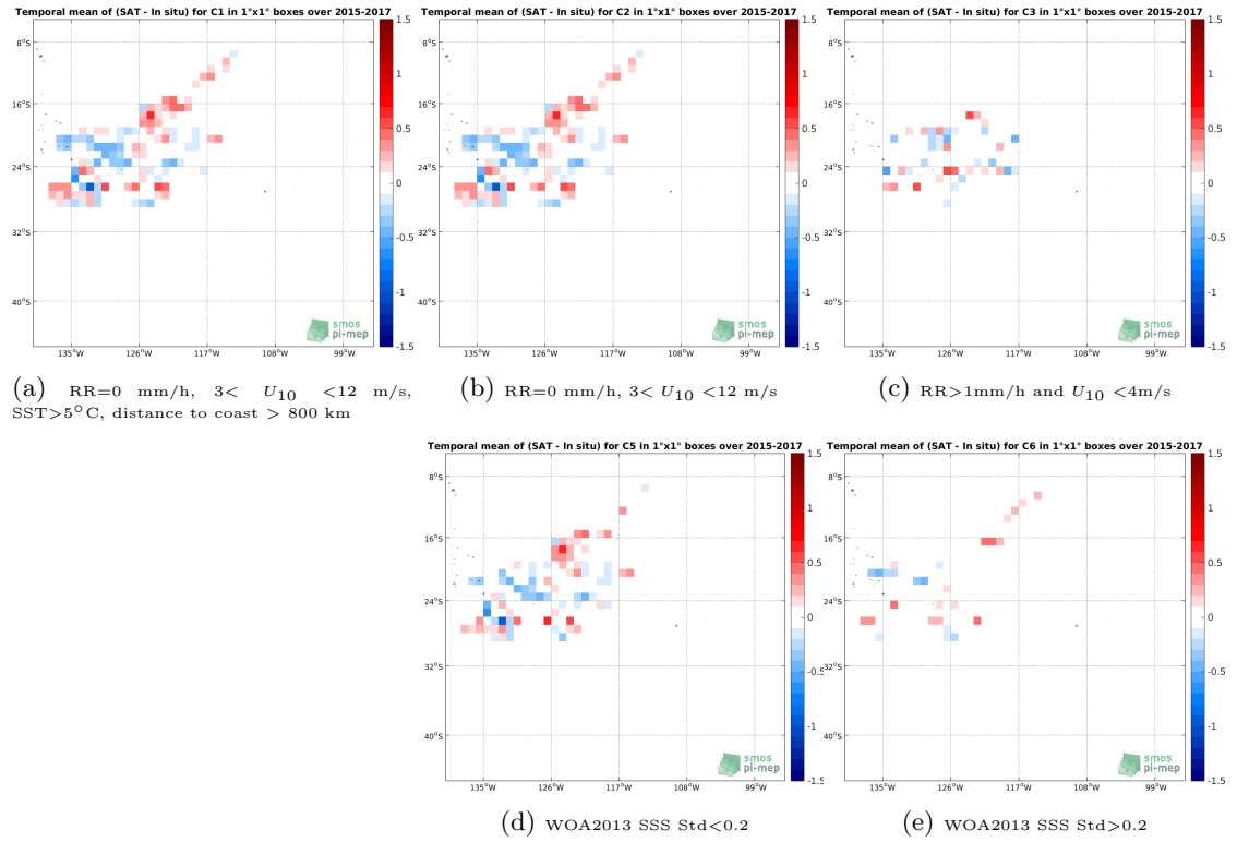
Figure 11: Temporal mean gridded over spatial boxes of size 1^\circ \times 1^\circ of \Delta SSS (SMOS-L3-CATDS-CECOS-LOCEAN-V3-9DAYS-25KM - Surface drifters) for 5 different subdatasets corresponding to: RR=0 mm/h, 3 < U_{10} < 12 m/s, SST>5°C, distance to coast > 800 km (a), RR=0 mm/h, 3 < U_{10} < 12 m/s (b), RR>1mm/h and U_{10} < 4 m/s (c), WOA2013 SSS Std<0.2 (d), WOA2013 SSS Std>0.2 (e).
