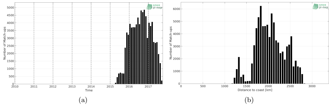
Figure 1: Number of match-ups between Surface drifters and SMOS-L3-CATDS-CECOS-LOCEAN-V3-9DAYS-25KM SSS as a function of time (a) and as function of the distance to coast (b) over the OTT zone Pi-MEP region and for the full satellite product period.
