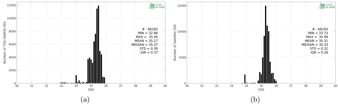
Figure 2: Histograms of SSS from TSG-SAMOS (a) and SMOS-L3-CATDS-CECOS-LOCEAN-V3-18DAYS-25KM (b) considering all match-up pairs per bins of 0.1 over the OTT zone Pi-MEP region and for the full satellite product period.
