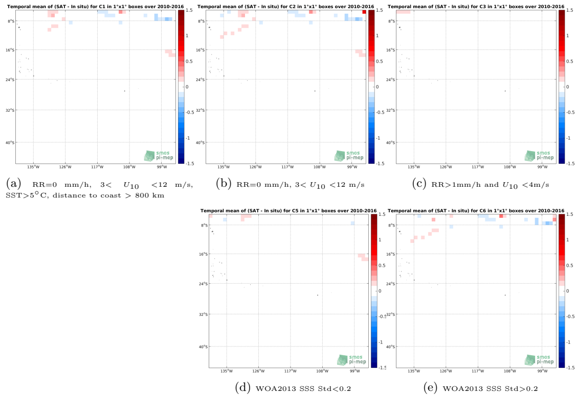
Figure 12: Temporal mean gridded over spatial boxes of size 1^\circ \times 1^\circ of \Delta SSS (SMOS-L3-CATDS-CECOS-LOCEAN-V3-18DAYS-25KM - TSG-SAMOS) for 5 different subdatasets corresponding to: RR=0 mm/h, 3 < U_{10} < 12 m/s, SST > 5^\circ\text{C} , distance to coast > 800 km (a), RR=0 mm/h, 3 < U_{10} < 12 m/s (b), RR > 1 mm/h and U_{10} < 4 m/s (c), WOA2013 SSS Std < 0.2 (d), WOA2013 SSS Std > 0.2 (e).
