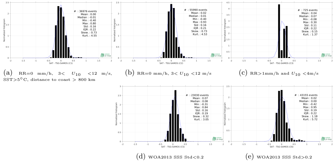
Figure 13: Normalized histogram of \Delta SSS (SMOS-L3-CATDS-CECOS-LOCEAN-V3-18DAYS-25KM - TSG-SAMOS) for 5 different subdatasets corresponding to: RR=0 mm/h, 3 < U_{10} < 12 m/s, SST>5°C, distance to coast > 800 km (a), RR=0 mm/h, 3 < U_{10} < 12 m/s (b), RR>1mm/h and U_{10} < 4 m/s (c), WOA2013 SSS Std<0.2 (d), WOA2013 SSS Std>0.2 (e).
