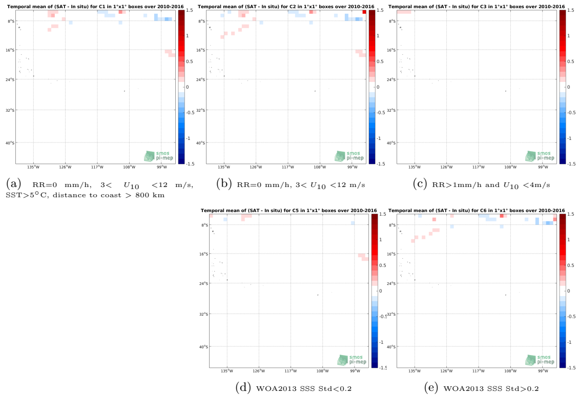
Figure 12: Temporal mean gridded over spatial boxes of size 1^\circ \times 1^\circ of \Delta SSS (SMOS-L3-CATDS-CECOS-LOCEAN-V3-18DAYS-25KM - TSG-SAMOS) for 5 different subdatasets corresponding to:RR=0 mm/h, 3 < U_{10} < 12 m/s, SST >5^\circ C, distance to coast > 800 km (a), RR=0 mm/h, 3 < U_{10} < 12 m/s (b), RR >1 mm/h and U_{10} < 4 m/s (c), WOA2013 SSS Std <0.2 (d), WOA2013 SSS Std >0.2 (e).
