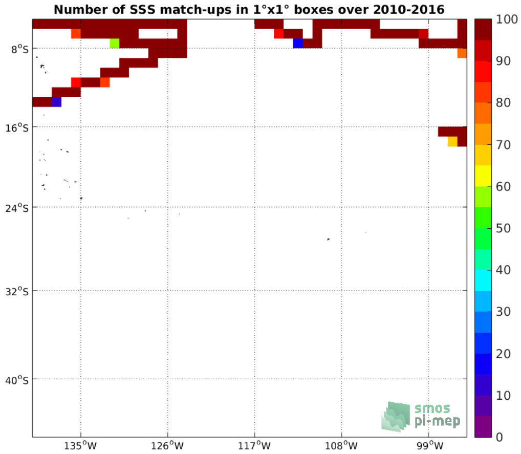
Figure 4: Number of SSS match-ups between TSG-SAMOS SSS and the SMOS-L3-CATDS-CECOS-LOCEAN-V3-18DAYS-25KM SSS product for the OTT zone Pi-MEP region over 1°x1° boxes and for the full satellite product period.
