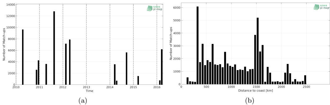
Figure 1: Number of match-ups between TSG-SAMOS and SMOS-L3-CATDS-CECOS-LOCEAN-V3-18DAYS-25KM SSS as a function of time (a) and as function of the distance to coast (b) over the OTT zone Pi-MEP region and for the full satellite product period.
