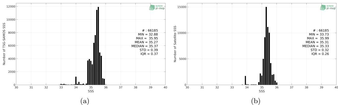
Figure 2: Histograms of SSS from TSG-SAMOS (a) and SMOS-L3-CATDS-CECOS-LOCEAN-V3-18DAYS-25KM (b) considering all match-up pairs per bins of 0.1 over the OTT zone Pi-MEP region and for the full satellite product period.
