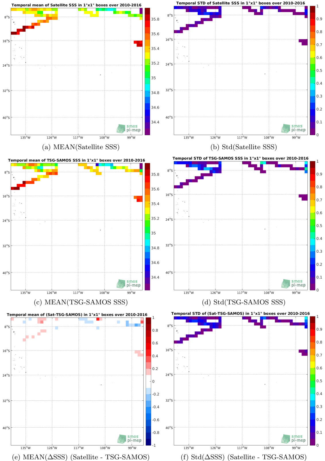
Figure 6: Temporal mean (left) and Std (right) of SSS from SMOS-L3-CATDS-CECOS-LOCEAN-V3-18DAYS-25KM (top), TSG-SAMOS (middle), and of \Delta SSS (Satellite - TSG-SAMOS). Only match-up pairs are used to generate these maps.
