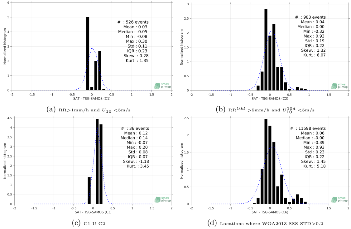
Figure 13: Normalized histogram of \Delta\text{SSS} (SMOS-L3-CATDS-CECOS-LOCEAN-V3-18DAYS-25KM - TSG-SAMOS) for 6 different subdatasets corresponding to: RR > 1mm/h and U_{10} < 5\text{m/s} (a), RR^{10d} > 5\text{mm/h} and U_{10}^{10d} < 5\text{m/s} (b), C1 U C2 (c), Locations where WOA2013 SSS STD > 0.2 (d).
