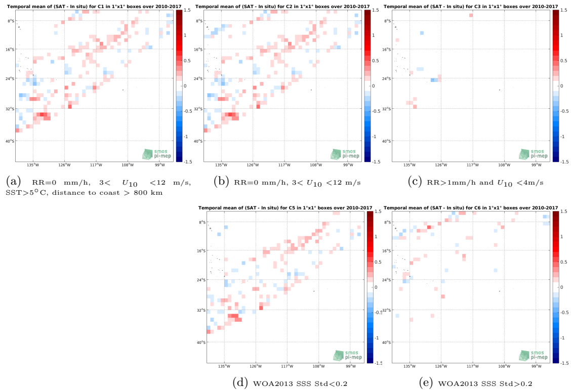
Figure 12: Temporal mean gridded over spatial boxes of size 1^\circ \times 1^\circ of \Delta SSS (SMOS-L3-CATDS-CECOS-LOCEAN-V3-18DAYS-25KM - TSG-LEGOS-DM) for 5 different subdatasets corresponding to:RR=0 mm/h, 3 < U_{10} < 12 m/s, SST >5^\circ C, distance to coast > 800 km (a), RR=0 mm/h, 3 < U_{10} < 12 m/s (b), RR >1 mm/h and U_{10} < 4 m/s (c), WOA2013 SSS Std <0.2 (d), WOA2013 SSS Std >0.2 (e).
