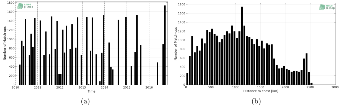
Figure 1: Number of match-ups between TSG-LEGOS-DM and SMOS-L3-CATDS-CECOS-LOCEAN-V3-18DAYS-25KM SSS as a function of time (a) and as function of the distance to coast (b) over the OTT zone Pi-MEP region and for the full satellite product period.
