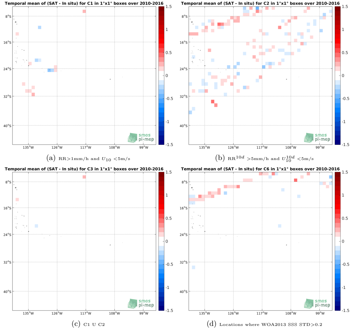
Figure 12: Temporal mean gridded over spatial boxes of size 1^\circ \times 1^\circ of \Delta SSS (SMOS-L3-CATDS-CECOS-LOCEAN-V3-18DAYS-25KM - TSG-LEGOS-DM) for 4 different subdatasets corresponding to:RR >1\text{mm/h} and U_{10} < 5\text{m/s} (a), RR^{10d} > 5\text{mm/h} and U_{10}^{10d} < 5\text{m/s} (b), C1 U C2 (c),Locations where WOA2013 SSS STD >0.2 (d).
