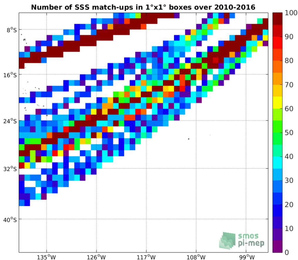
Figure 4: Number of SSS match-ups between TSG-LEGOS-DM SSS and the SMOS-L3-CATDS-CECOS-LOCEAN-V3-18DAYS-25KM SSS product for the OTT zone Pi-MEP region over 1°x1° boxes and for the full satellite product period.
