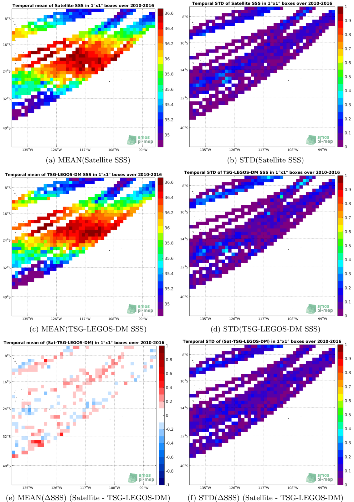
Figure 6: Temporal mean (left) and STD (right) of SSS from SMOS-L3-CATDS-CECOS-LOCEAN-V3-18DAYS-25KM (top), TSG-LEGOS-DM (middle), and of \Delta SSS (Satellite - TSG-LEGOS-DM). Only match-up pairs are used to generate these maps.
