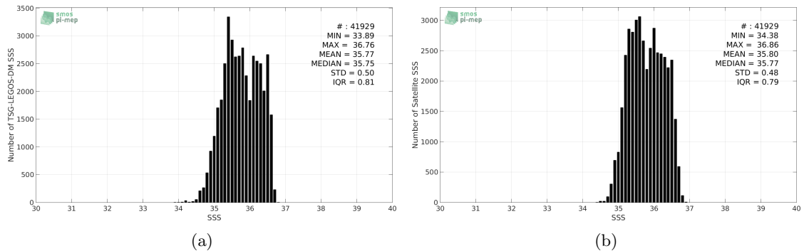
Figure 2: Histograms of SSS from TSG-LEGOS-DM (a) and SMOS-L3-CATDS-CECOS-LOCEAN-V3-18DAYS-25KM (b) considering all match-up pairs per bins of 0.1 over the OTT zone Pi-MEP region and for the full satellite product period.
