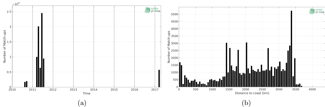
Figure 1: Number of match-ups between TSG-GOSUD-Sailing-ship and SMOS-L3-CATDS-CECOS-LOCEAN-V3-18DAYS-25KM SSS as a function of time (a) and as function of the distance to coast (b) over the OTT zone Pi-MEP region and for the full satellite product period.
