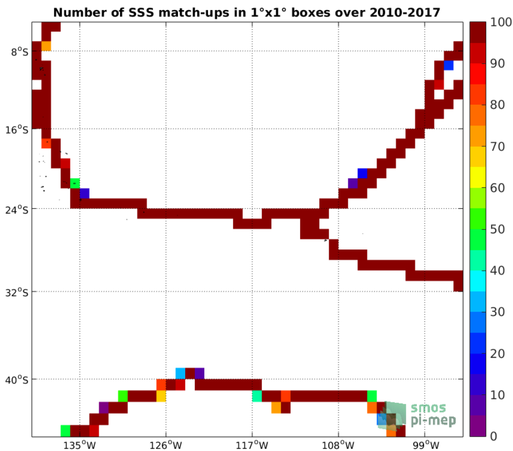
Figure 4: Number of SSS match-ups between TSG-GOSUD-Sailing-ship SSS and the SMOS-L3-CATDS-CECOS-LOCEAN-V3-18DAYS-25KM SSS product for the OTT zone Pi-MEP region over 1°x1° boxes and for the full satellite product period.
