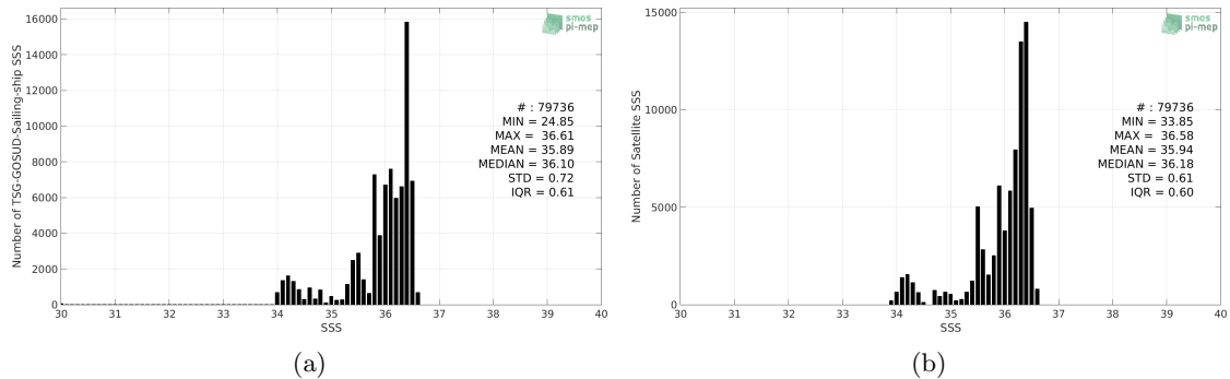
Figure 2: Histograms of SSS from TSG-GOSUD-Sailing-ship (a) and SMOS-L3-CATDS-CECOS-LOCEAN-V3-18DAYS-25KM (b) considering all match-up pairs per bins of 0.1 over the OTT zone Pi-MEP region and for the full satellite product period.
