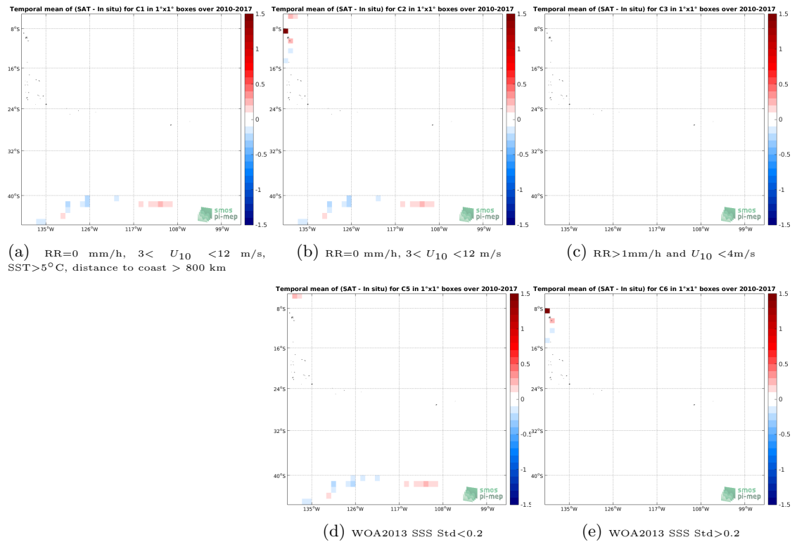
Figure 12: Temporal mean gridded over spatial boxes of size 1^\circ \times 1^\circ of \Delta SSS (SMOS-L3-CATDS-CECOS-LOCEAN-V3-18DAYS-25KM - TSG-GOSUD-Sailing-ship) for 5 different subdatasets corresponding to:RR=0 mm/h, 3 < U_{10} < 12 m/s, SST >5^\circ\text{C} , distance to coast > 800 km (a), RR=0 mm/h, 3 < U_{10} < 12 m/s (b), RR >1 mm/h and U_{10} < 4 m/s (c), WOA2013 SSS Std <0.2 (d), WOA2013 SSS Std >0.2 (e).
