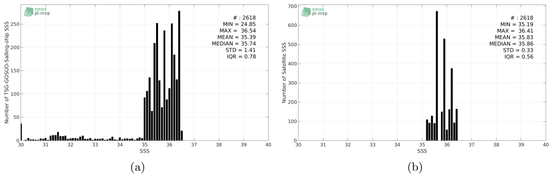
Figure 2: Histograms of SSS from TSG-GOSUD-Sailing-ship (a) and SMOS-L3-CATDS-CECOS-LOCEAN-V3-18DAYS-25KM (b) considering all match-up pairs per bins of 0.1 over the OTT zone Pi-MEP region and for the full satellite product period.
