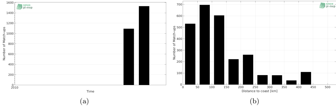
Figure 1: Number of match-ups between TSG-GOSUD-Sailing-ship and SMOS-L3-CATDS-CECOS-LOCEAN-V3-18DAYS-25KM SSS as a function of time (a) and as function of the distance to coast (b) over the OTT zone Pi-MEP region and for the full satellite product period.
