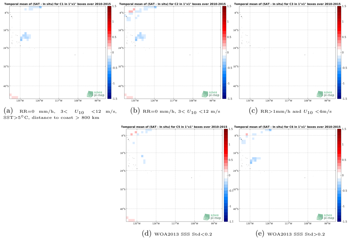
Figure 12: Temporal mean gridded over spatial boxes of size 1^\circ \times 1^\circ of \Delta SSS (SMOS-L3-CATDS-CECOS-LOCEAN-V3-18DAYS-25KM - TSG-GOSUD-Research-vessel) for 5 different subdatasets corresponding to:RR=0 mm/h, 3 < U_{10} < 12 m/s, SST >5^\circ C, distance to coast > 800 km (a), RR=0 mm/h, 3 < U_{10} < 12 m/s (b), RR >1 mm/h and U_{10} < 4 m/s (c), WOA2013 SSS Std <0.2 (d), WOA2013 SSS Std >0.2 (e).
