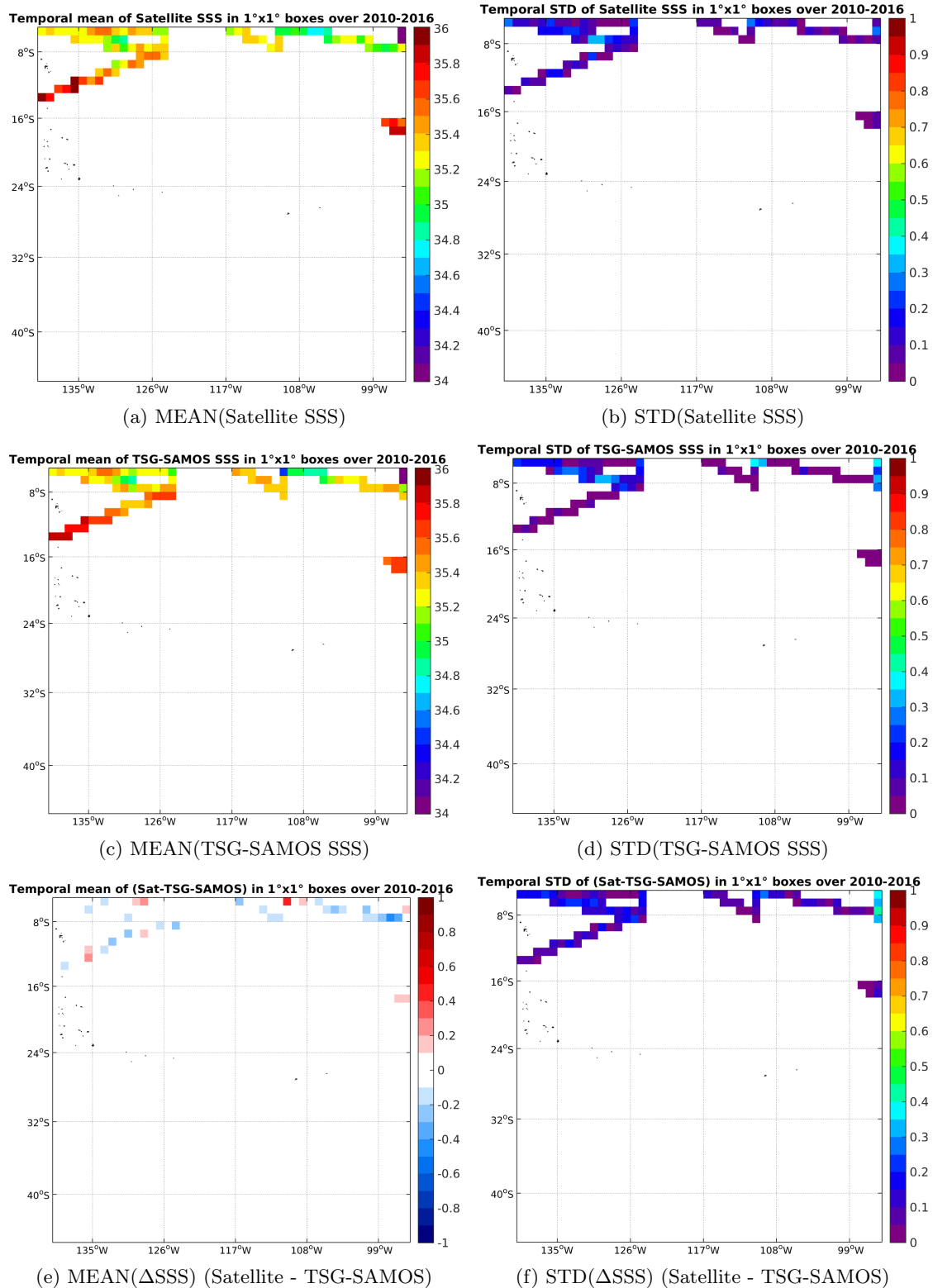
Figure 6: Temporal mean (left) and STD (right) of SSS from SMOS-L3-CATDS-CECOS-LOCEAN-V2-9DAYS-25KM (top), TSG-SAMOS (middle), and of \Delta SSS (Satellite - TSG-SAMOS). Only match-up pairs are used to generate these maps.
