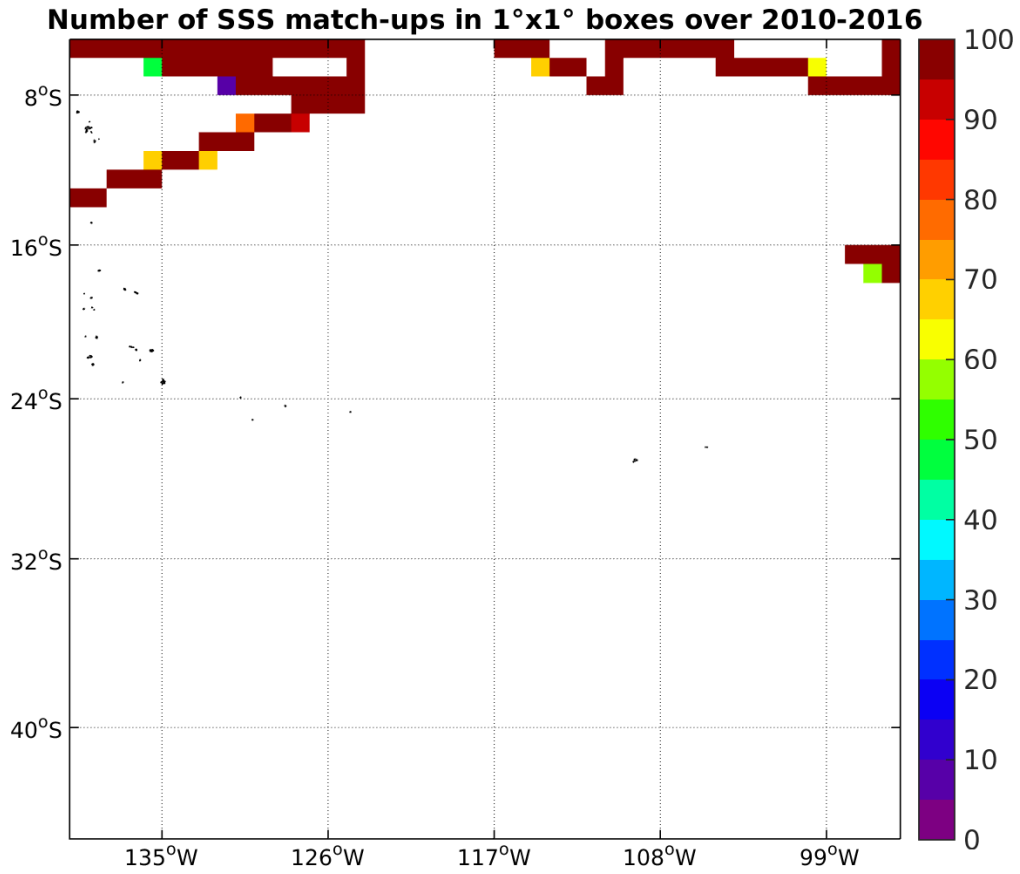
Figure 4: Number of SSS match-ups between TSG-SAMOS SSS and the SMOS-L3-CATDS-CECOS-LOCEAN-V2-9DAYS-25KM SSS product for the OTT zone Pi-MEP region over 1°x1° boxes and for the full satellite product period.
