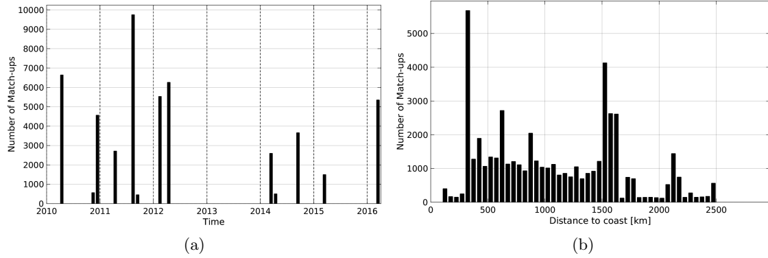
Figure 1: Number of match-ups between TSG-SAMOS and SMOS-L3-CATDS-CECOS-LOCEAN-V2-9DAYS-25KM SSS as a function of time (a) and as function of the distance to coast (b) over the OTT zone Pi-MEP region and for the full satellite product period.
