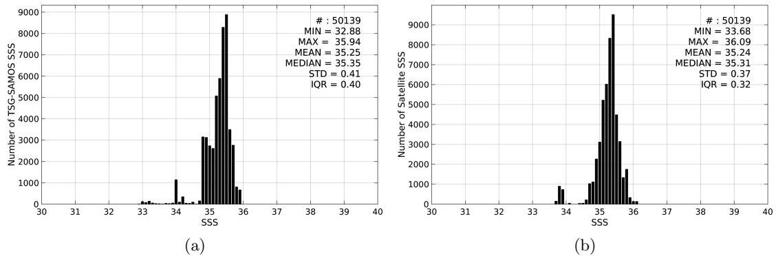
Figure 2: Histograms of SSS from TSG-SAMOS (a) and SMOS-L3-CATDS-CECOS-LOCEAN-V2-9DAYS-25KM (b) considering all match-up pairs per bins of 0.1 over the OTT zone Pi-MEP region and for the full satellite product period.
