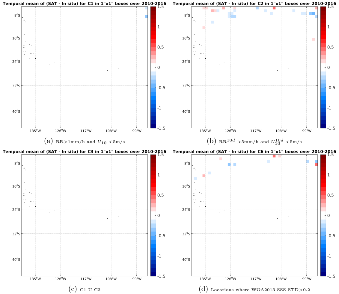
Figure 12: Temporal mean gridded over spatial boxes of size 1°x1° of \Delta SSS (SMOS-L3-CATDS-CECOS-LOCEAN-V2-9DAYS-25KM - TSG-SAMOS) for 4 different subdatasets corresponding to: RR > 1\text{mm/h} and U_{10} < 5\text{m/s} (a), RR^{10d} > 5\text{mm/h} and U_{10}^{10d} < 5\text{m/s} (b), C1 U C2 (c), Locations where WOA2013 SSS STD > 0.2 (d).
