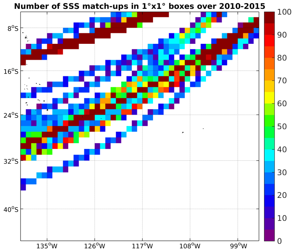
Figure 4: Number of SSS match-ups between TSG-LEGOS-DM SSS and the SMOS-L3-CATDS-CECOS-LOCEAN-V2-9DAYS-25KM SSS product for the OTT zone Pi-MEP region over 1°x1° boxes and for the full satellite product period.
