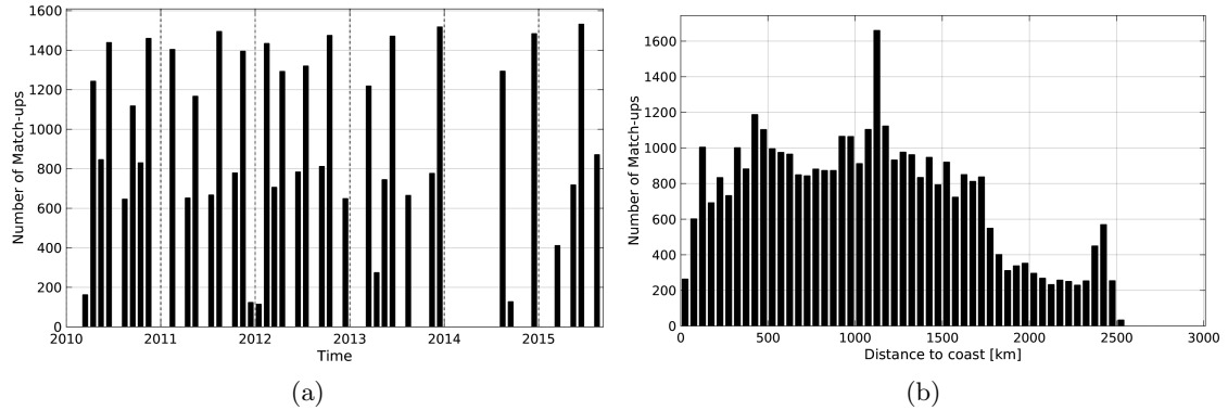
Figure 1: Number of match-ups between TSG-LEGOS-DM and SMOS-L3-CATDS-CECOS-LOCEAN-V2-9DAYS-25KM SSS as a function of time (a) and as function of the distance to coast (b) over the OTT zone Pi-MEP region and for the full satellite product period.
