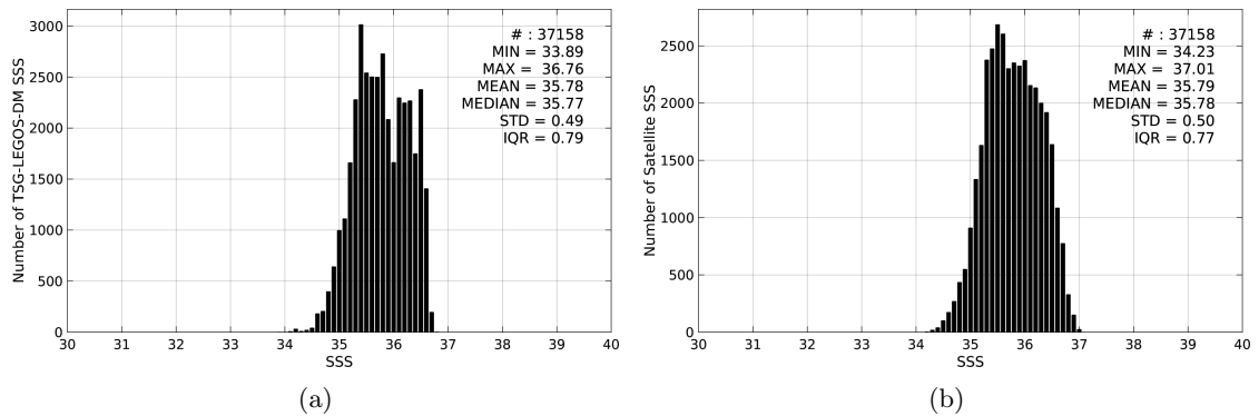
Figure 2: Histograms of SSS from TSG-LEGOS-DM (a) and SMOS-L3-CATDS-CECOS-LOCEAN-V2-9DAYS-25KM (b) considering all match-up pairs per bins of 0.1 over the OTT zone Pi-MEP region and for the full satellite product period.
