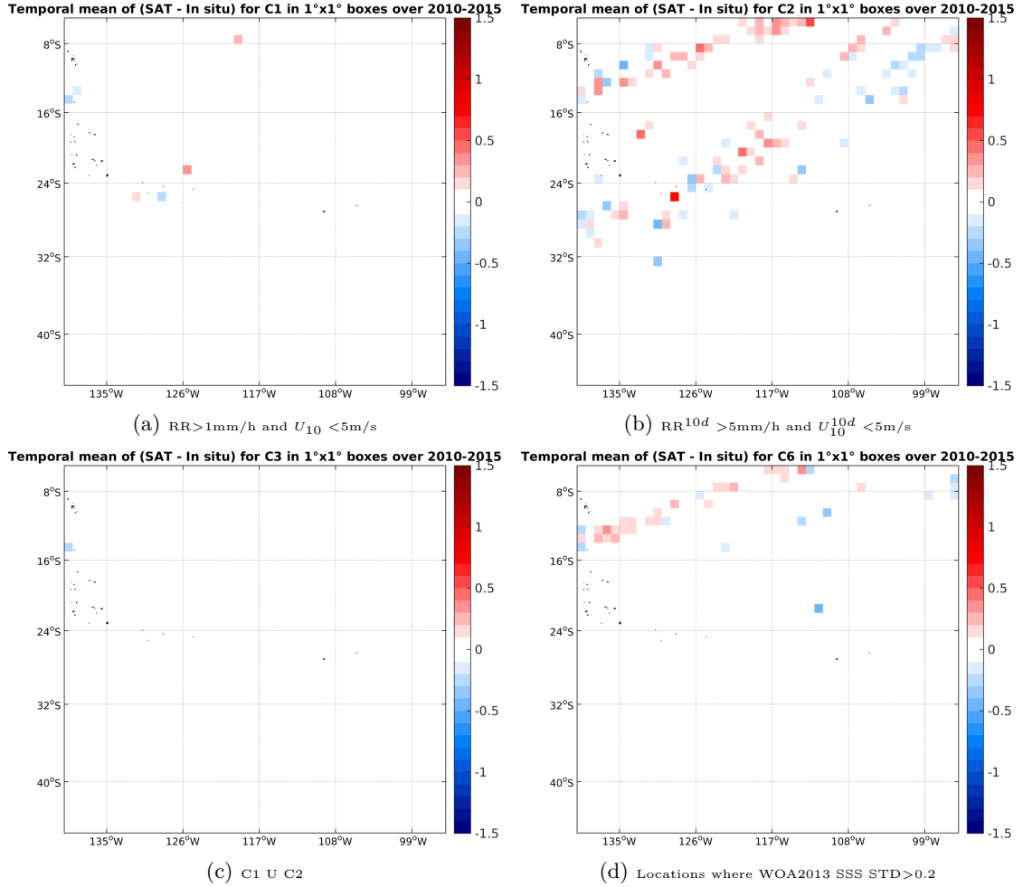
Figure 12: Temporal mean gridded over spatial boxes of size 1°x1° of \Delta SSS (SMOS-L3-CATDS-CECOS-LOCEAN-V2-9DAYS-25KM - TSG-LEGOS-DM) for 4 different subdatasets corresponding to:RR>1mm/h and U_{10} < 5 m/s (a), RR^{10d} > 5 mm/h and U_{10}^{10d} < 5 m/s (b), C1 U C2 (c),Locations where WOA2013 SSS STD>0.2 (d).
