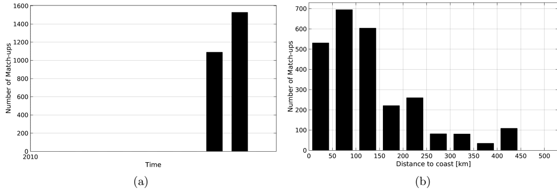
Figure 1: Number of match-ups between TSG-GOSUD-Sailing-ship and SMOS-L3-CATDS-CECOS-LOCEAN-V2-9DAYS-25KM SSS as a function of time (a) and as function of the distance to coast (b) over the OTT zone Pi-MEP region and for the full satellite product period.
