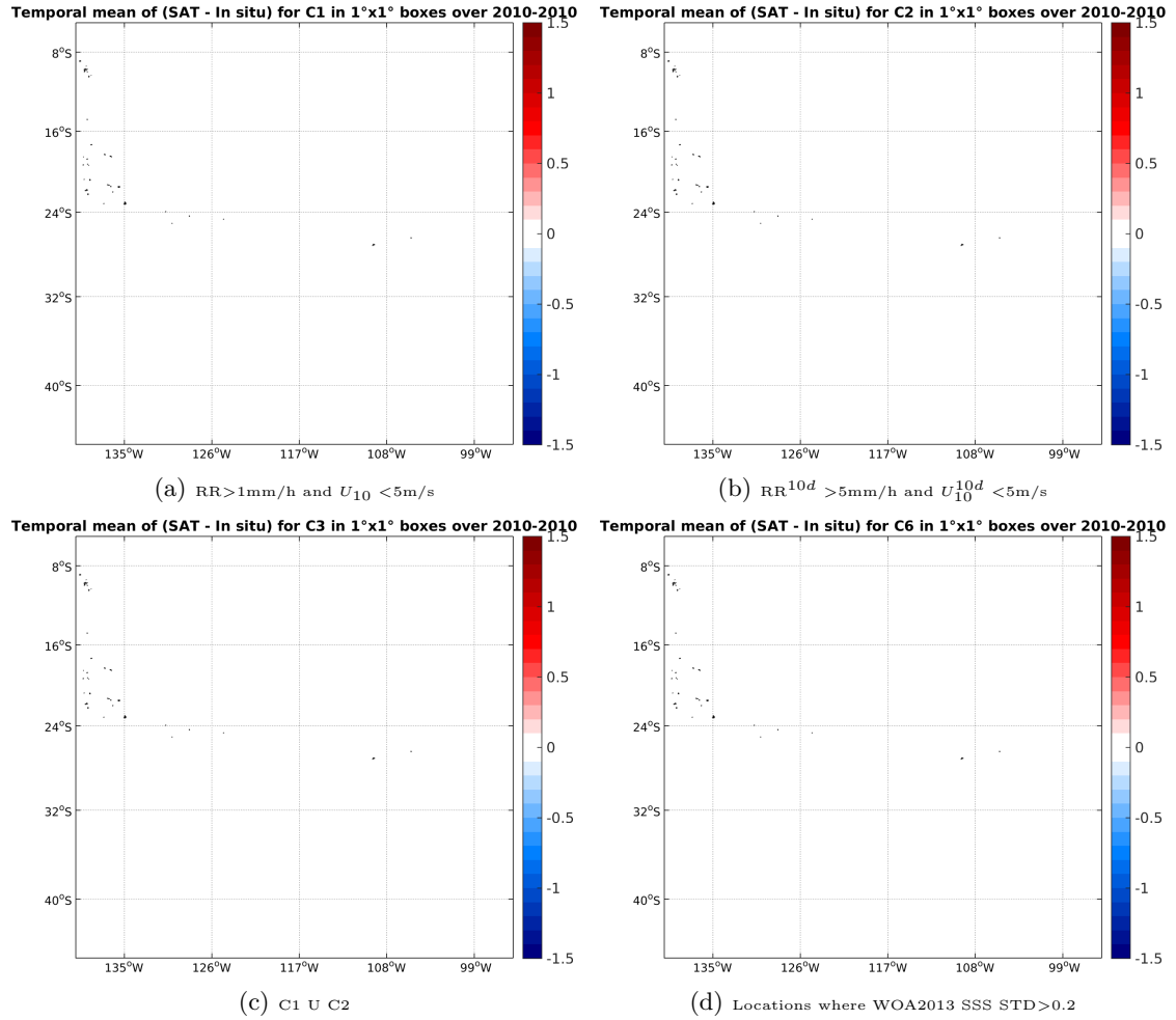
Figure 12: Temporal mean gridded over spatial boxes of size 1°x1° of \Delta SSS (SMOS-L3-CATDS-CECOS-LOCEAN-V2-9DAYS-25KM - TSG-GOSUD-Sailing-ship) for 4 different subdatasets corresponding to: RR > 1\text{mm/h} and U_{10} < 5\text{m/s} (a), RR^{10d} > 5\text{mm/h} and U_{10}^{10d} < 5\text{m/s} (b), C1 U C2 (c), Locations where WOA2013 SSS STD > 0.2 (d).
