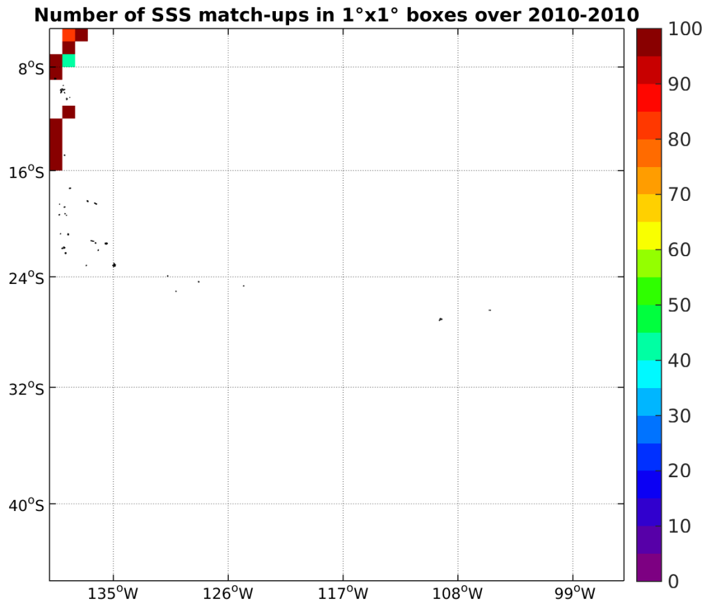
Figure 4: Number of SSS match-ups between TSG-GOSUD-Sailing-ship SSS and the SMOS-L3-CATDS-CECOS-LOCEAN-V2-9DAYS-25KM SSS product for the OTT zone Pi-MEP region over 1°x1° boxes and for the full satellite product period.
