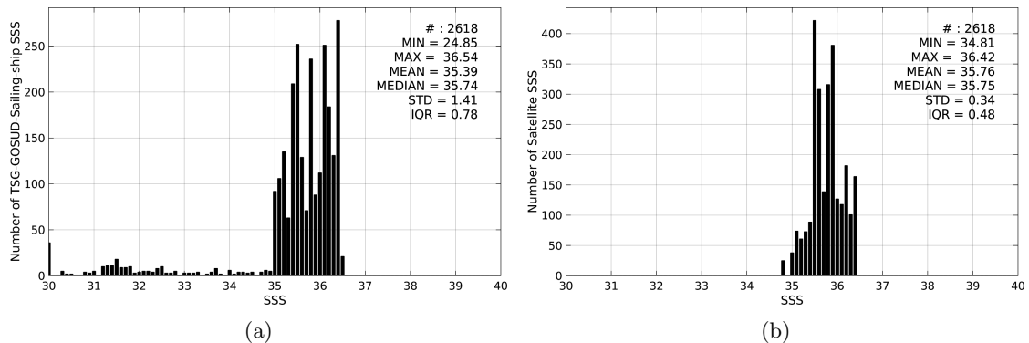
Figure 2: Histograms of SSS from TSG-GOSUD-Sailing-ship (a) and SMOS-L3-CATDS-CECOS-LOCEAN-V2-9DAYS-25KM (b) considering all match-up pairs per bins of 0.1 over the OTT zone Pi-MEP region and for the full satellite product period.
