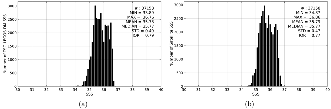
Figure 2: Histograms of SSS from TSG-LEGOS-DM (a) and SMOS-L3-CATDS-CECOS-LOCEAN-V2-18DAYS-25KM (b) considering all match-up pairs per bins of 0.1 over the OTT zone Pi-MEP region and for the full satellite product period.
