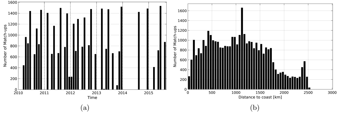
Figure 1: Number of match-ups between TSG-LEGOS-DM and SMOS-L3-CATDS-CECOS-LOCEAN-V2-18DAYS-25KM SSS as a function of time (a) and as function of the distance to coast (b) over the OTT zone Pi-MEP region and for the full satellite product period.
