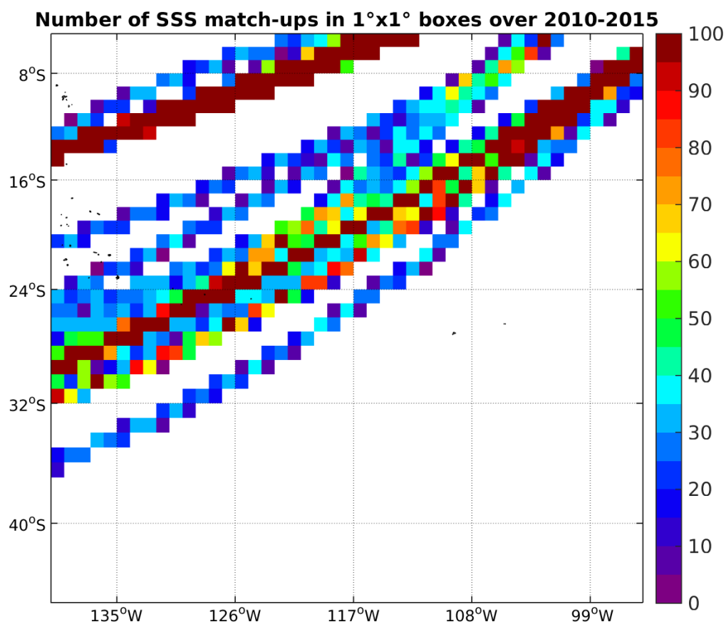
Figure 4: Number of SSS match-ups between TSG-LEGOS-DM SSS and the SMOS-L3-CATDS-CECOS-LOCEAN-V2-18DAYS-25KM SSS product for the OTT zone Pi-MEP region over 1°x1° boxes and for the full satellite product period.
