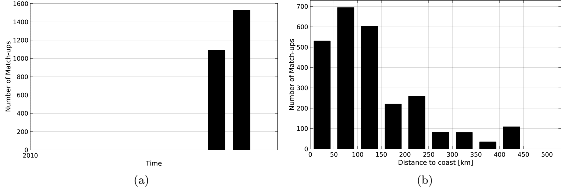
Figure 1: Number of match-ups between TSG-GOSUD-Sailing-ship and SMOS-L3-CATDS-CECOS-LOCEAN-V2-18DAYS-25KM SSS as a function of time (a) and as function of the distance to coast (b) over the OTT zone Pi-MEP region and for the full satellite product period.
