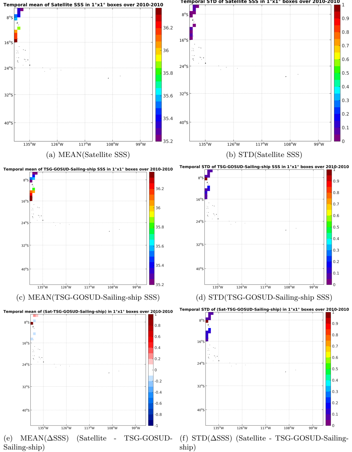
Figure 6: Temporal mean (left) and STD (right) of SSS from SMOS-L3-CATDS-CECOS-LOCEAN-V2-18DAYS-25KM (top), TSG-GOSUD-Sailing-ship (middle), and of \Delta SSS (Satellite - TSG-GOSUD-Sailing-ship). Only match-up pairs are used to generate these maps.
