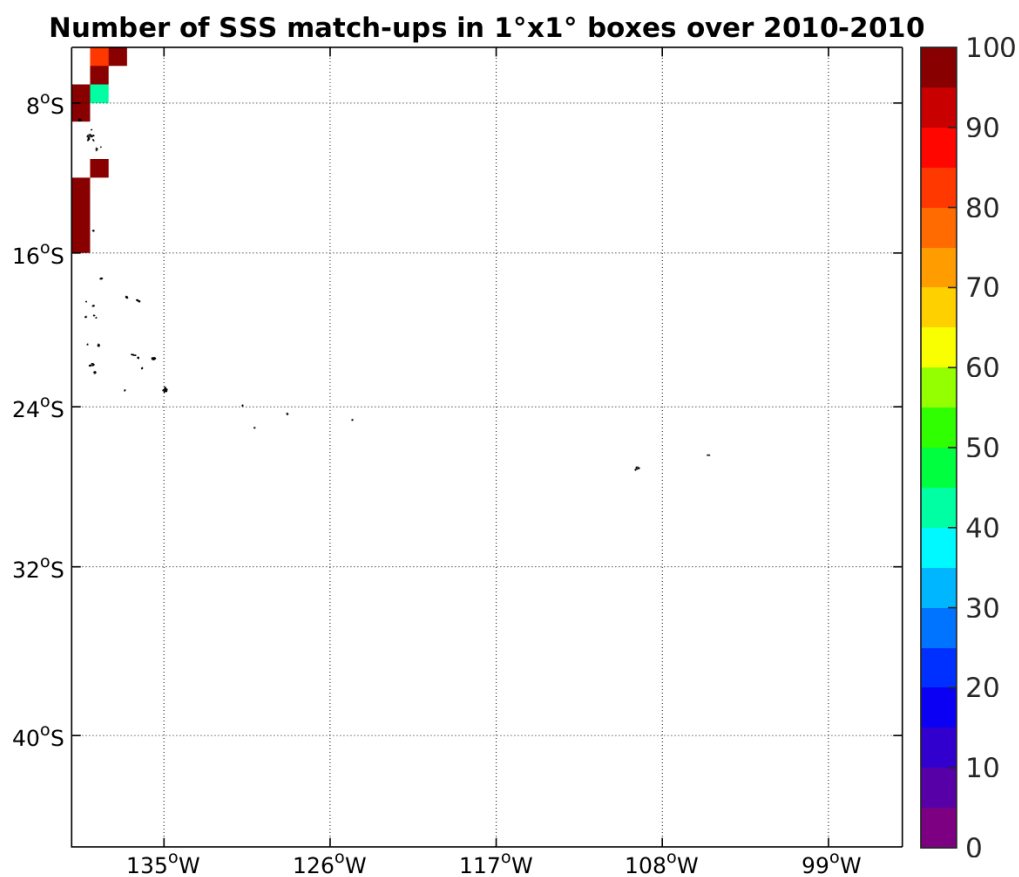
Figure 4: Number of SSS match-ups between TSG-GOSUD-Sailing-ship SSS and the SMOS-L3-CATDS-CECOS-LOCEAN-V2-18DAYS-25KM SSS product for the OTT zone Pi-MEP region over 1°x1° boxes and for the full satellite product period.
