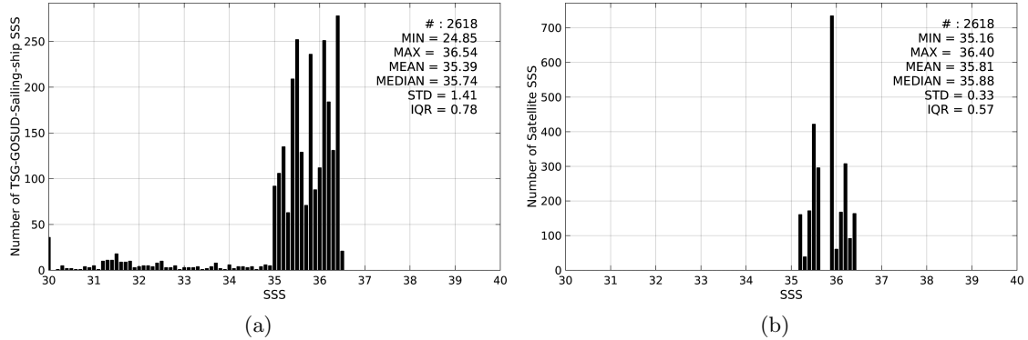
Figure 2: Histograms of SSS from TSG-GOSUD-Sailing-ship (a) and SMOS-L3-CATDS-CECOS-LOCEAN-V2-18DAYS-25KM (b) considering all match-up pairs per bins of 0.1 over the OTT zone Pi-MEP region and for the full satellite product period.
