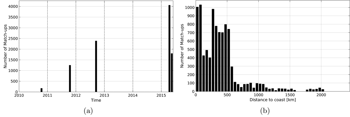
Figure 1: Number of match-ups between TSG-GOSUD-Research-vessel and SMOS-L3-CATDS-CECOS-LOCEAN-V2-18DAYS-25KM SSS as a function of time (a) and as function of the distance to coast (b) over the OTT zone Pi-MEP region and for the full satellite product period.
