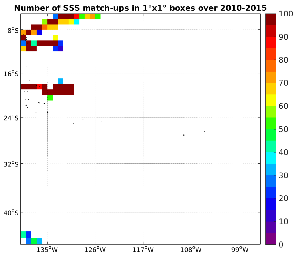
Figure 4: Number of SSS match-ups between TSG-GOSUD-Research-vessel SSS and the SMOS-L3-CATDS-CECOS-LOCEAN-V2-18DAYS-25KM SSS product for the OTT zone Pi-MEP region over 1°x1° boxes and for the full satellite product period.
