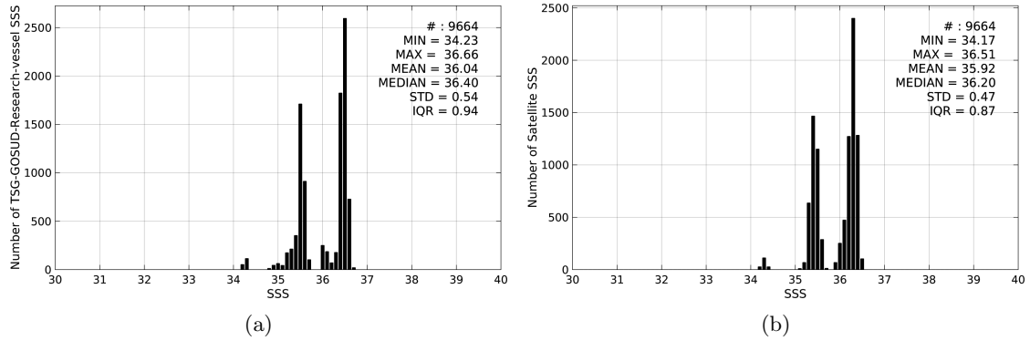
Figure 2: Histograms of SSS from TSG-GOSUD-Research-vessel (a) and SMOS-L3-CATDS-CECOS-LOCEAN-V2-18DAYS-25KM (b) considering all match-up pairs per bins of 0.1 over the OTT zone Pi-MEP region and for the full satellite product period.
