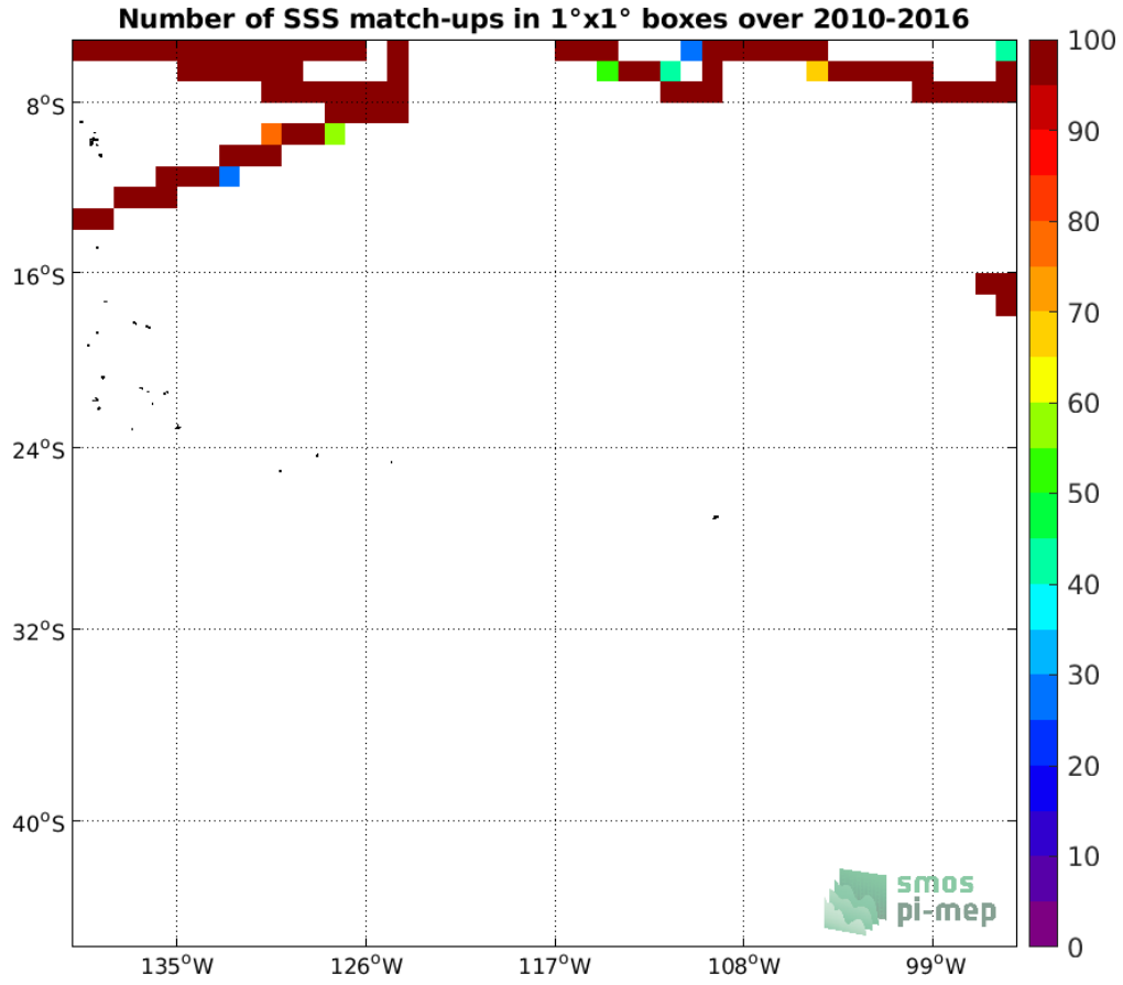
Figure 4: Number of SSS match-ups between TSG (SAMOS) SSS and the SMOS SSS L3 v2 - Monthly - 0.25 Deg (CATDS-CECOS-IFREMER) SSS product for the OTT zone Pi-MEP region over 1°x1° boxes and for the full satellite product period.
