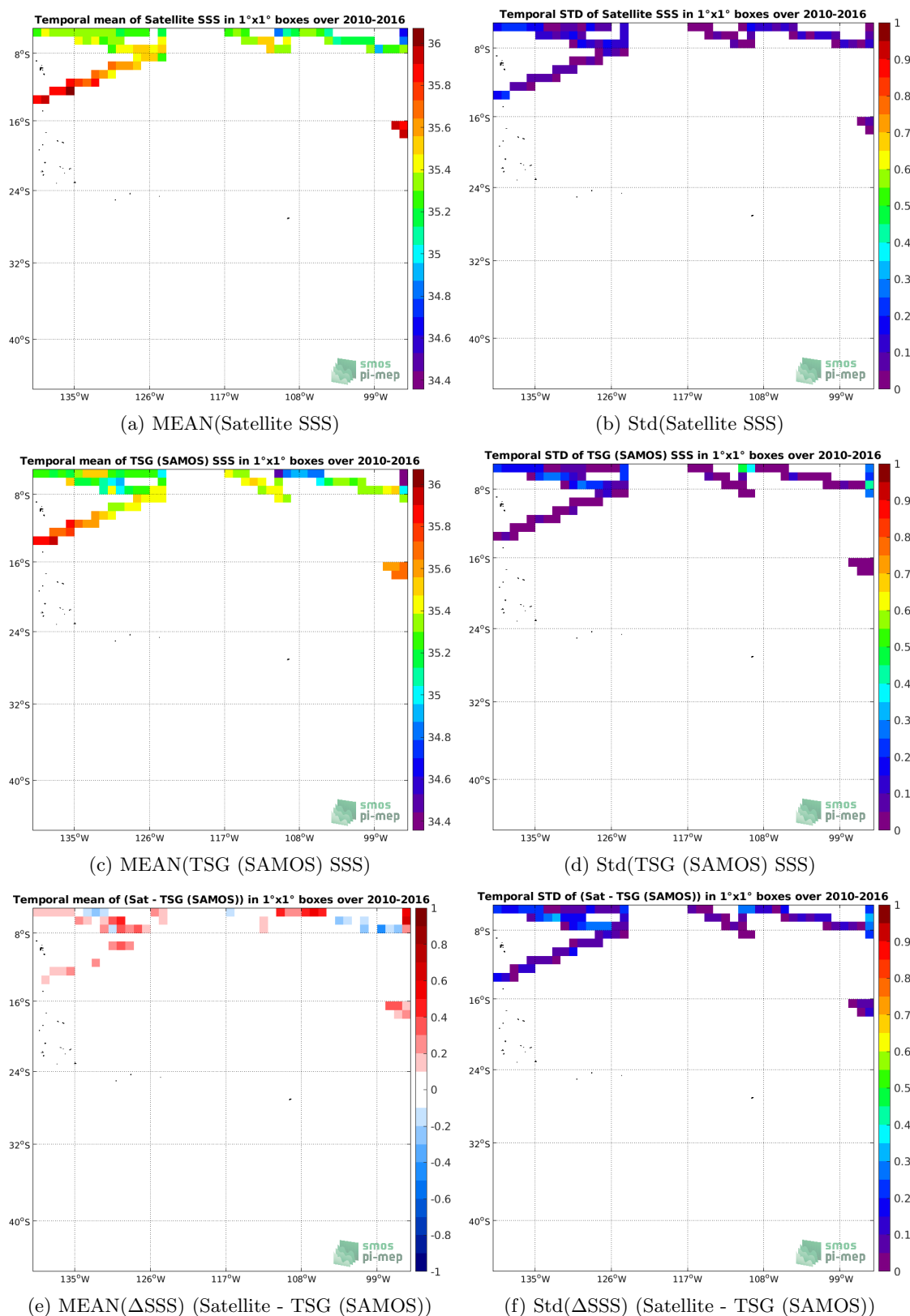
Figure 6: Temporal mean (left) and Std (right) of SSS from SMOS SSS L3 v2 - Monthly - 0.25 Deg (CATDS-CECOS-IFREMER) (top), TSG (SAMOS) (middle), and of \Delta SSS (Satellite - TSG (SAMOS)). Only match-up pairs are used to generate these maps.
