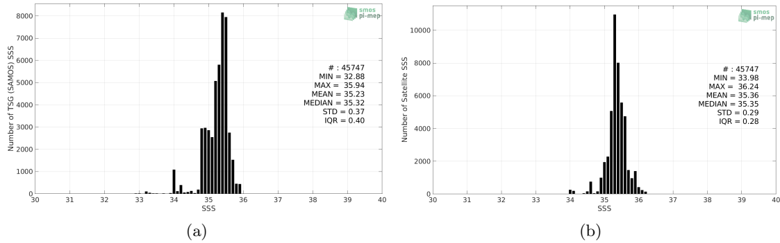
Figure 2: Histograms of SSS from TSG (SAMOS) (a) and SMOS SSS L3 v2 - Monthly - 0.25 Deg (CATDS-CECOS-IFREMER) (b) considering all match-up pairs per bins of 0.1 over the OTT zone Pi-MEP region and for the full satellite product period.
