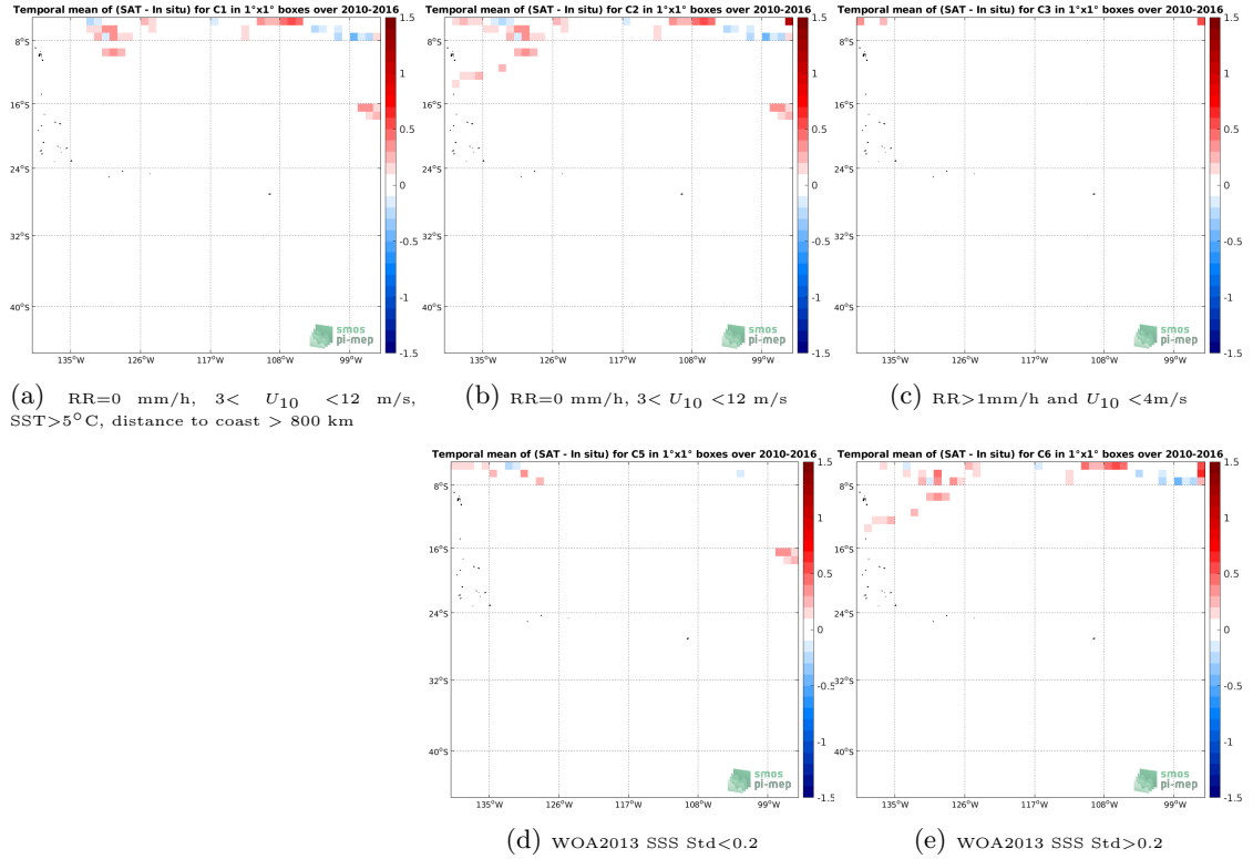
Figure 12: Temporal mean gridded over spatial boxes of size 1^{\circ}\times 1^{\circ} of \Delta\text{SSS} (SMOS SSS L3 v2 - Monthly - 0.25 Deg (CATDS-CECOS-IFREMER) - TSG (SAMOS)) for 5 different subdatasets corresponding to: \text{RR}=0 mm/h, 3 < U_{10} < 12 m/s, \text{SST}>5^{\circ}\text{C} , distance to coast > 800 km (a), \text{RR}=0 mm/h, 3 < U_{10} < 12 m/s (b), \text{RR}>1\text{mm/h} and U_{10} < 4\text{m/s} (c), \text{WOA2013 SSS Std}<0.2 (d), \text{WOA2013 SSS Std}>0.2 (e).
