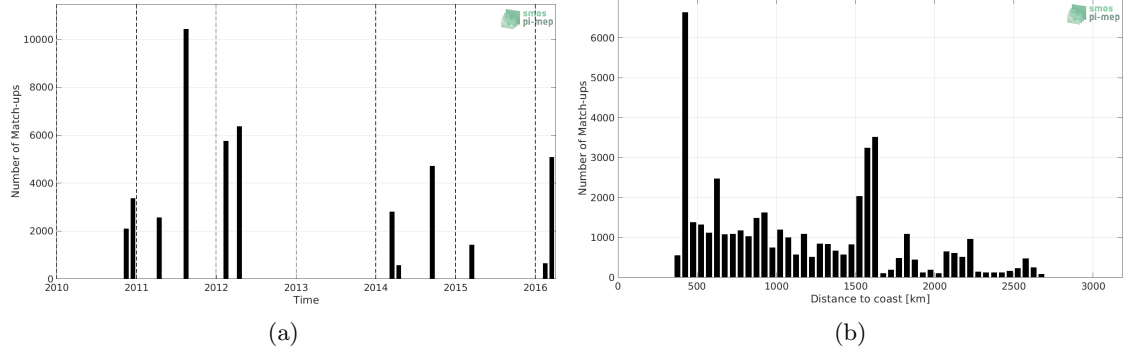
Figure 1: Number of match-ups between TSG (SAMOS) and SMOS SSS L3 v2 - Monthly - 0.25 Deg (CATDS-CECOS-IFREMER) SSS as a function of time (a) and as function of the distance to coast (b) over the OTT zone Pi-MEP region and for the full satellite product period.
