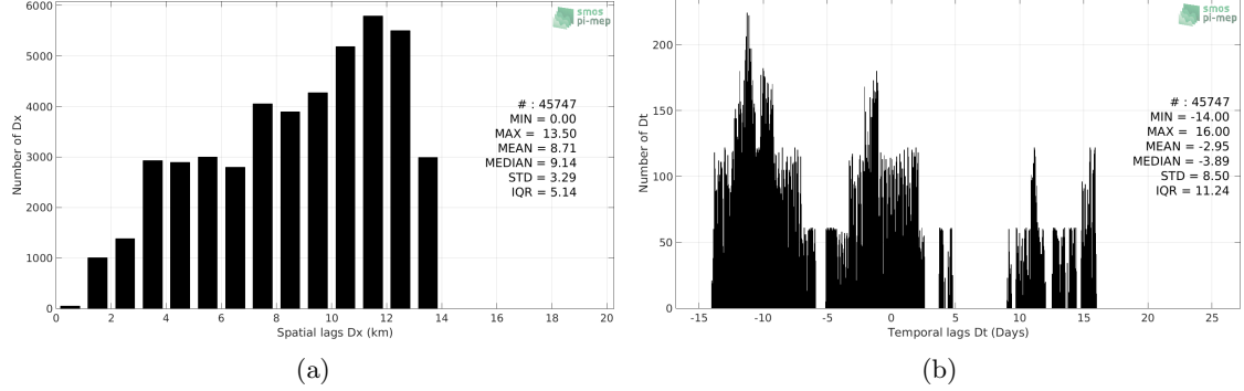
Figure 5: Histograms of the spatial (a) and temporal (b) lags between the time of the TSG (SAMOS) measurements and the date of the corresponding SMOS SSS L3 v2 - Monthly - 0.25 Deg (CATDS-CECOS-IFREMER) SSS product.
