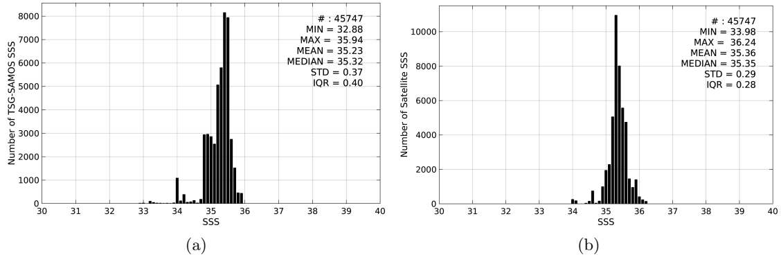
Figure 2: Histograms of SSS from TSG-SAMOS (a) and SMOS-L3-CATDS-IFREMER-CECOS-V2-MONTHLY-0.25DEG (b) considering all match-up pairs per bins of 0.1 over the OTT zone Pi-MEP region and for the full satellite product period.
