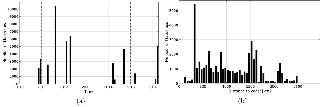
Figure 1: Number of match-ups between TSG-SAMOS and SMOS-L3-CATDS-IFREMER-CECOS-V2-MONTHLY-0.25DEG SSS as a function of time (a) and as function of the distance to coast (b) over the OTT zone Pi-MEP region and for the full satellite product period.
