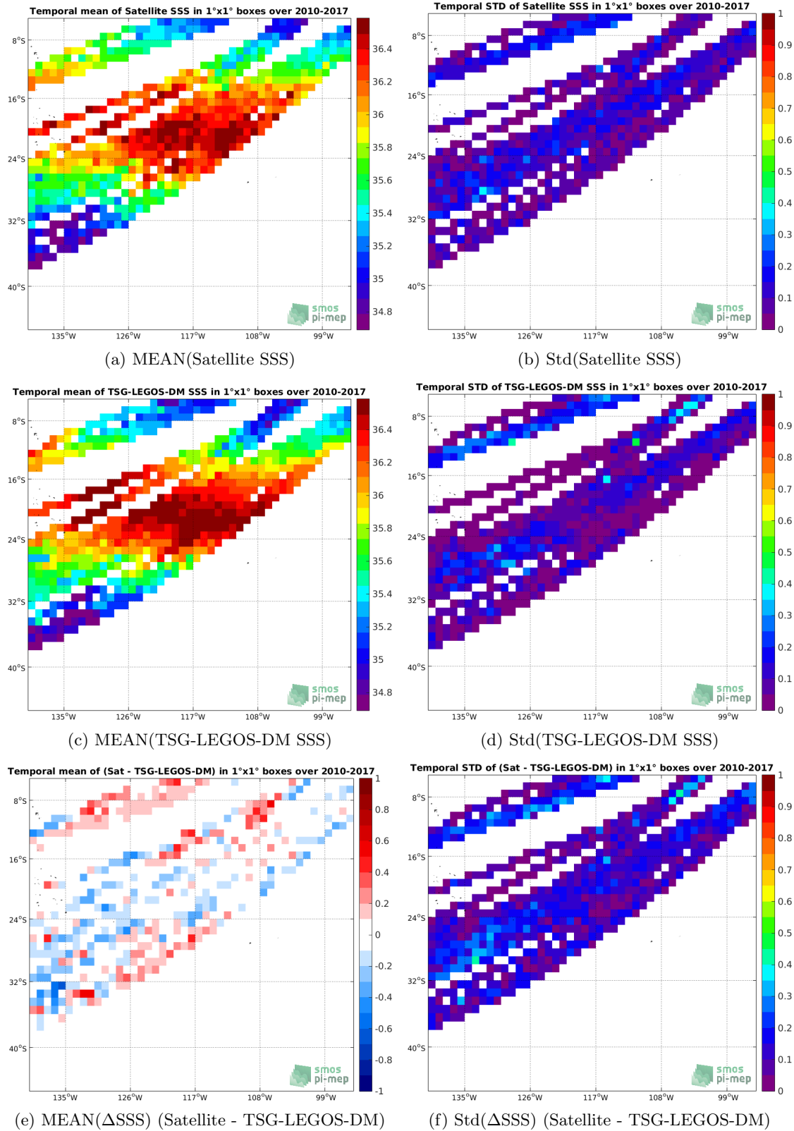
Figure 6: Temporal mean (left) and Std (right) of SSS from SMOS-L3-CATDS-IFREMER-CECOS-V2-MONTHLY-0.25DEG (top), TSG-LEGOS-DM (middle), and of \Delta SSS (Satellite - TSG-LEGOS-DM). Only match-up pairs are used to generate these maps.
