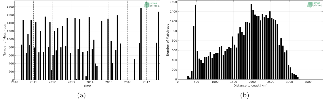
Figure 1: Number of match-ups between TSG-LEGOS-DM and SMOS-L3-CATDS-IFREMER-CECOS-V2-MONTHLY-0.25DEG SSS as a function of time (a) and as function of the distance to coast (b) over the OTT zone Pi-MEP region and for the full satellite product period.
