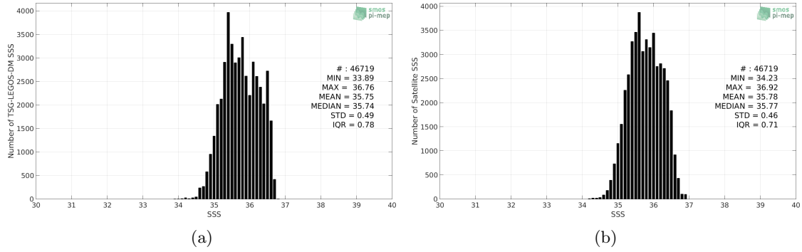
Figure 2: Histograms of SSS from TSG-LEGOS-DM (a) and SMOS-L3-CATDS-IFREMER-CECOS-V2-MONTHLY-0.25DEG (b) considering all match-up pairs per bins of 0.1 over the OTT zone Pi-MEP region and for the full satellite product period.
