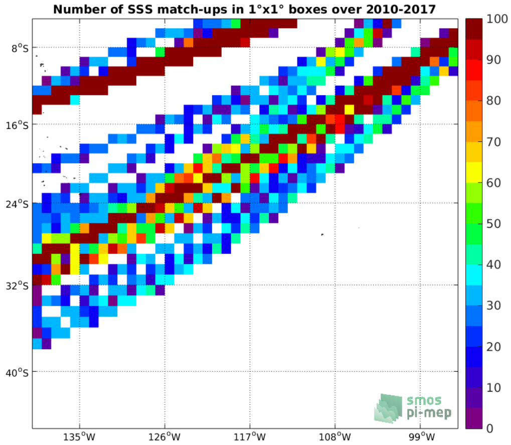
Figure 4: Number of SSS match-ups between TSG-LEGOS-DM SSS and the SMOS-L3-CATDS-IFREMER-CECOS-V2-MONTHLY-0.25DEG SSS product for the OTT zone Pi-MEP region over 1°x1° boxes and for the full satellite product period.
