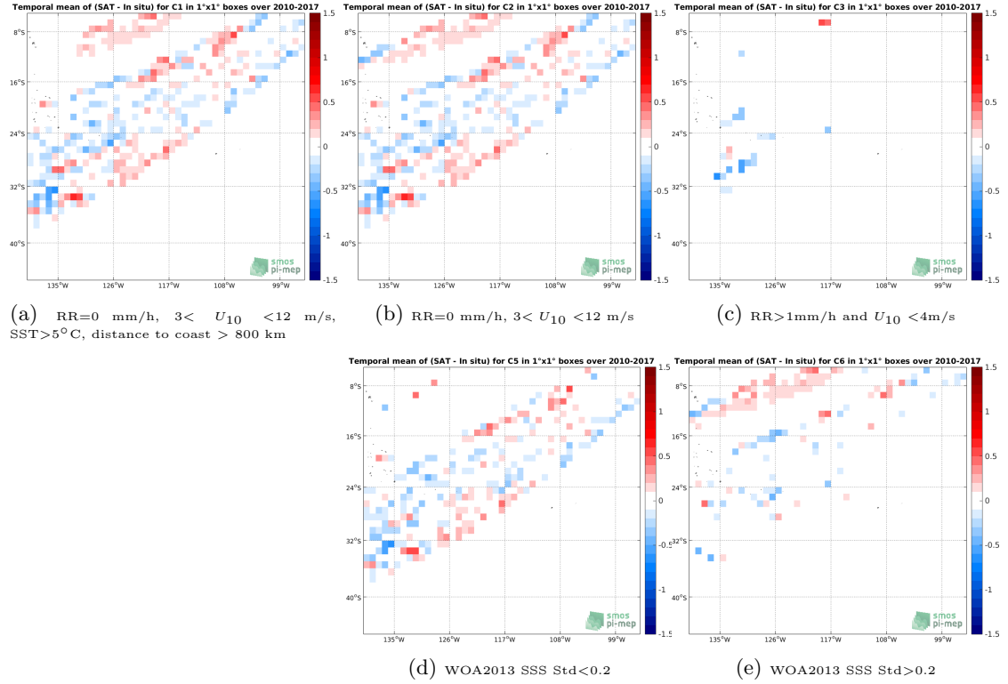
Figure 12: Temporal mean gridded over spatial boxes of size 1^\circ \times 1^\circ of \Delta SSS (SMOS-L3-CATDS-IFREMER-CECOS-V2-MONTHLY-0.25DEG - TSG-LEGOS-DM) for 5 different subdatasets corresponding to: RR=0 mm/h, 3 < U_{10} < 12 m/s, SST >5^\circ C, distance to coast > 800 km (a), RR=0 mm/h, 3 < U_{10} < 12 m/s (b), RR >1 mm/h and U_{10} < 4 m/s (c), WOA2013 SSS Std <0.2 (d), WOA2013 SSS Std >0.2 (e).
